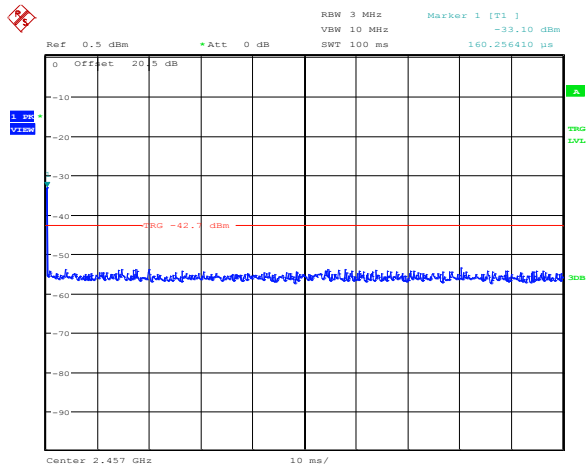
Figure 8.3-1: 100 ms transmission time frame for OB protocol
