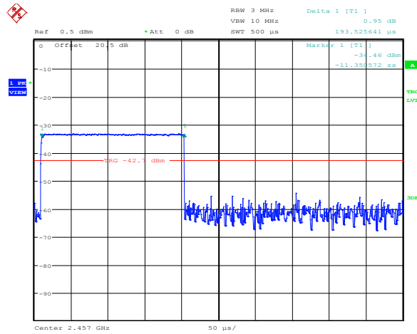
Figure 8.3-2: Pulse width for OB protocol
