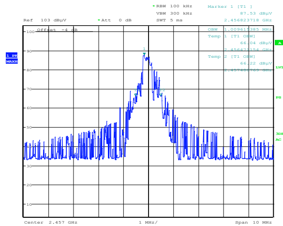
Figure 8.2-2: 99% dB bandwidth for OB protocol, sample plot
