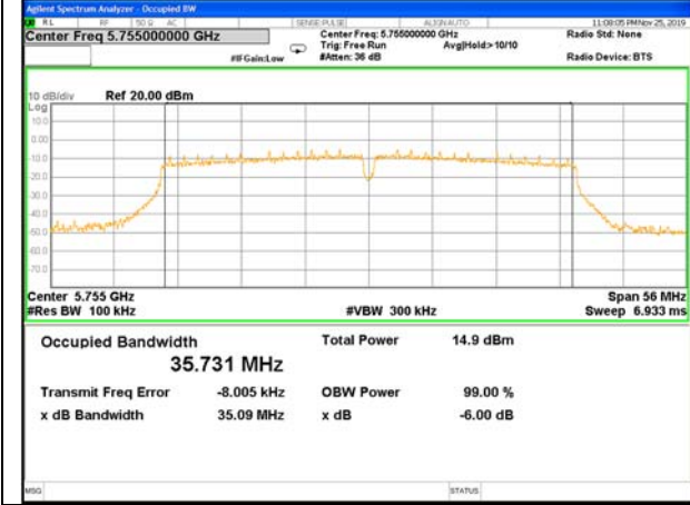
W58_11n40_Lower_6BW
