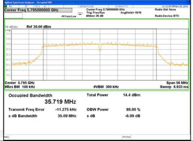
W58_11n40_Higher_6BW
