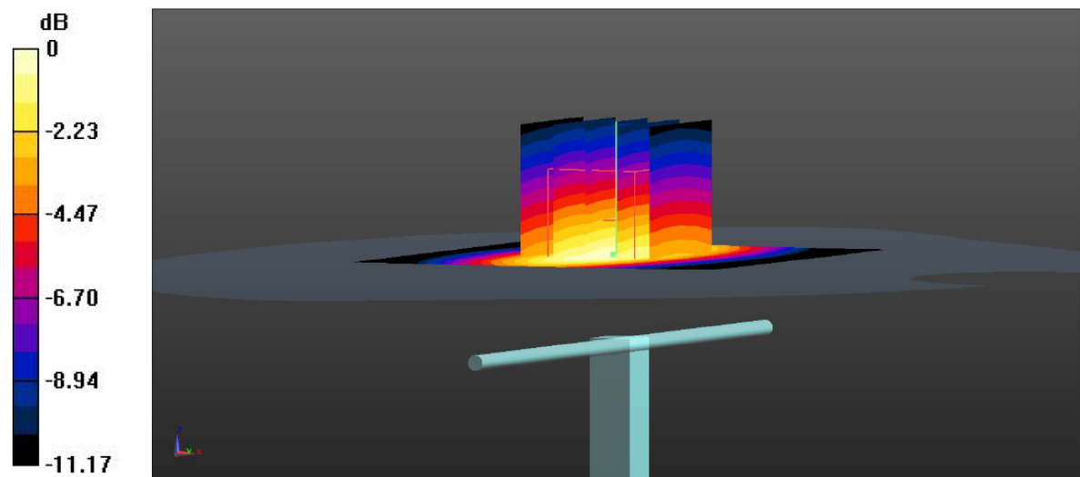
0 dB = 3.08 W/kg = 4.89 dBW/kg
