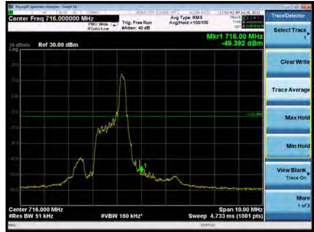
LTE eMTC Band 12 QPSK 10MHz CH-High, 100%RB
