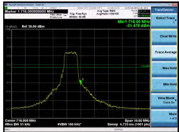
LTE eMTC Band 12 16QAM 10MHz CH-High, 1 RB
