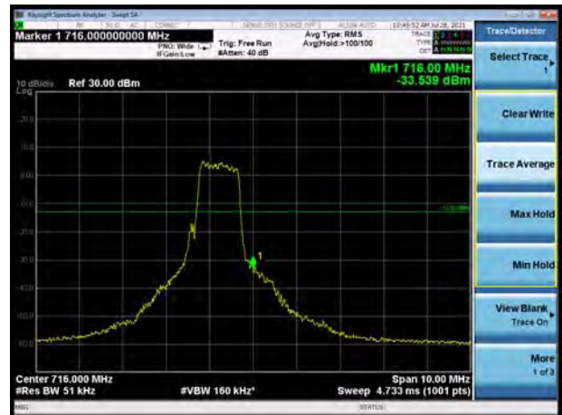
LTE eMTC Band 12 16QAM 3MHz CH-High, 100%RB
