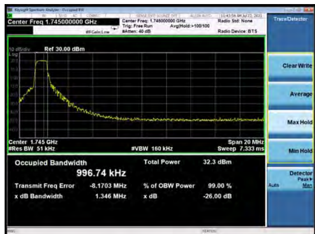
LTE eMTC Band 66 16QAM 20MHz CH-Middle
