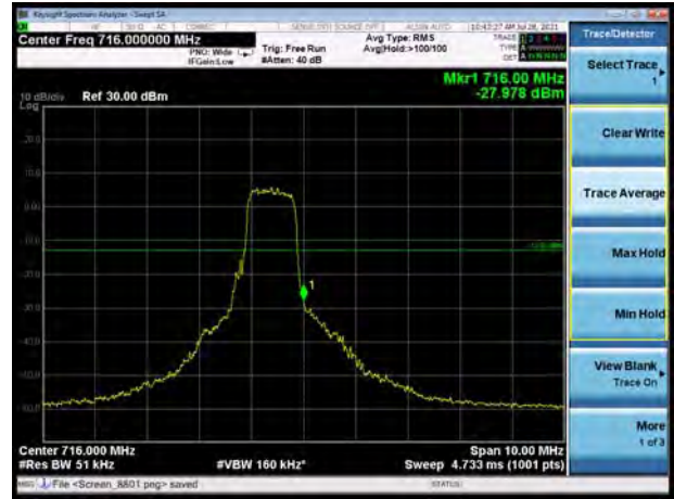
LTE eMTC Band 12 16QAM 3MHz CH-High, 1 RB
