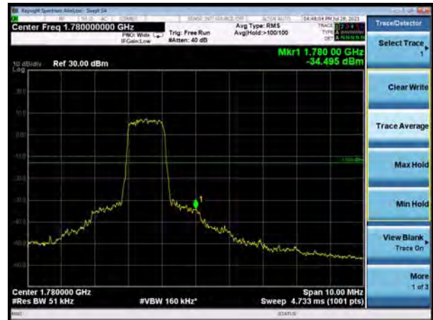
LTE eMTC Band 66 QPSK 20MHz CH-High, 1 RB
