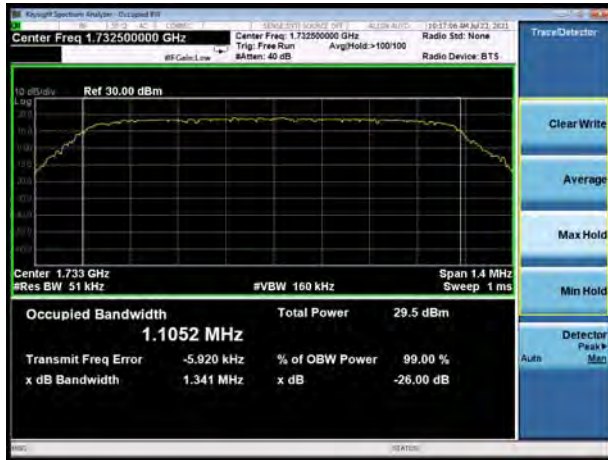
LTE eMTC Band 4 QPSK 5MHz CH-Middle
