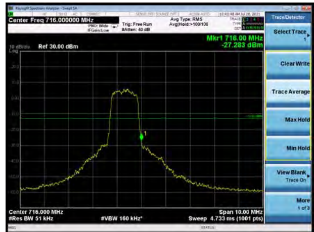
LTE eMTC Band 12 QPSK 3MHz CH-High, 1 RB
