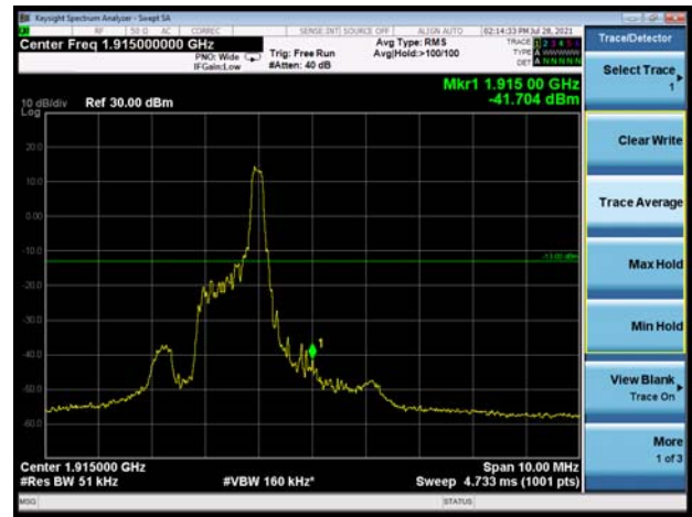
LTE eMTC Band 25 15MHz QPSK 100%RB CH-High
