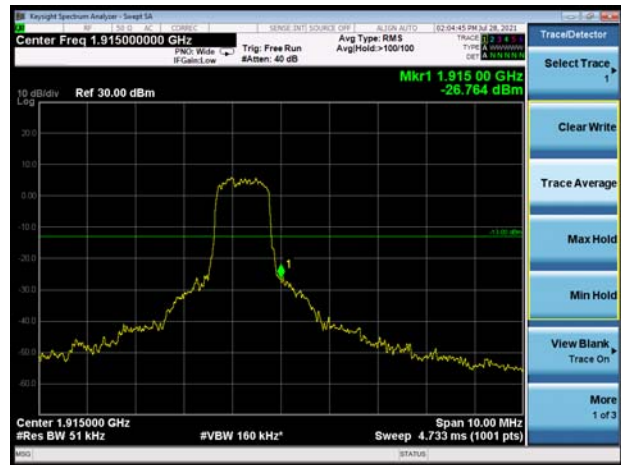
LTE eMTC Band 25 10MHz QPSK 1RB CH-High
