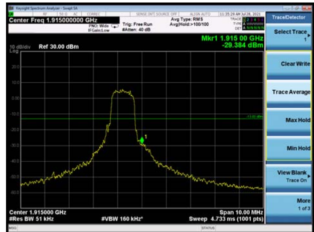
LTE eMTC Band 25 5MHz 16QAM 1RB CH-High
