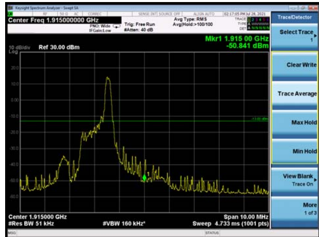
LTE eMTC Band 25 20MHz 16QAM 1RB CH-High
