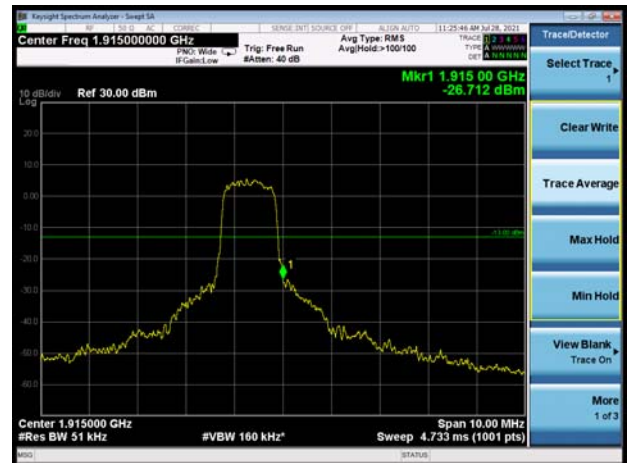
LTE eMTC Band 25 3MHz QPSK 1RB CH-High
