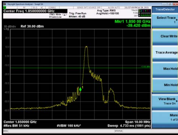
LTE eMTC Band 25 3MHz 16QAM 100%RB CH-Low
