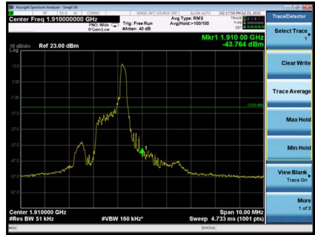
LTE eMTC Band 2 10MHz QPSK 100%RB CH-High
