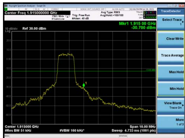
LTE eMTC Band 25 10MHz QPSK 100%RB CH-High
