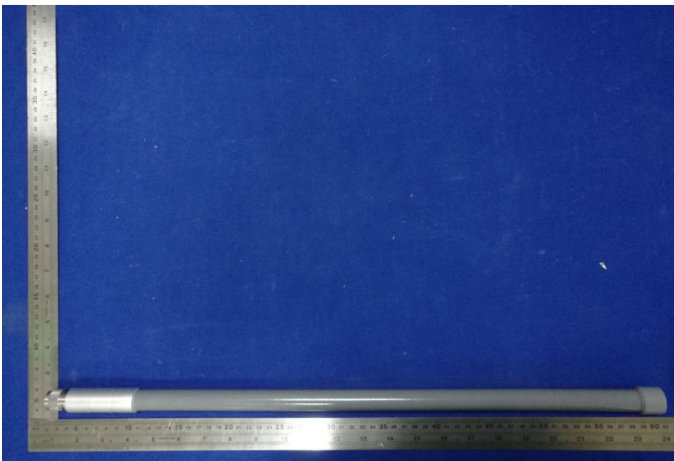
EUT – 5G WIFI Antenna View
