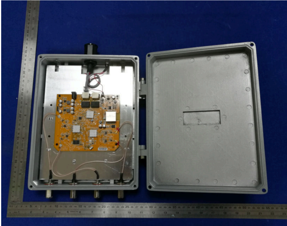
EUT - Open View
