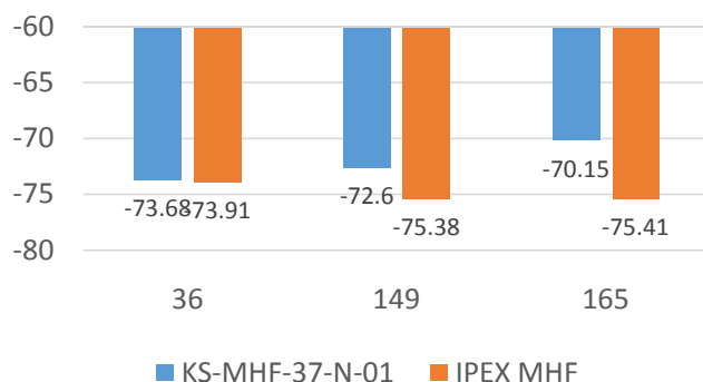
TIS (802.11n)
