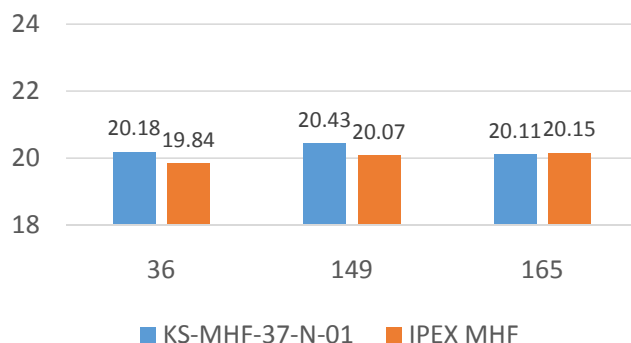
TRP (802.11n)
