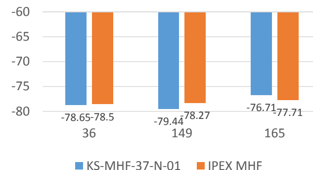
TIS (802.11ac)
