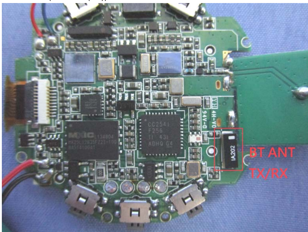
(20) EUT Photo (Antenna (BT))
