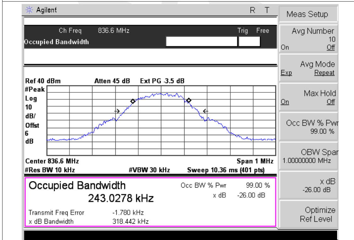
Occupied Bandwidth (99%) GSM 850 BAND CH 190
