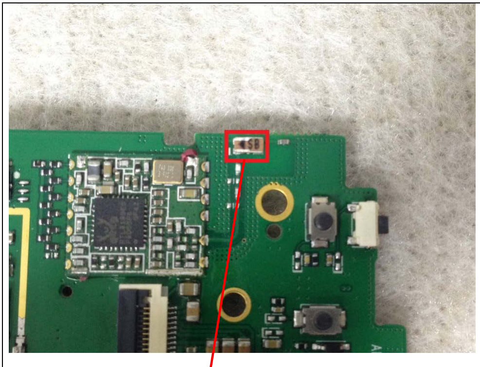
Chip Antenna
