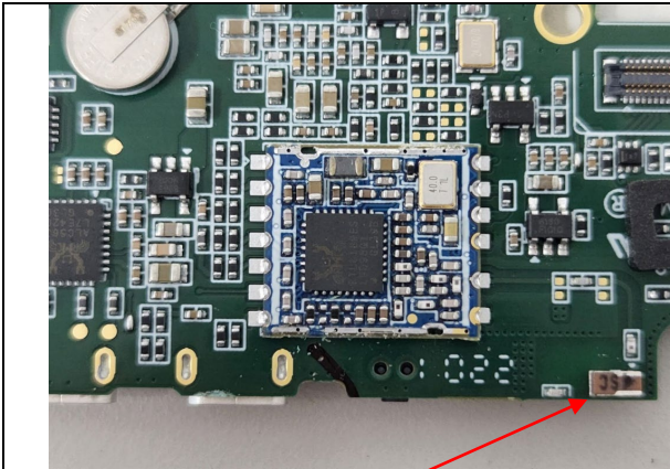
Chip Antenna
