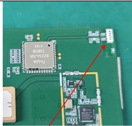
Chip Antenna
