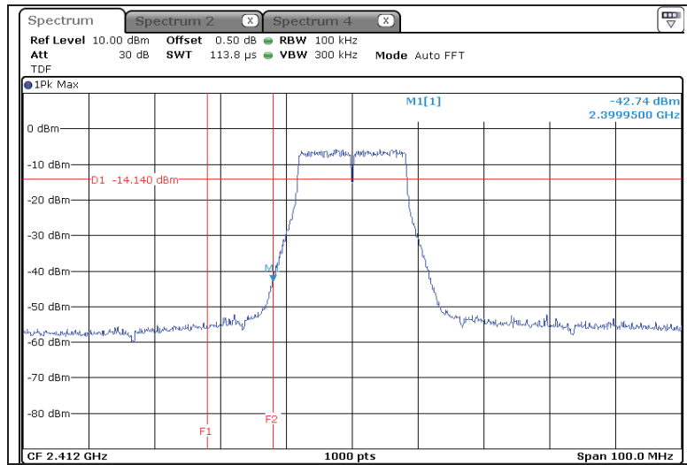
* Result of 2 400.0 MHz (F1:2 390 MHz, F2:2 400 MHz)
