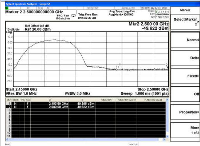
802.11b-High channel(Peak)
