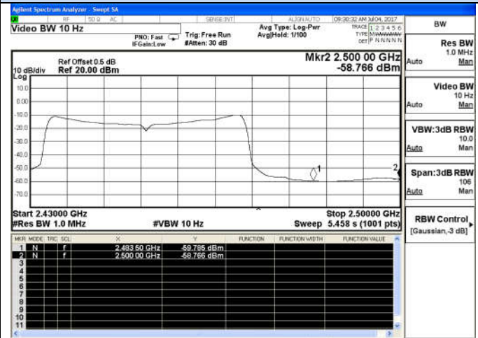
802.11n(HT40)-High channel(Average)
