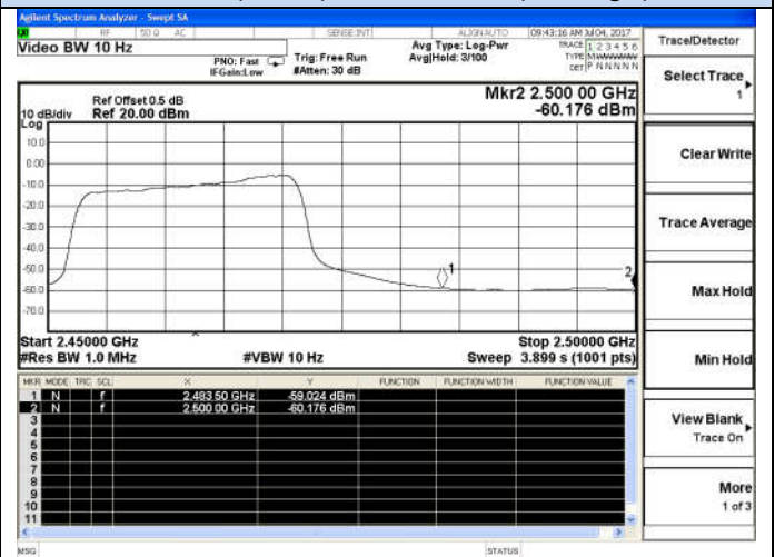
802.11n(HT20)-High channel(Average)
