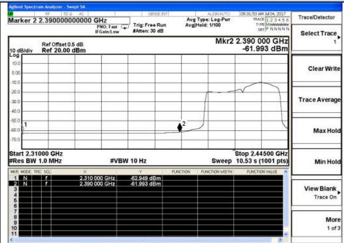
802.11n(HT40)-Low channel(Average)
