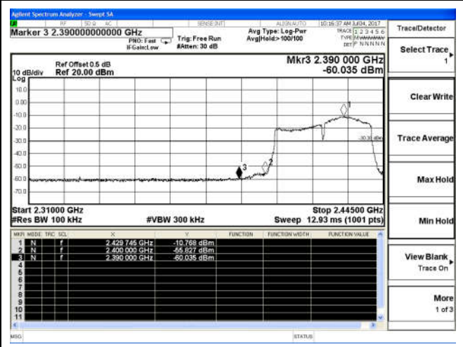
Channel 3 / 2422 MHz
