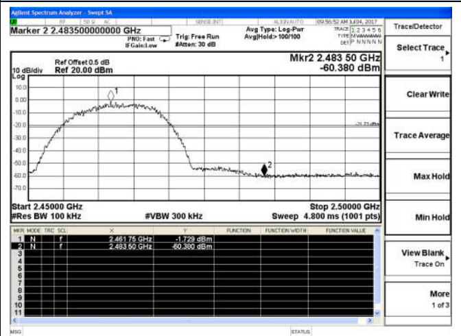
Channel 11 / 2462 MHz
