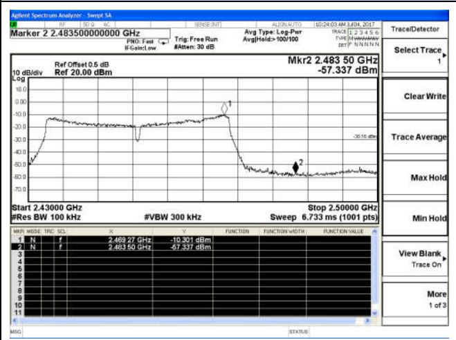
Channel 9 / 2452 MHz
