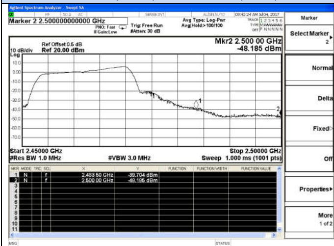
802.11n(HT20)-High channel(Peak)
