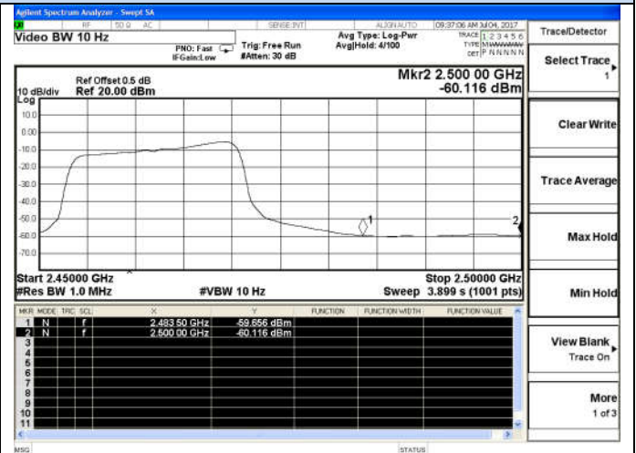
802.11g-High channel(Average)
