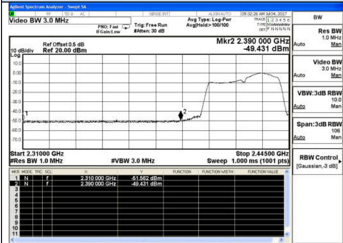
802.11n(HT40)-Low channel(Peak)
