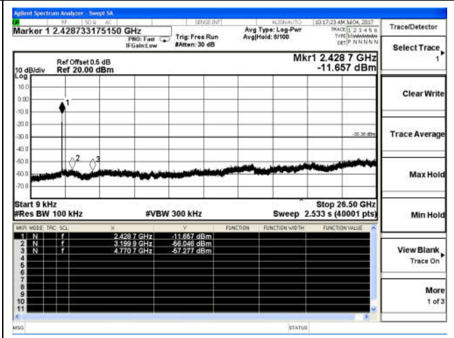
9 KHz – 26.5 GHz
