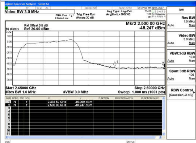
802.11g-High channel(Peak)
