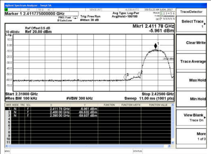
Channel 1 / 2412 MHz
