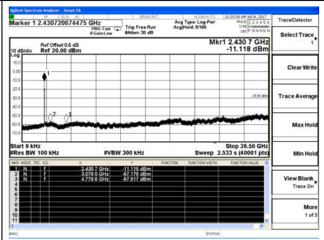
9 KHz – 26.5 GHz
