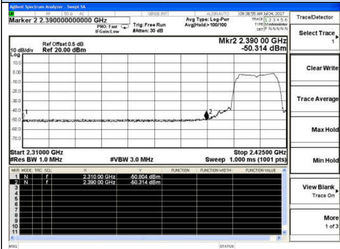
802.11g-Low channel(Peak)
