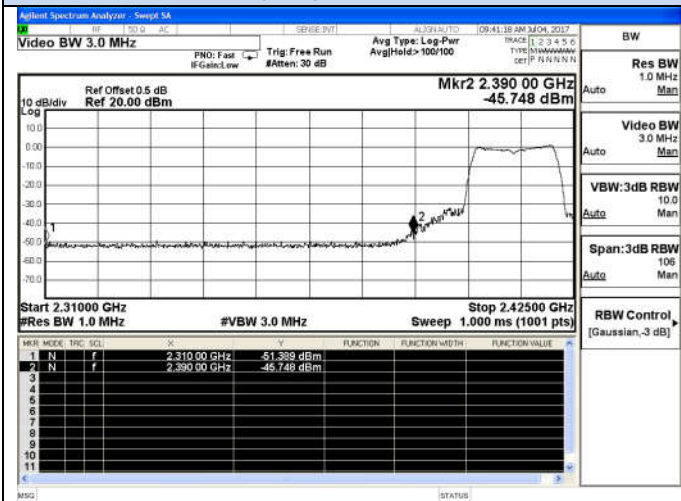
802.11n(HT20)-Low channel(Peak)
