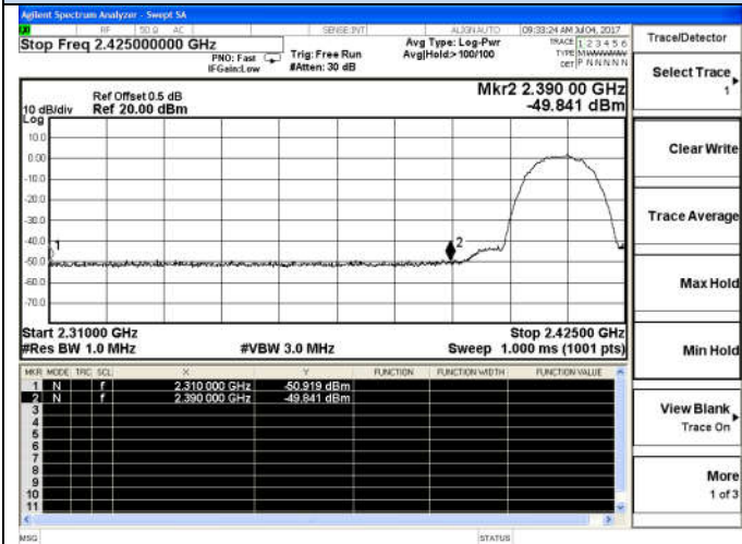
802.11b-Low channel(Peak)
