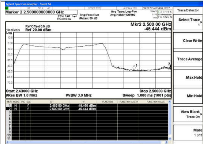
802.11n(HT40)-High channel(Peak)
