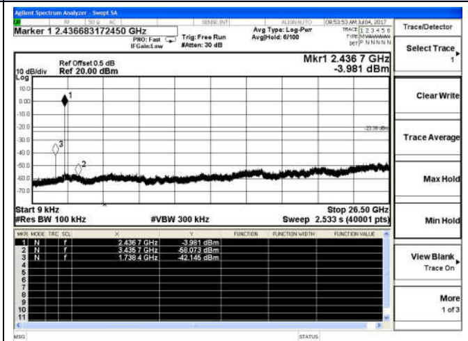
9 KHz – 26.5 GHz
