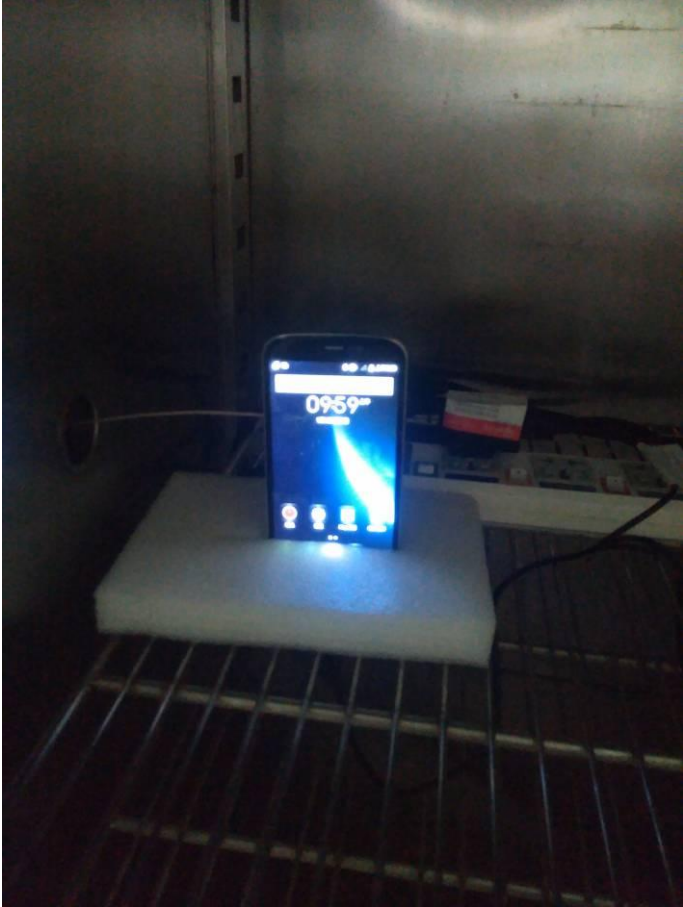
Photograph – Extreme Condition Test Setup
