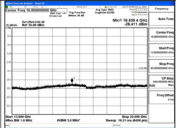
13.6 GHz – 20 GHz
