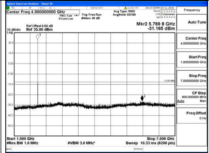
1 GHz – 7 GHz
