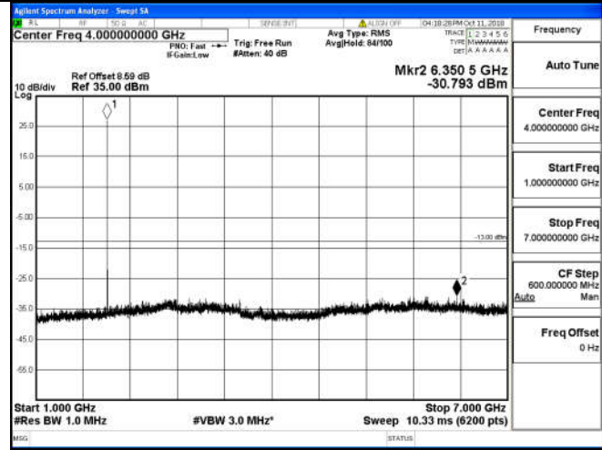
1 GHz – 7 GHz
