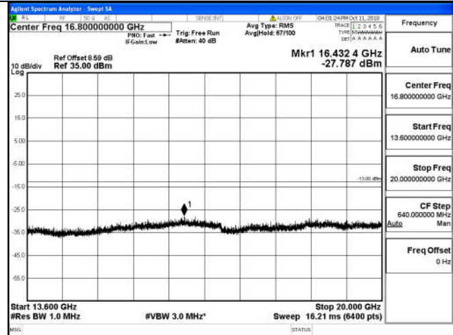
13.6 GHz – 20 GHz
