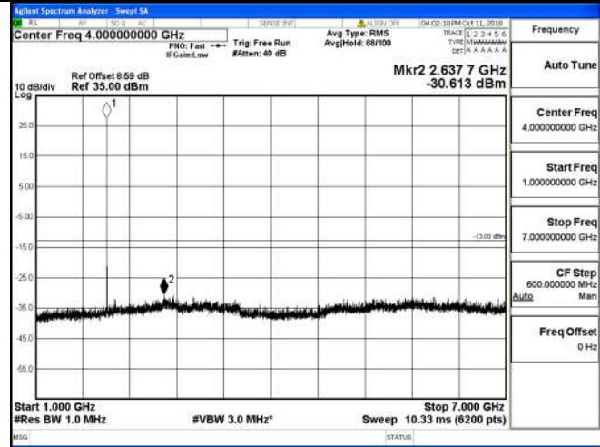
1 GHz – 7 GHz
