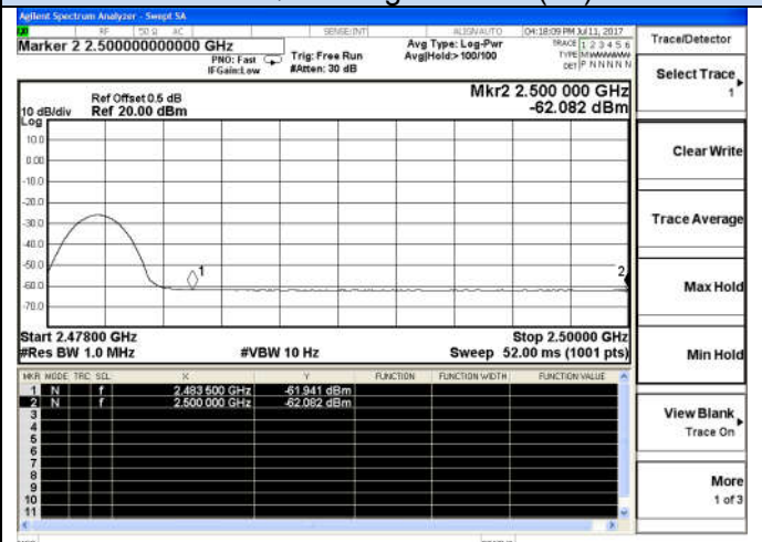
8-DPQK-High channel(Av)
