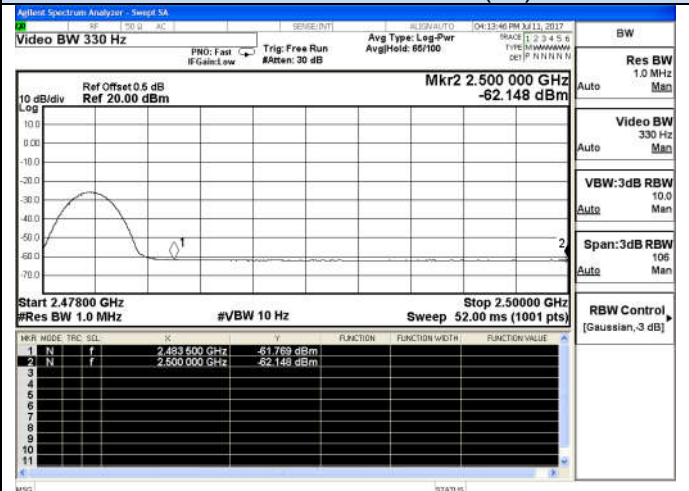
Pi/4-DQPSK-High channel(Av)
