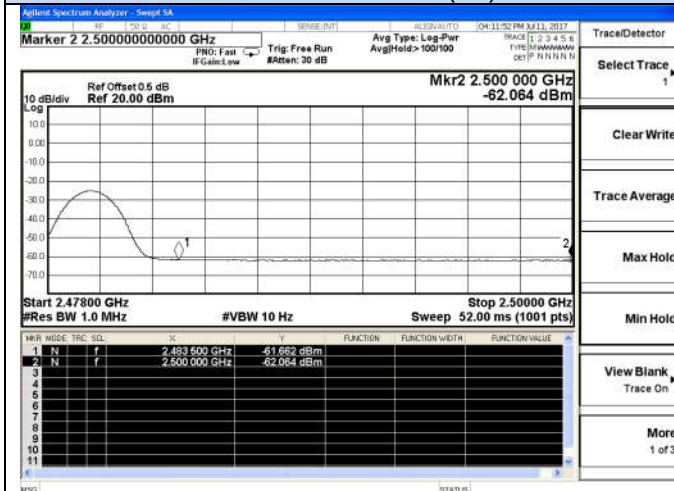
GFSK-High channel(Av)
