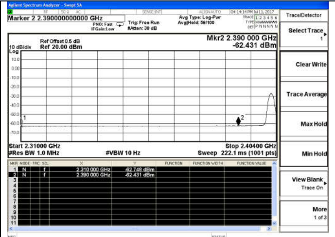
Pi/4-DQPSK-Low channel(Av)
