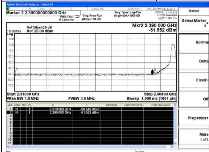
GFSK-Low channel(Peak)
