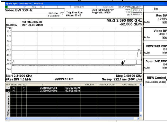
8-DPQK-Low channel(Av)
