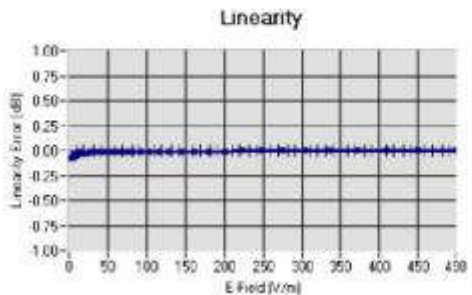
Linearity \pm 1.61\% ( \pm 0.07\text{dB} )
