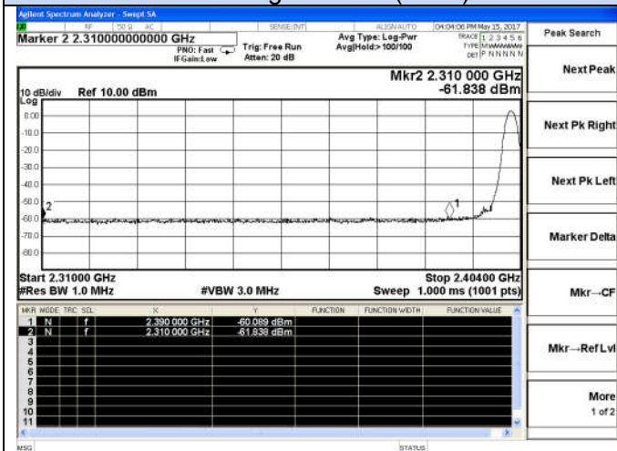
8-DPQK-Low channel(Peak)
