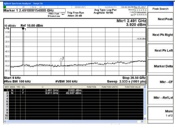
9 KHz – 26.5 GHz
