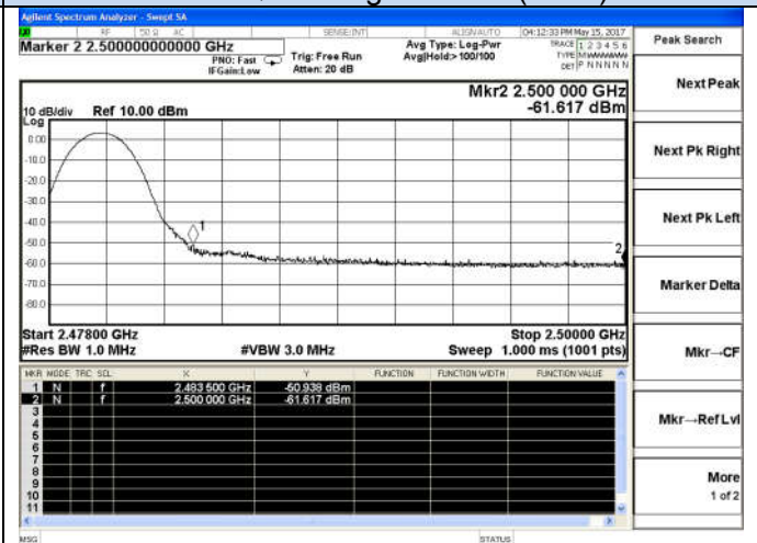
8-DPQK-High channel(Peak)
