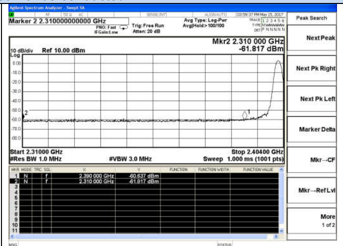
Pi/4-DQPSK-Low channel(Peak)
