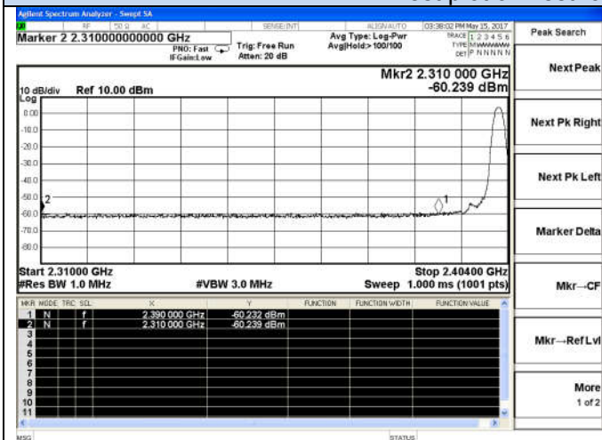
GFSK-Low channel(Peak)
