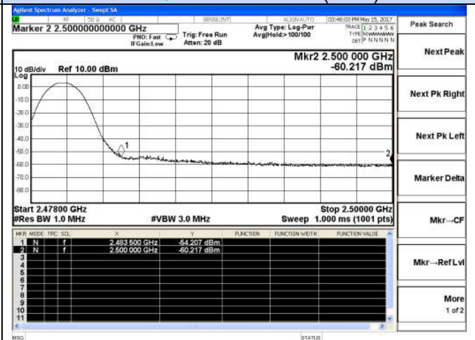
Pi/4-DQPSK-High channel(Peak)
