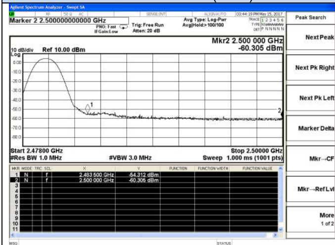
GFSK-High channel(Peak)
