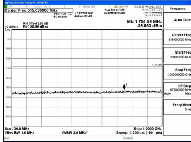
30 MHz – 1000 MHz
