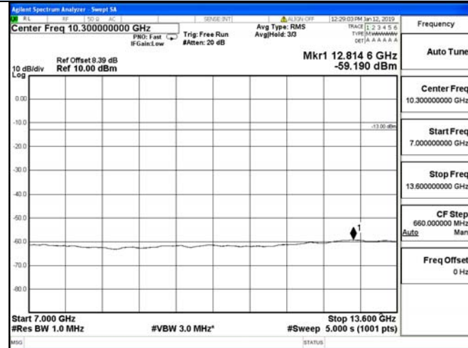
7 GHz – 13.6 GHz
