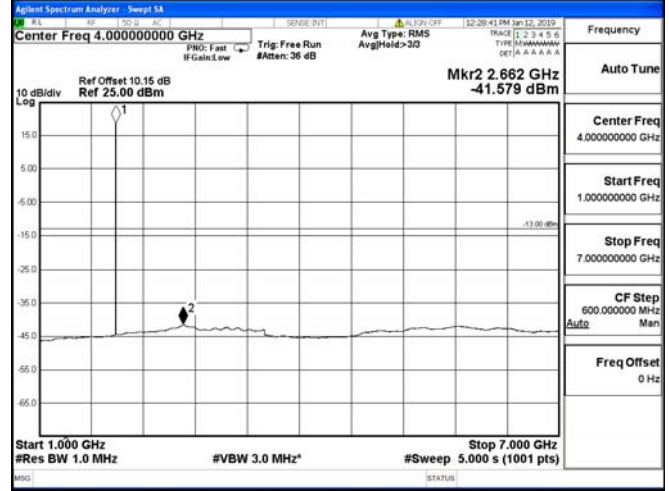
1 GHz – 7 GHz
