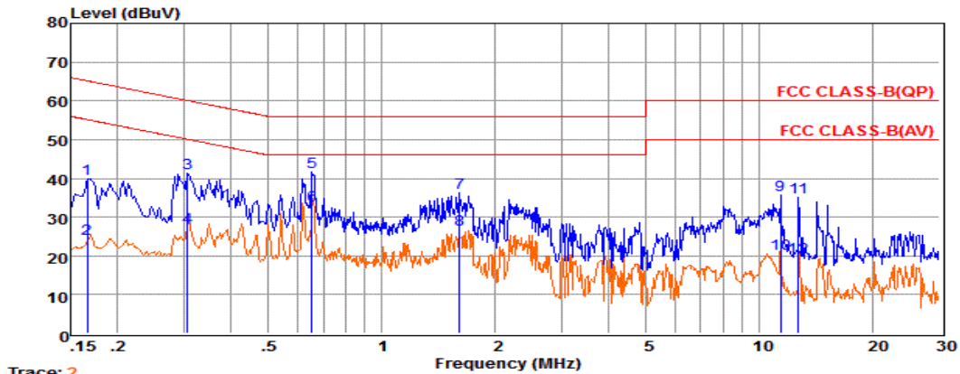
Trace: 2 Pol:
