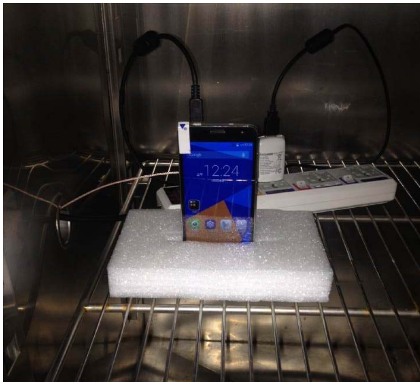
Photograph – Extreme Condition Test Setup
