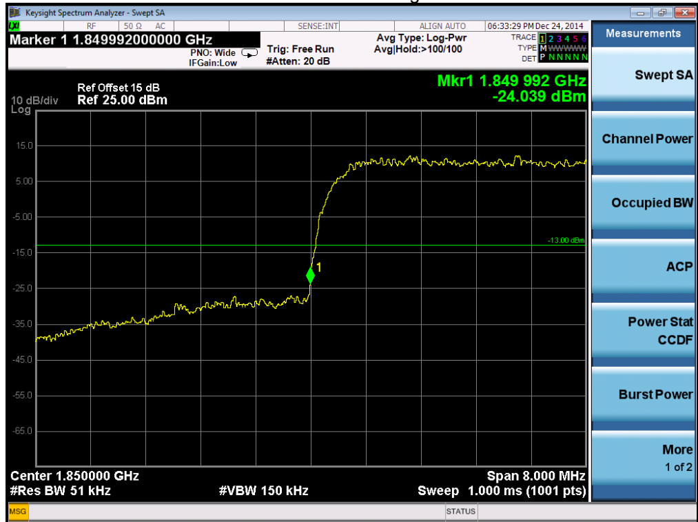
WCDMA band II band edge-left side
