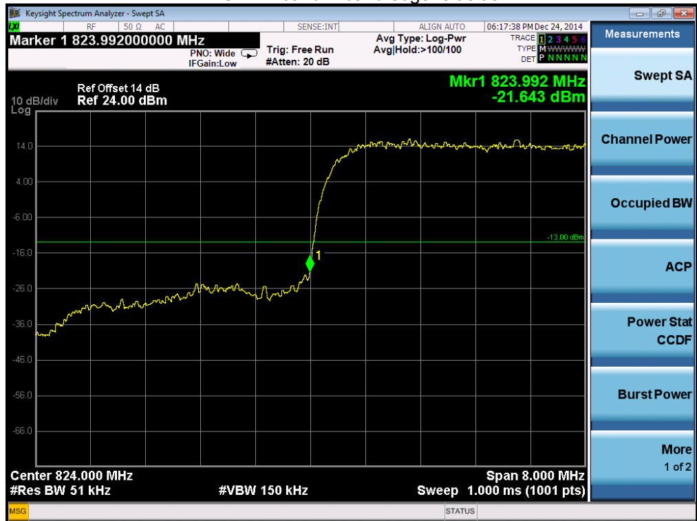
WCDMA band V band edge-left side
