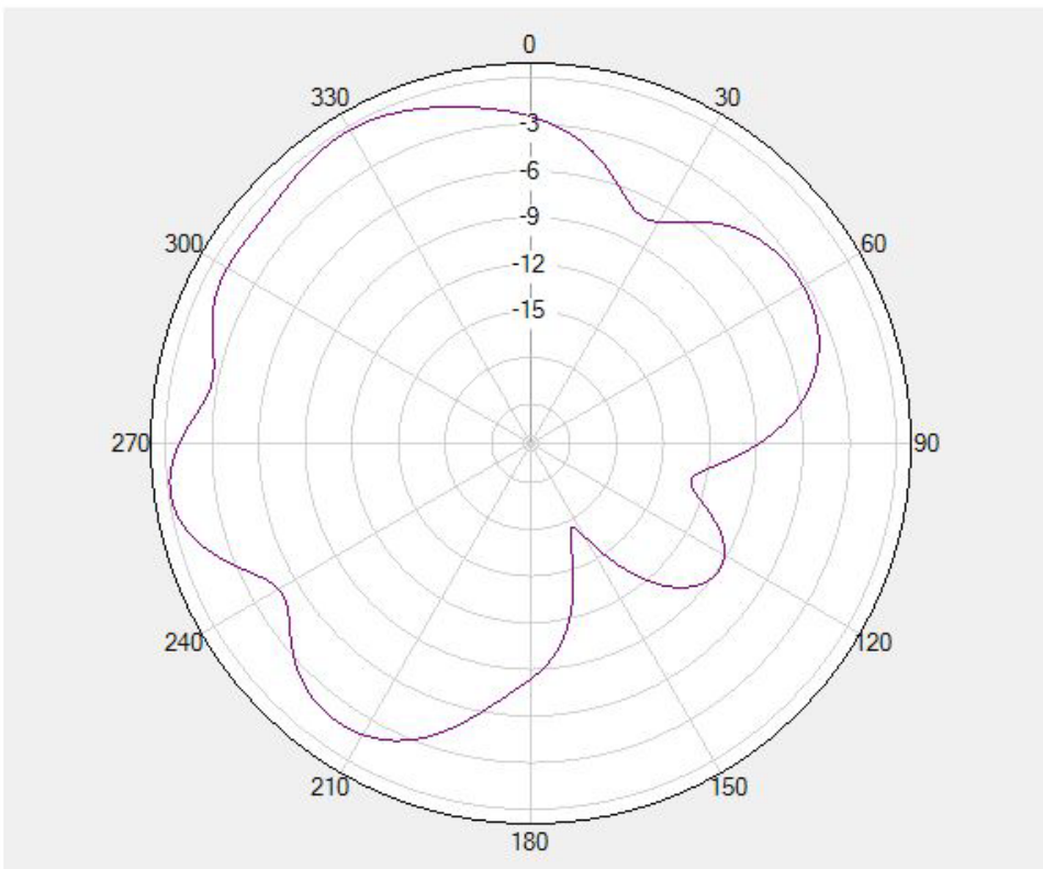
Vertical (2450 MHZ)
