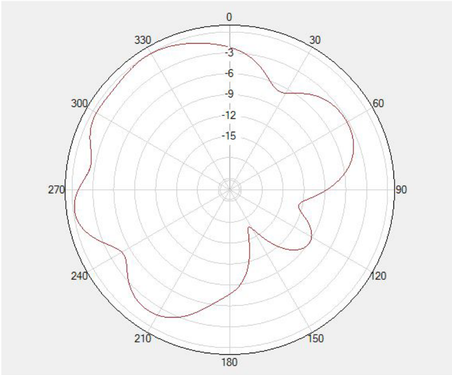
Vertical (2480 MHz)
