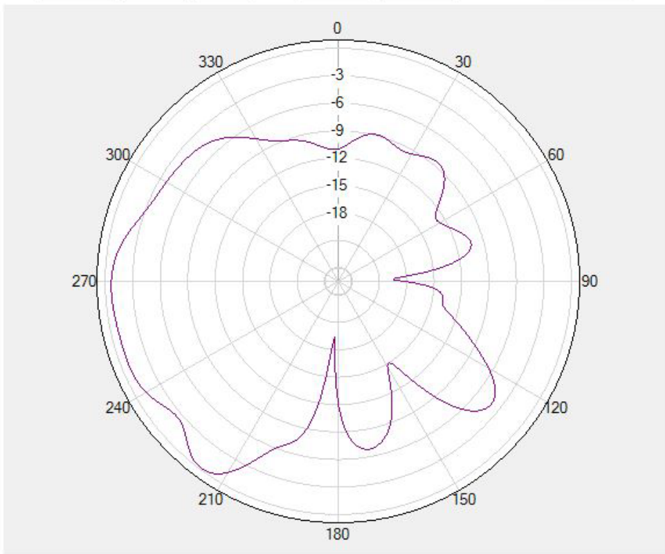
Horizontal (2450 MHZ)
