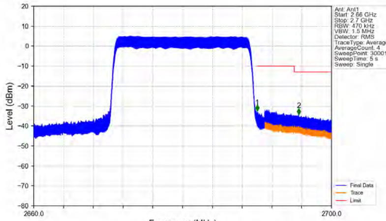
Band41_20MHz_64QAM_HCH_2680MHz_RB_100_0_NTNV
