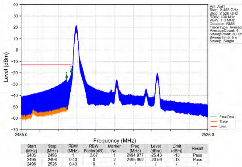
Band41_20MHz_16QAM_LCH_2506MHz_RB_1_0_NTNV
