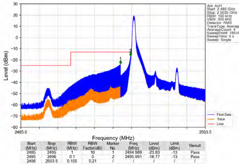
Band41_5MHz_16QAM_LCH_2498.5MHz_RB_1_0_NTNV
