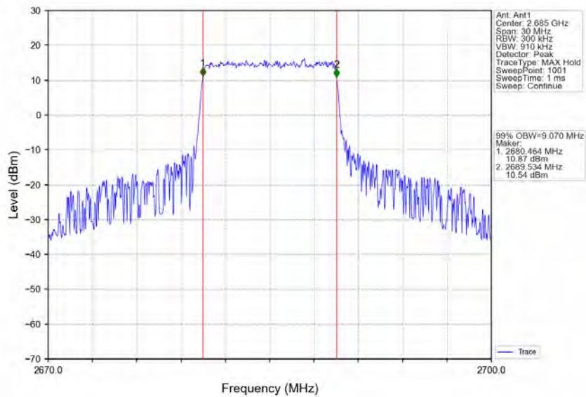
Band41_10MHz_64QAM_HCH_2685MHz_RB_50_0_NTNV
