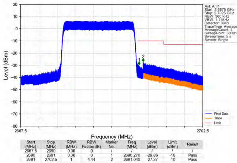
Band41_15MHz_16QAM_HCH_2682.5MHz_RB_75_0_NTNV
