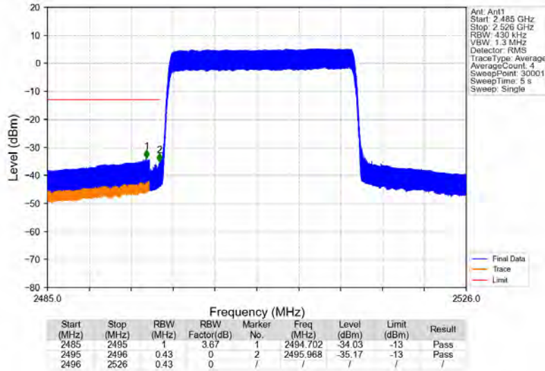
Band41_20MHz_64QAM_LCH_2506MHz_RB_100_0_NTNV
