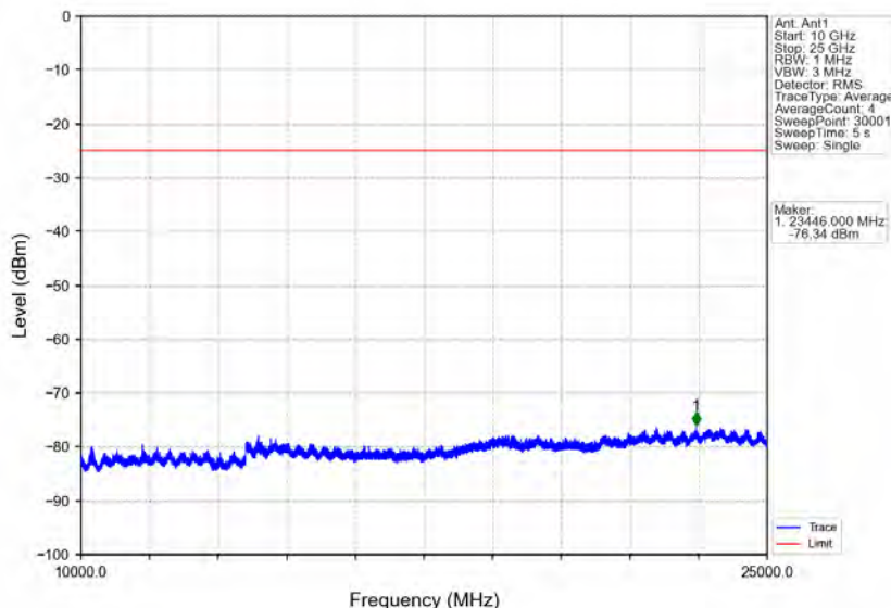
Band41_20MHz_64QAM_HCH_2680MHz_RB_1_0_NTNV
