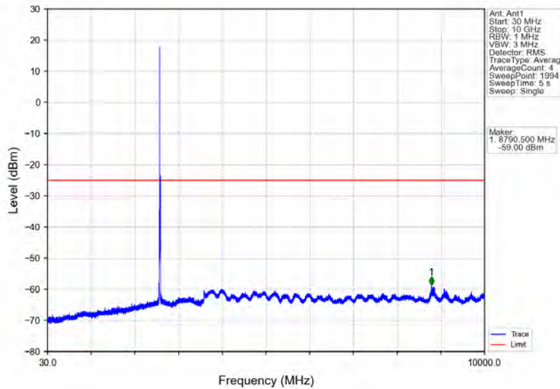
Band41_10MHz_64QAM_MCH_2593MHz_RB_1_0_NTNV
