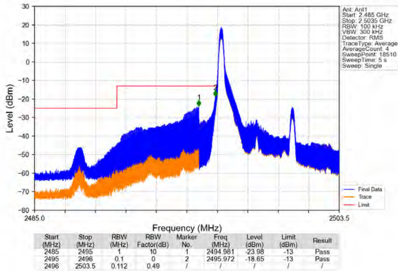
Band41_5MHz_64QAM_LCH_2498.5MHz_RB_1_0_NTNV
