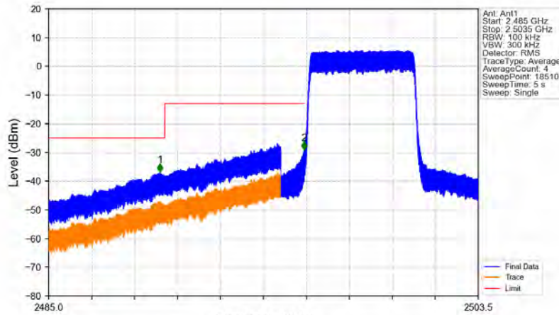
Band41_5MHz_16QAM_LCH_2498.5MHz_RB_25_0_NTNV
