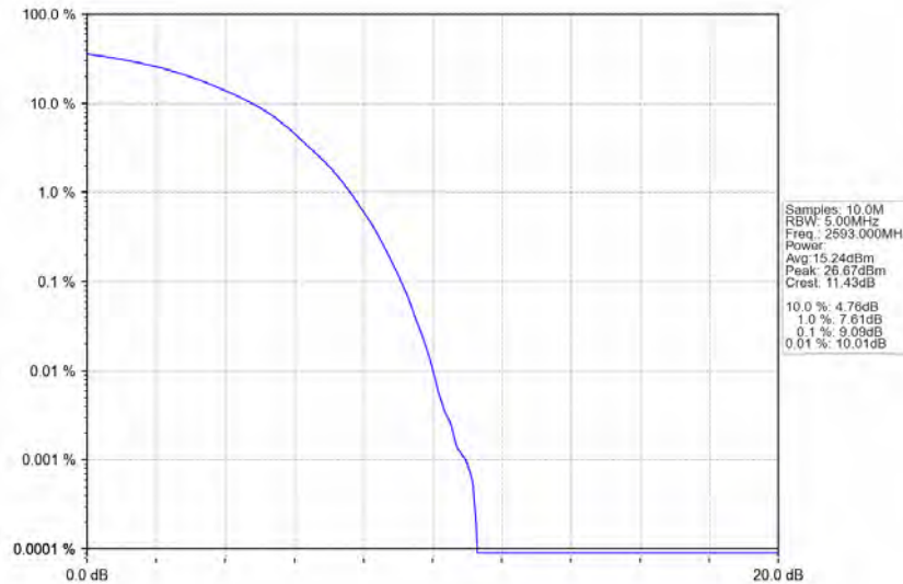
Band41_15MHz_16QAM_MCH_2593MHz_RB_75_0_NTNV
