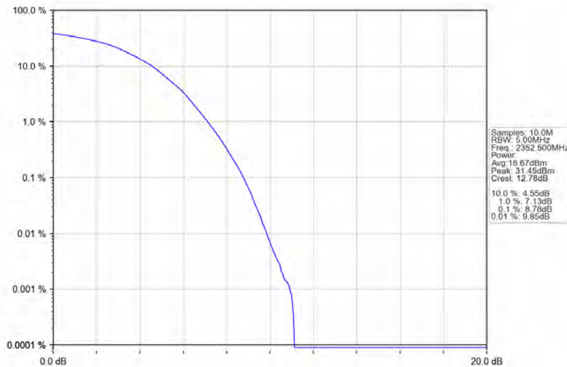
Band40b_5MHz_64QAM_LCH_2352.5MHz_RB_25_0_NTNV
