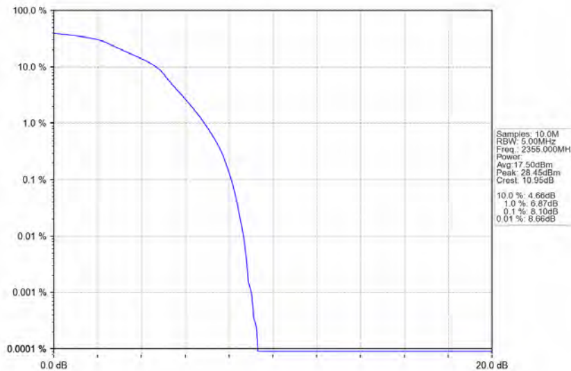
Band40b_5MHz_16QAM_MCH_2355MHz_RB_25_0_NTNV
