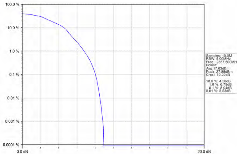
Band40b_5MHz_16QAM_HCH_2357.5MHz_RB_25_0_NTNV
