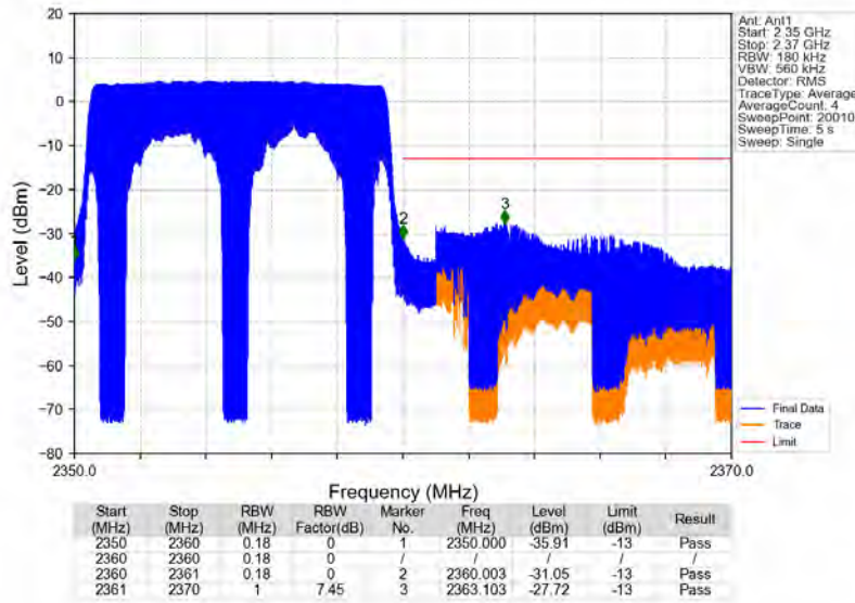
Band40b_10MHz_16QAM_HCH_2355MHz_RB_50_0_NTNV
