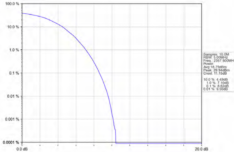
Band40b_5MHz_64QAM_HCH_2357.5MHz_RB_25_0_NTNV
