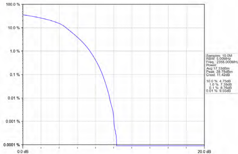
Band40b_10MHz_64QAM_HCH_2355MHz_RB_50_0_NTNV
