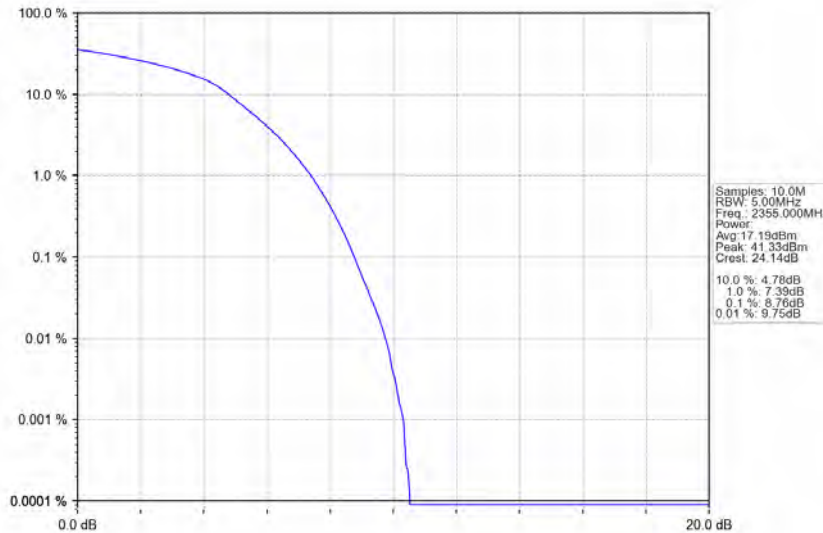
Band40b_10MHz_64QAM_MCH_2355MHz_RB_50_0_NTNV
