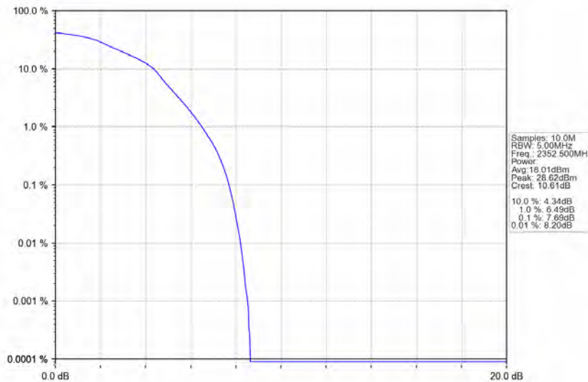
Band40b_5MHz_16QAM_LCH_2352.5MHz_RB_25_0_NTNV
