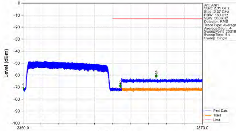
Band40b_10MHz_64QAM_HCH_2355MHz_RB_50_0_NTNV
