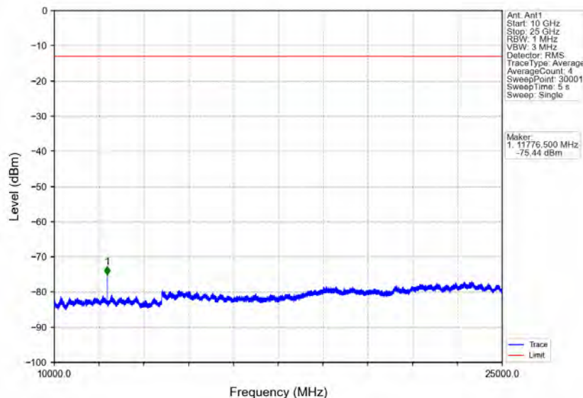
Band40b_5MHz_16QAM_HCH_2357.5MHz_RB_1_0_NTNV
