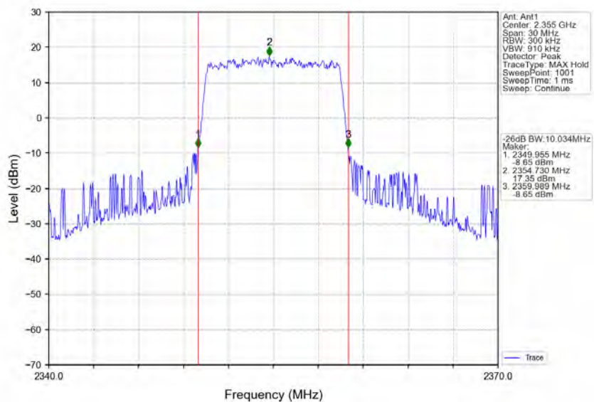
Band40b_10MHz_64QAM_LCH_2355MHz_RB_50_0_NTNV
