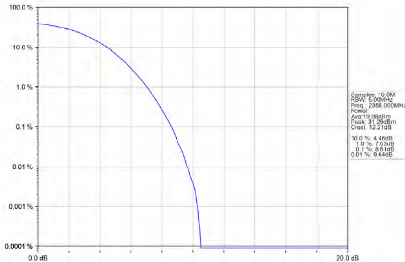
Band40b_5MHz_64QAM_MCH_2355MHz_RB_25_0_NTNV
