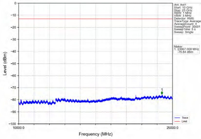
Band40b_5MHz_64QAM_HCH_2357.5MHz_RB_1_0_NTNV
