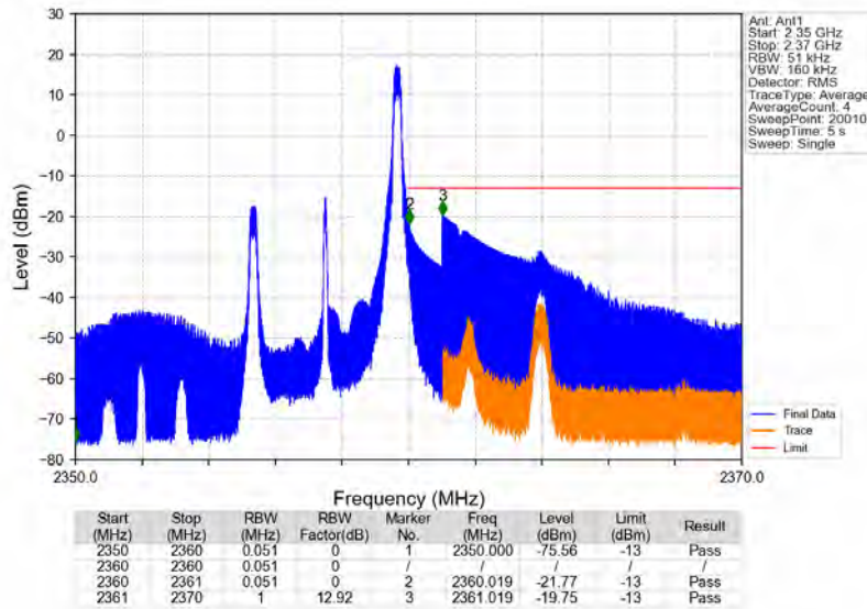
Band40b_5MHz_64QAM_HCH_2357.5MHz_RB_1_24_NTNV
