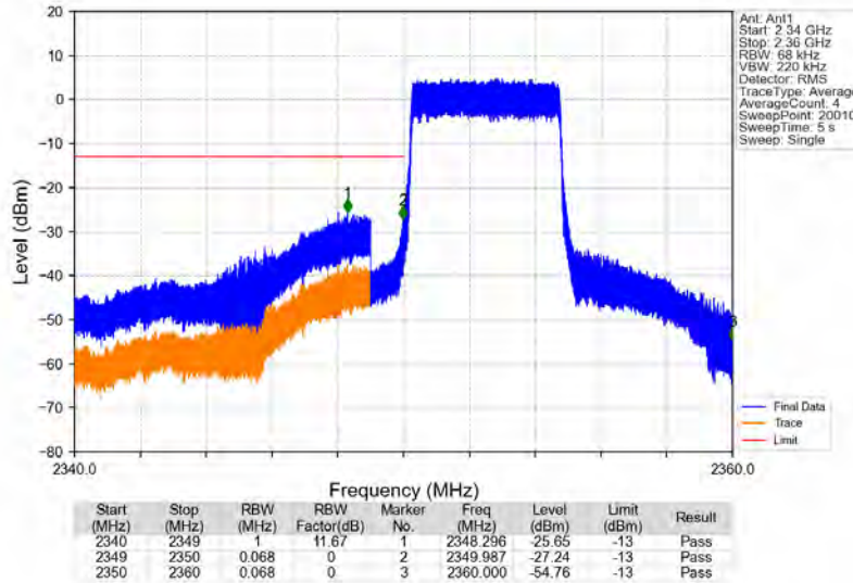
Band40b_5MHz_QPSK_LCH_2352.5MHz_RB_25_0_NTNV
