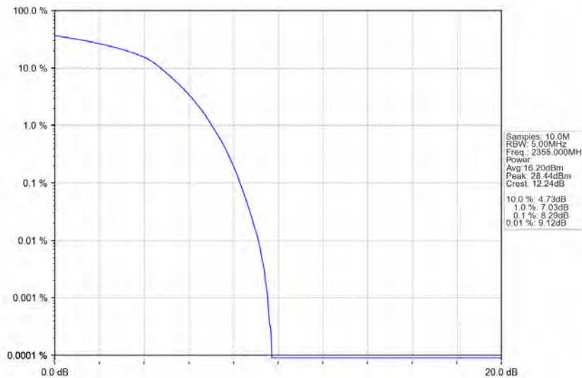
Band40b_10MHz_16QAM_HCH_2355MHz_RB_50_0_NTNV
