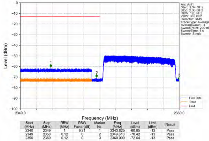
Band40b_10MHz_64QAM_LCH_2355MHz_RB_50_0_NTNV
