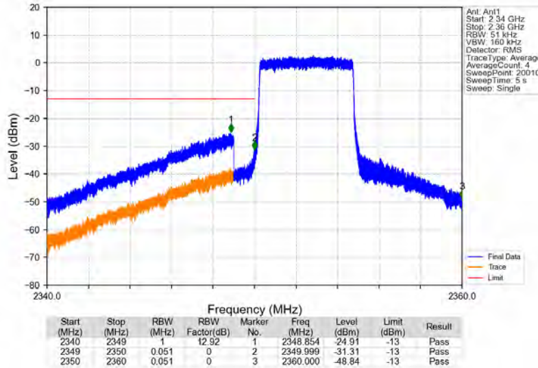
Band40b_5MHz_64QAM_LCH_2352.5MHz_RB_25_0_NTNV
