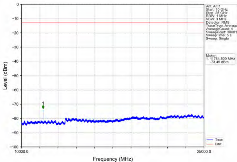
Band40b_5MHz_16QAM_MCH_2355MHz_RB_1_0_NTNV
