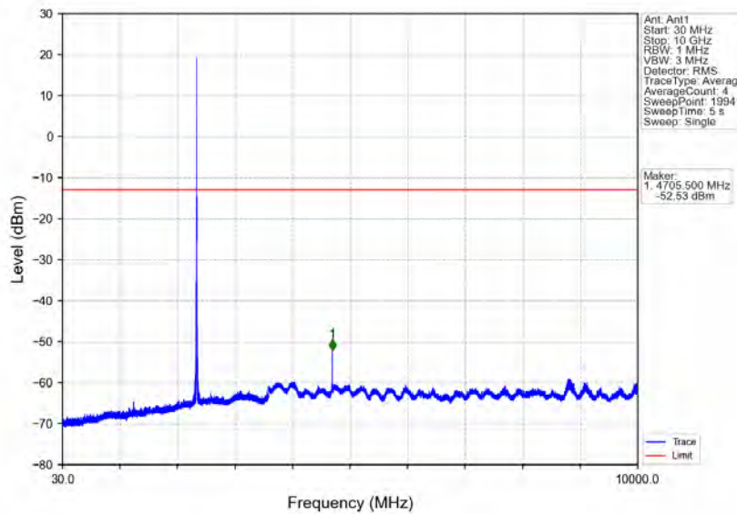
Band40b_5MHz_64QAM_MCH_2355MHz_RB_1_0_NTNV
