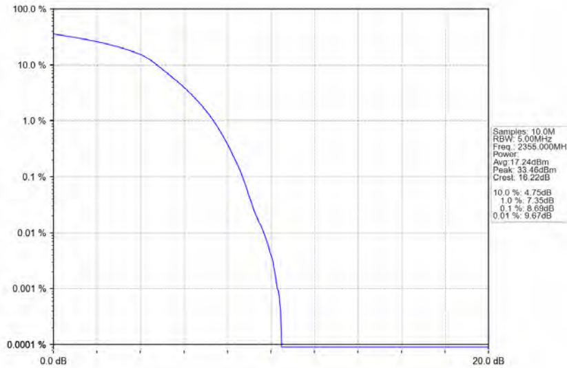
Band40b_10MHz_64QAM_LCH_2355MHz_RB_50_0_NTNV
