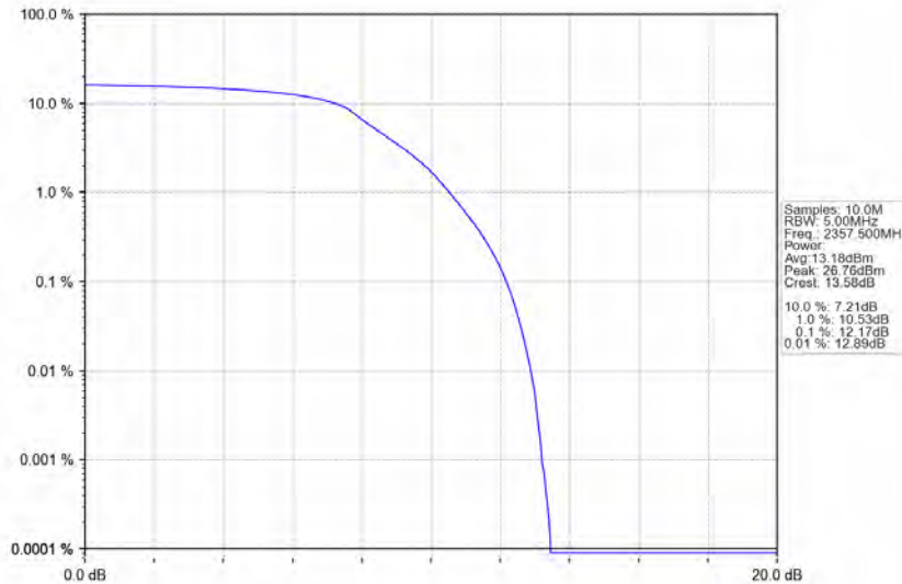
Band40b_5MHz_QPSK_HCH_2357.5MHz_RB_25_0_NTNV
