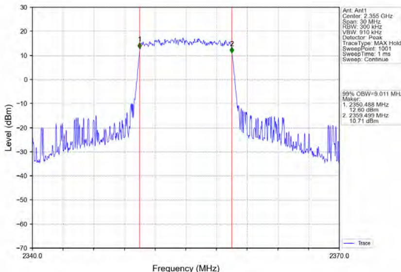
Band40b_10MHz_64QAM_LCH_2355MHz_RB_50_0_NTNV
