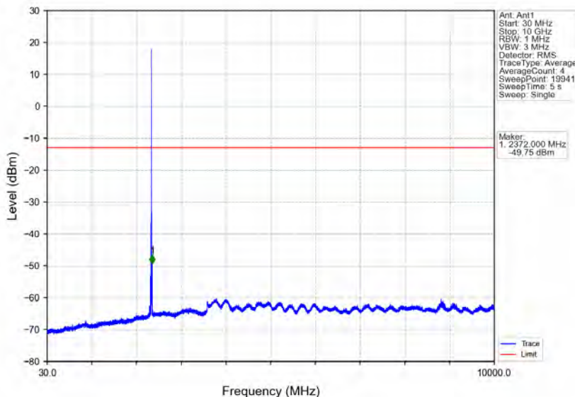
Band40b_5MHz_16QAM_MCH_2355MHz_RB_1_0_NTNV
