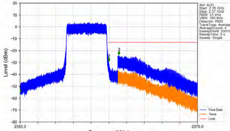
Band40b_5MHz_64QAM_HCH_2357.5MHz_RB_25_0_NTNV
