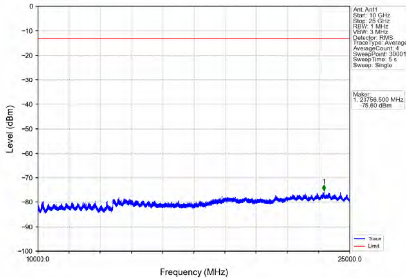
Band40b_5MHz_64QAM_MCH_2355MHz_RB_1_0_NTNV
