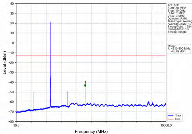
Band40a_5MHz_64QAM_LCH_2307.5MHz_RB_1_0_NTNV
