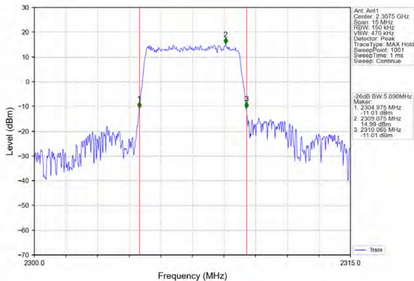
Band40a_5MHz_16QAM_LCH_2307.5MHz_RB_25_0_NTNV
