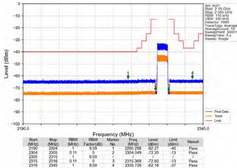
Band40a_10MHz_64QAM_HCH_2310MHz_RB_50_0_NTNV
