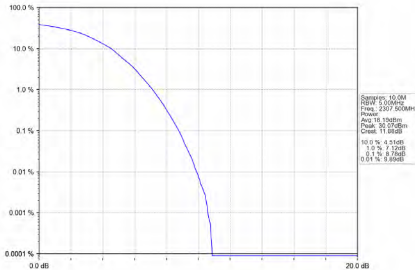
Band40a_5MHz_64QAM_LCH_2307.5MHz_RB_25_0_NTNV
