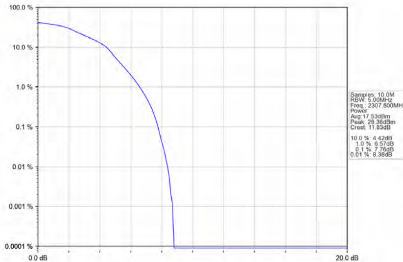
Band40a_5MHz_16QAM_LCH_2307.5MHz_RB_25_0_NTNV
