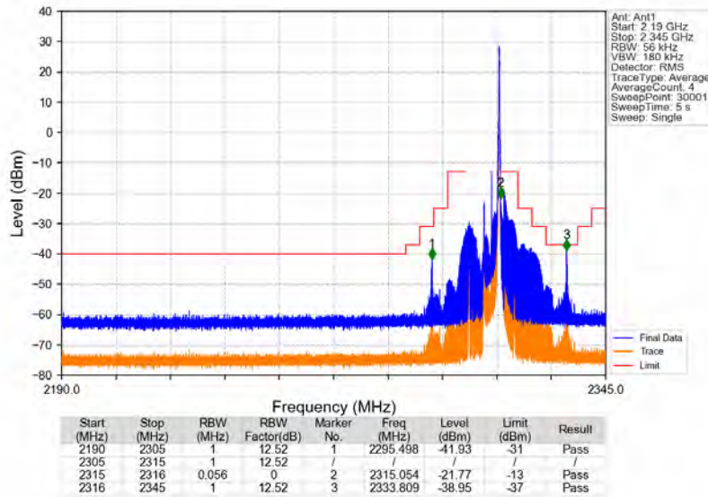
Band40a_5MHz_16QAM_HCH_2312.5MHz_RB_25_0_NTNV
