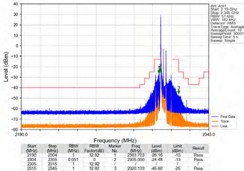
Band40a_5MHz_64QAM_LCH_2307.5MHz_RB_1_0_NTNV
