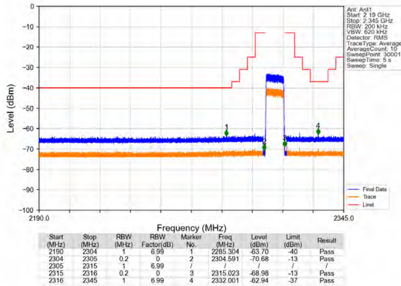
Band40a_10MHz_64QAM_MCH_2310MHz_RB_1_0_NTNV
