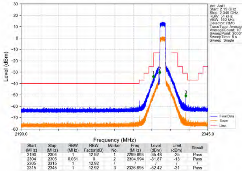
Band40a_5MHz_64QAM_MCH_2310MHz_RB_1_0_NTNV
