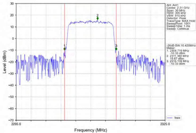
Band40a_10MHz_64QAM_LCH_2310MHz_RB_50_0_NTNV
