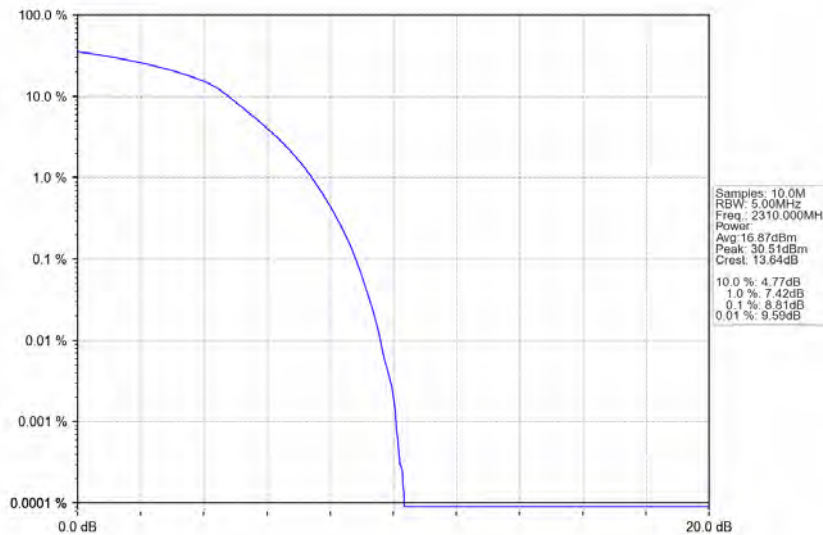
Band40a_10MHz_64QAM_MCH_2310MHz_RB_50_0_NTNV
