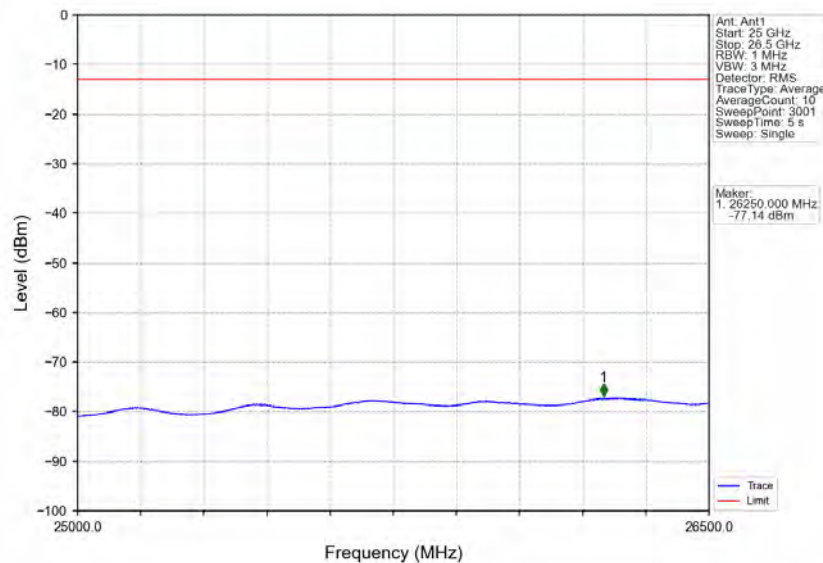
Band40a_5MHz_64QAM_MCH_2310MHz_RB_1_0_NTNV
