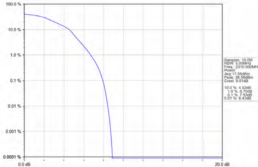
Band40a_5MHz_16QAM_MCH_2310MHz_RB_25_0_NTNV
