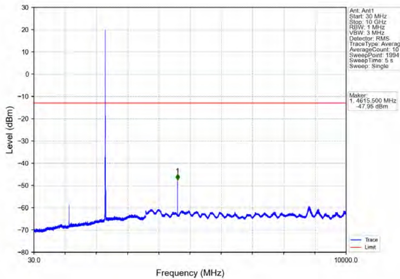
Band40a_5MHz_64QAM_MCH_2310MHz_RB_1_0_NTNV
