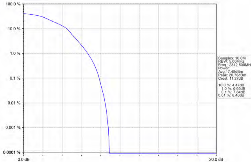
Band40a_5MHz_16QAM_HCH_2312.5MHz_RB_25_0_NTNV
