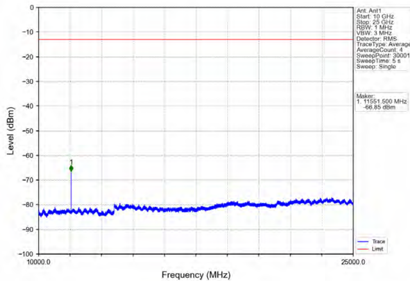
Band40a_5MHz_16QAM_HCH_2312.5MHz_RB_1_0_NTNV
