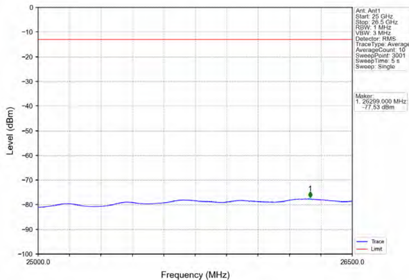
Band40a_10MHz_64QAM_MCH_2310MHz_RB_1_0_NTNV
