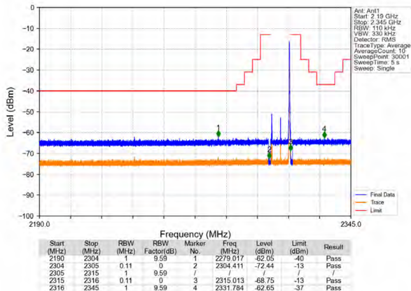
Band40a_10MHz_64QAM_HCH_2310MHz_RB_1_49_NTNV
