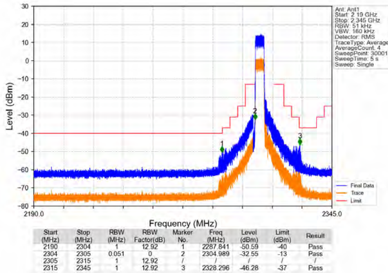
Band40a_5MHz_16QAM_LCH_2307.5MHz_RB_25_0_NTNV
