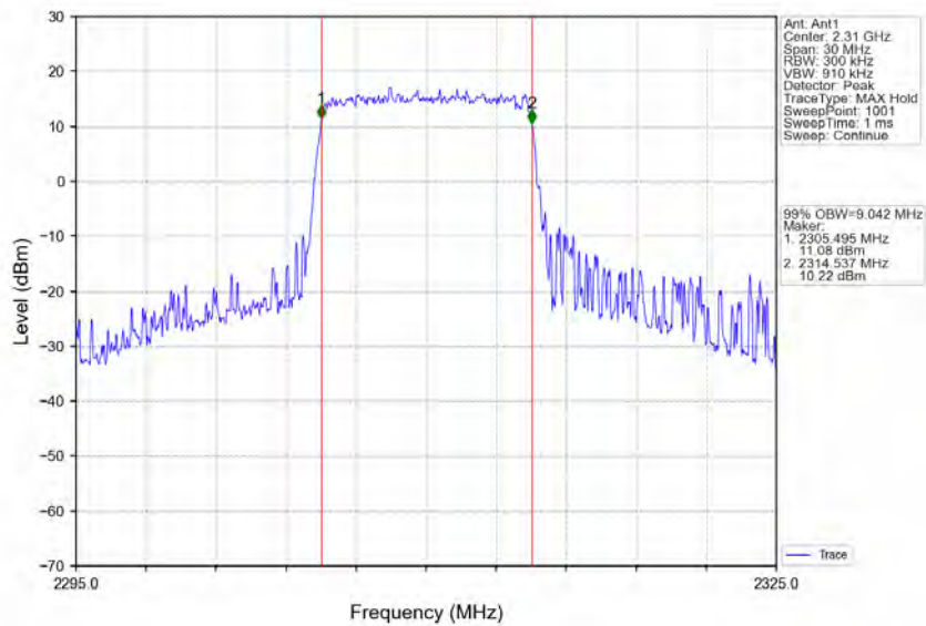
Band40a_10MHz_64QAM_HCH_2310MHz_RB_50_0_NTNV
