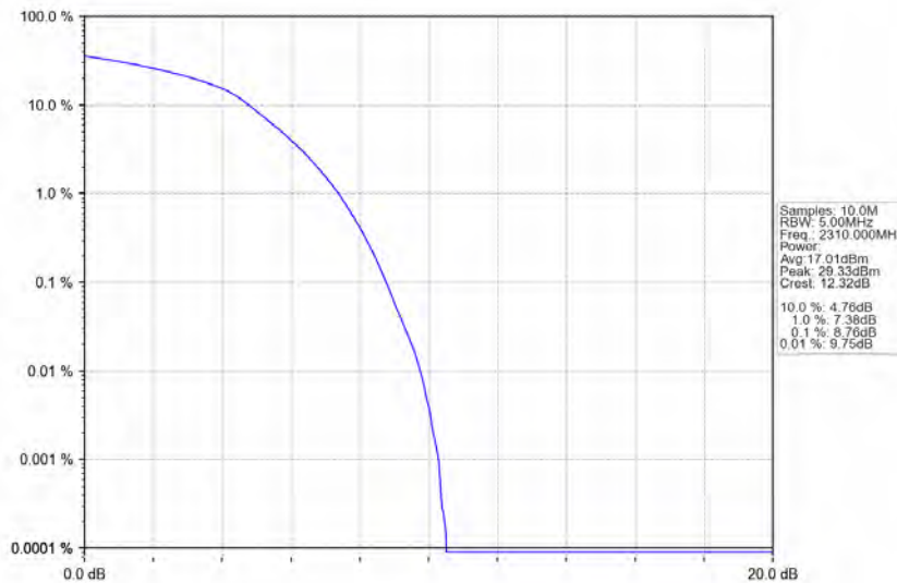
Band40a_10MHz_64QAM_LCH_2310MHz_RB_50_0_NTNV
