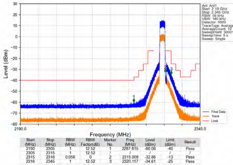
Band40a_5MHz_64QAM_HCH_2312.5MHz_RB_25_0_NTNV
