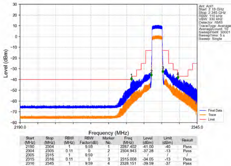
Band40a_10MHz_16QAM_HCH_2310MHz_RB_50_0_NTNV
