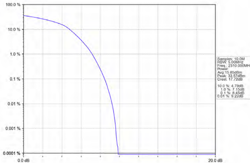
Band40a_10MHz_16QAM_HCH_2310MHz_RB_50_0_NTNV
