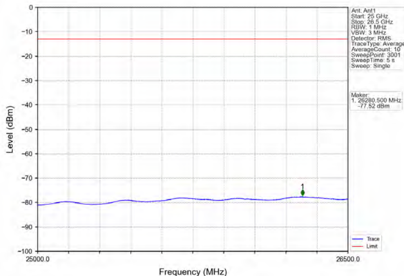
Band40a_10MHz_64QAM_HCH_2310MHz_RB_1_49_NTNV
