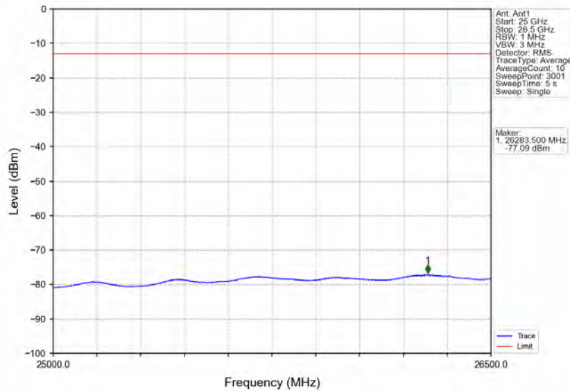
Band40a_5MHz_64QAM_HCH_2312.5MHz_RB_1_24_NTNV
