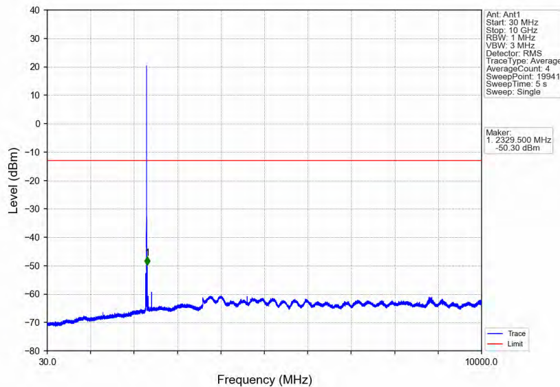
Band40a_5MHz_16QAM_HCH_2312.5MHz_RB_1_0_NTNV
