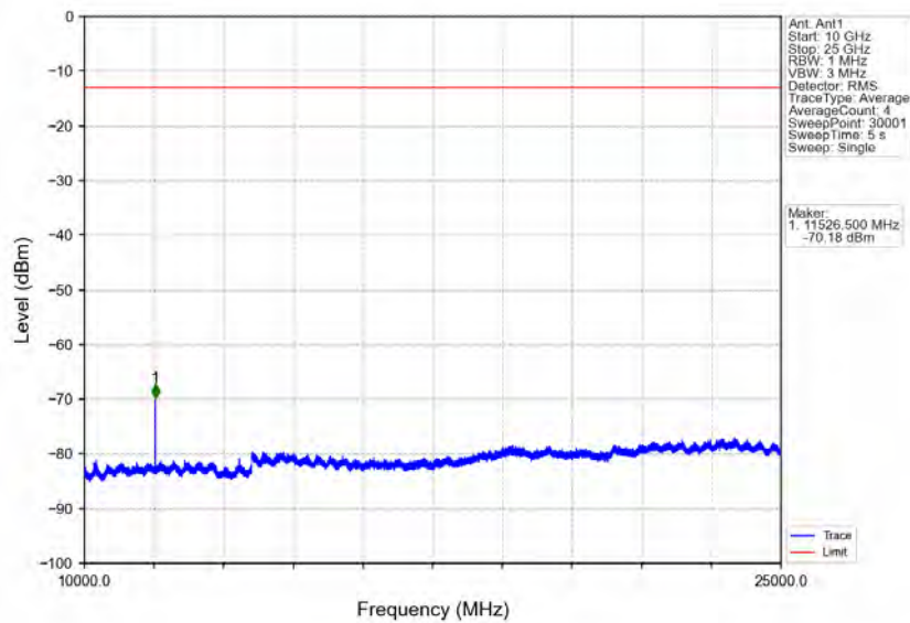
Band40a_5MHz_16QAM_LCH_2307.5MHz_RB_1_0_NTNV
