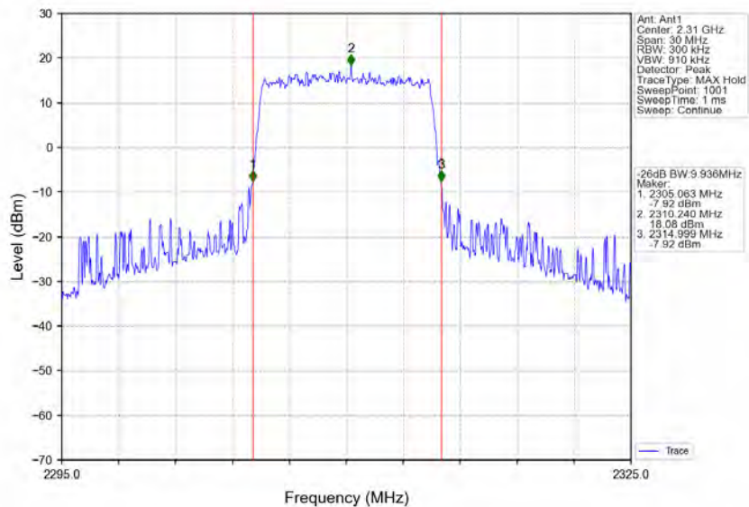
Band40a_10MHz_64QAM_HCH_2310MHz_RB_50_0_NTNV
