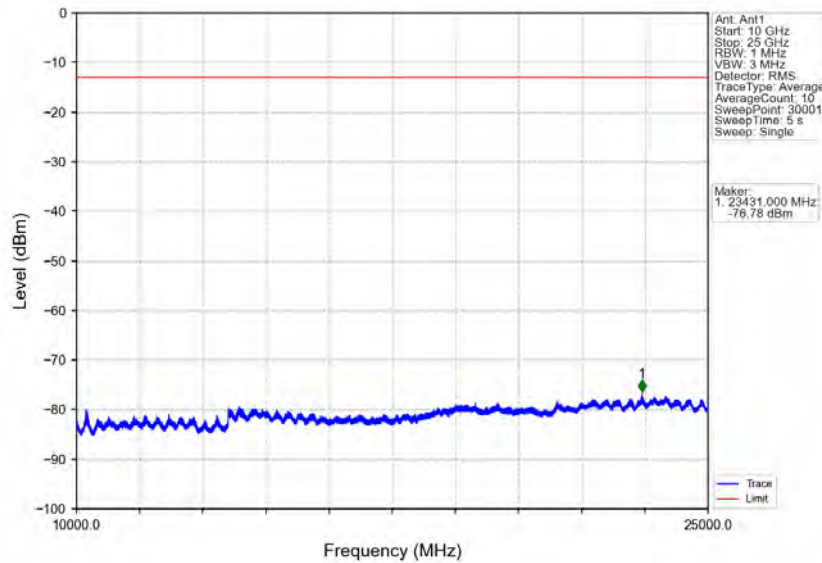
Band40a_5MHz_64QAM_LCH_2307.5MHz_RB_1_0_NTNV
