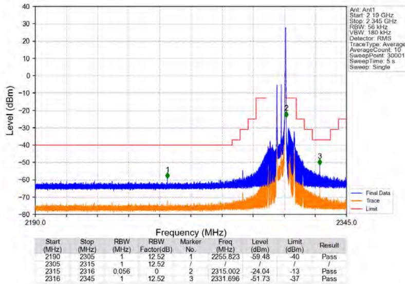
Band40a_5MHz_64QAM_HCH_2312.5MHz_RB_1_24_NTNV
