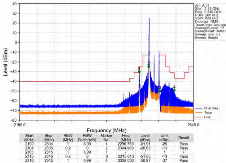
Band40a_10MHz_64QAM_LCH_2310MHz_RB_1_0_NTNV
