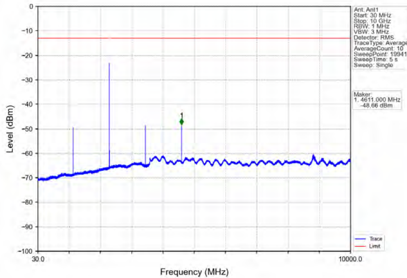
Band40a_10MHz_64QAM_HCH_2310MHz_RB_1_0_NTNV
