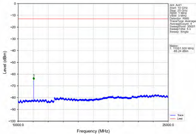
Band40a_5MHz_QPSK_HCH_2312.5MHz_RB_1_0_NTNV
