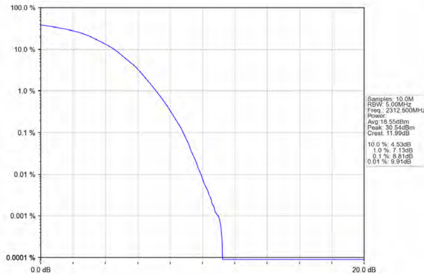
Band40a_5MHz_64QAM_HCH_2312.5MHz_RB_25_0_NTNV
