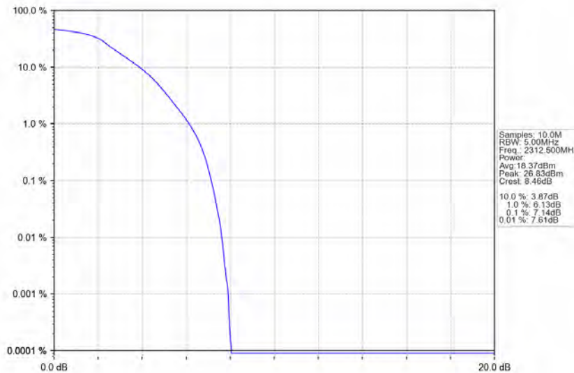
Band40a_5MHz_QPSK_HCH_2312.5MHz_RB_25_0_NTNV
