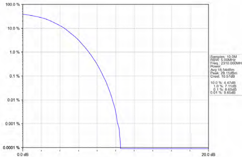
Band40a_5MHz_64QAM_MCH_2310MHz_RB_25_0_NTNV
