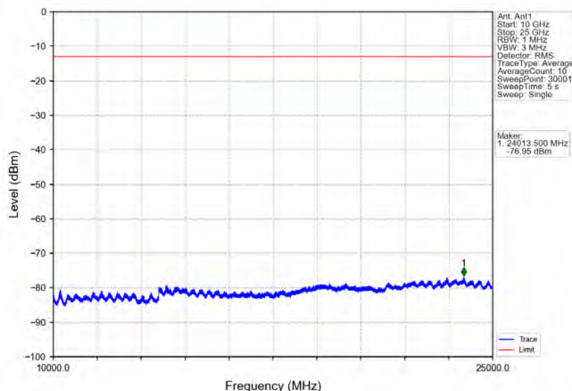
Band40a_5MHz_64QAM_HCH_2312.5MHz_RB_1_0_NTNV
