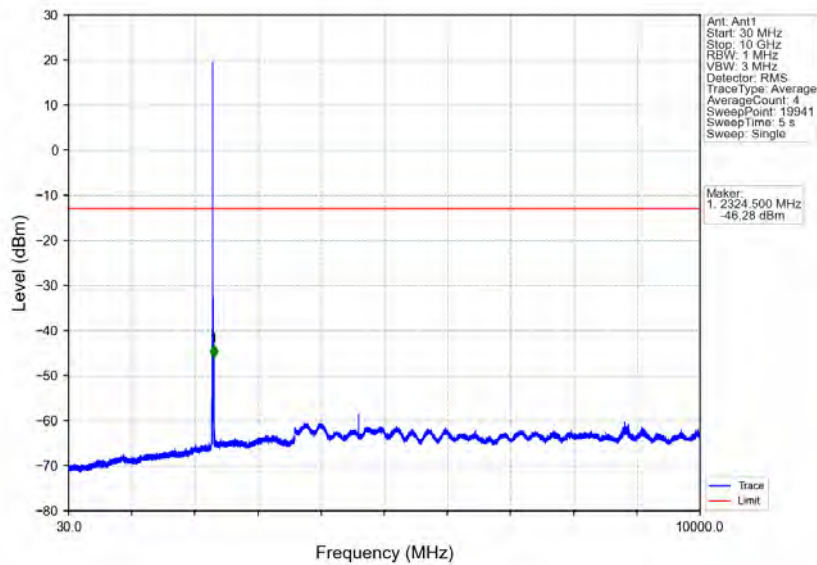
Band40a_5MHz_16QAM_LCH_2307.5MHz_RB_1_0_NTNV
