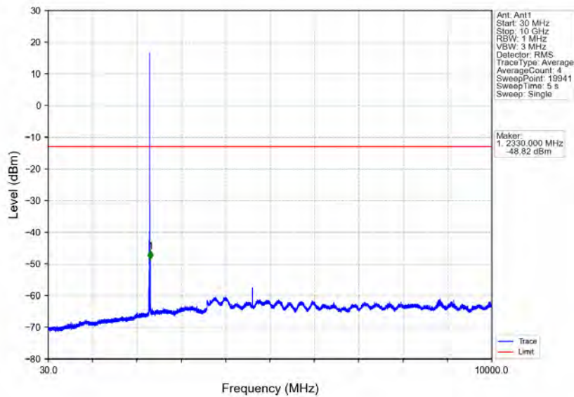
Band40a_5MHz_QPSK_HCH_2312.5MHz_RB_1_0_NTNV
