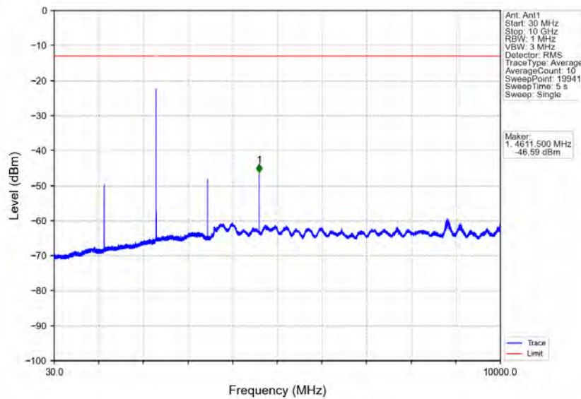
Band40a_10MHz_64QAM_LCH_2310MHz_RB_1_0_NTNV
