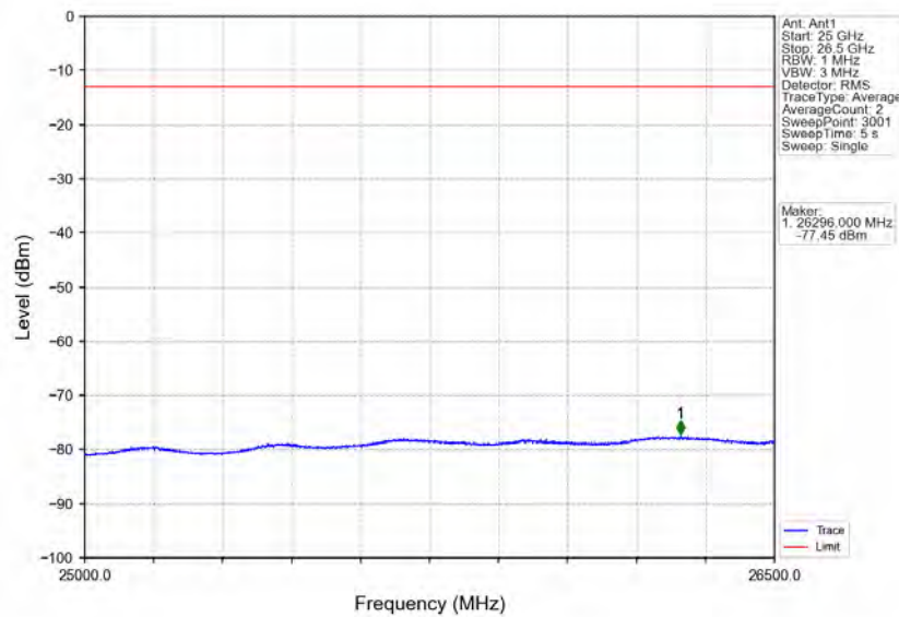
Band40a_5MHz_16QAM_LCH_2307.5MHz_RB_25_0_NTNV
