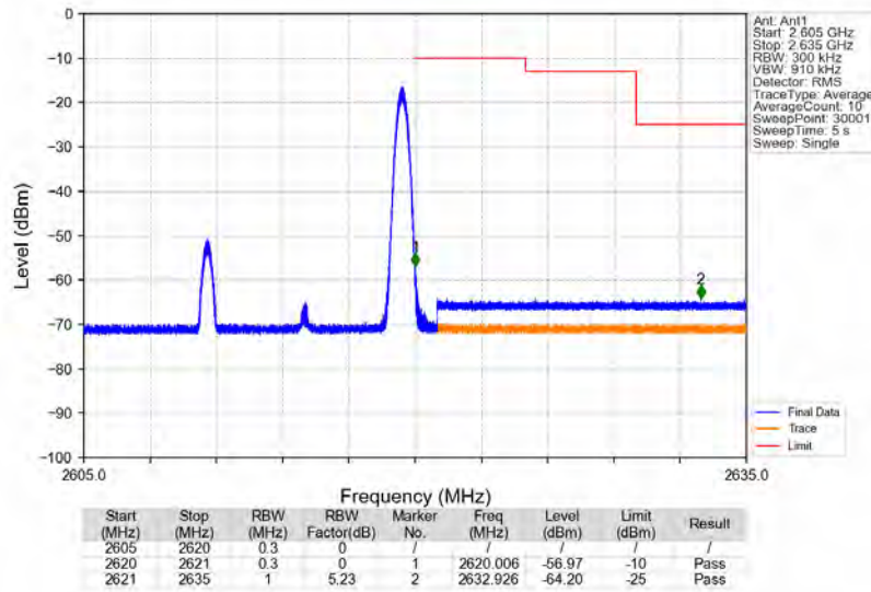
Band38_10MHz_16QAM_HCH_2615MHz_RB_1_49_NTNV
