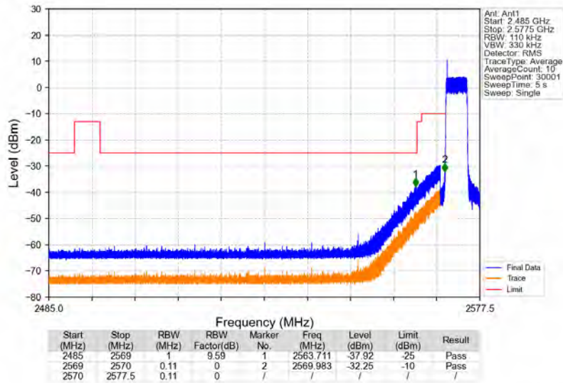
Band38_5MHz_64QAM_LCH_2572.5MHz_RB_25_0_NTNV
