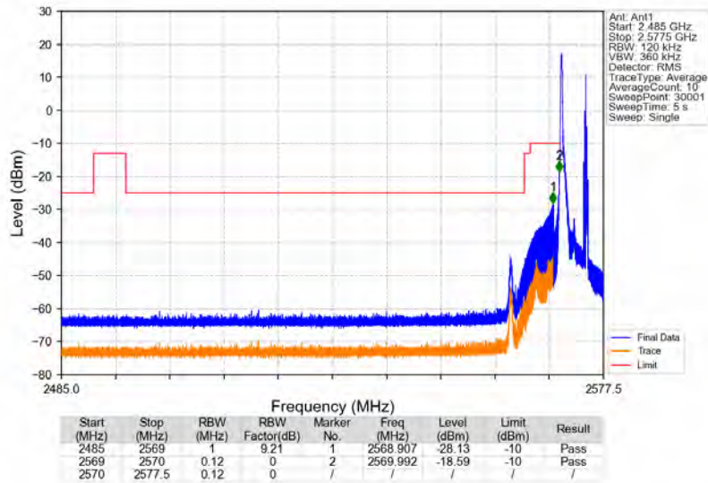
Band38_5MHz_64QAM_LCH_2572.5MHz_RB_1_0_NTV
