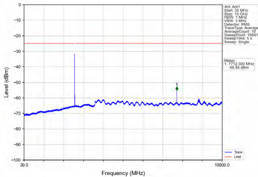
Band38_15MHz_64QAM_LCH_2577.5MHz_RB_1_0_NTNV
