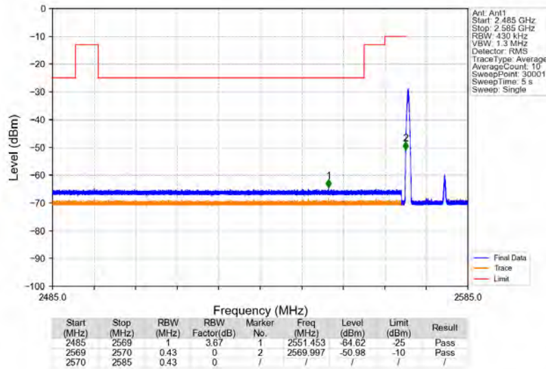
Band38_10MHz_16QAM_LCH_2575MHz_RB_1_0_NTV
