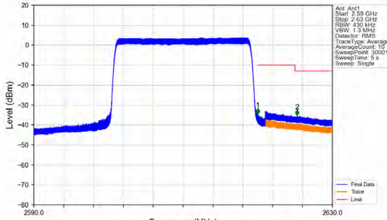
Band38_20MHz_64QAM_HCH_2610MHz_RB_100_0_NTNV
