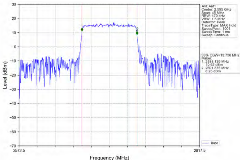
Band38_15MHz_QPSK_MCH_2595MHz_RB_75_0_NTNV
