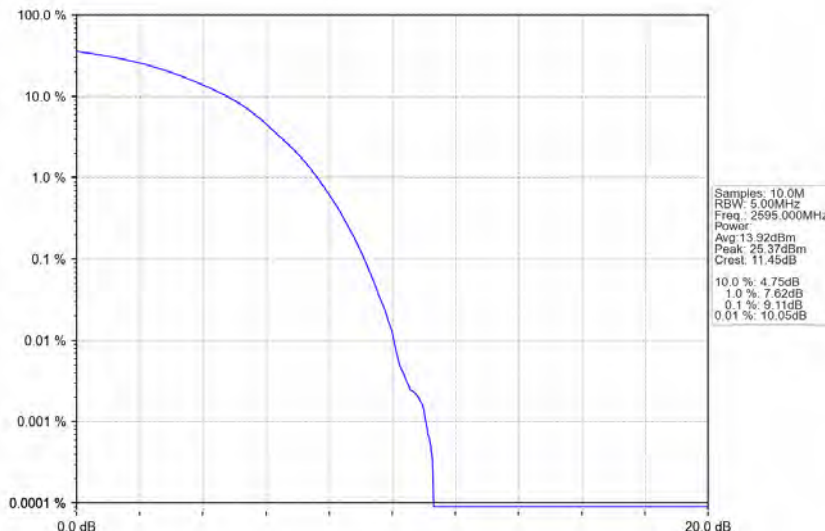
Band38_15MHz_16QAM_MCH_2595MHz_RB_75_0_NTNV
