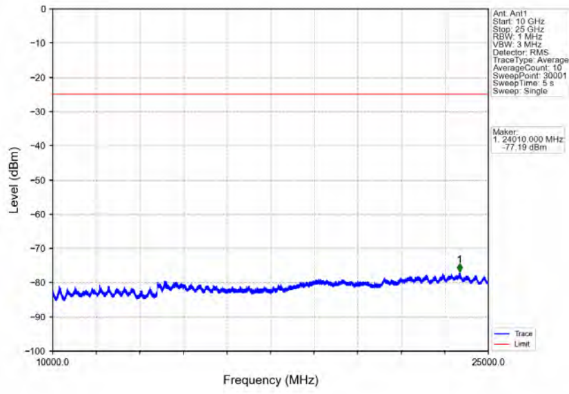
Band38_15MHz_64QAM_HCH_2612.5MHz_RB_1_0_NTNV
