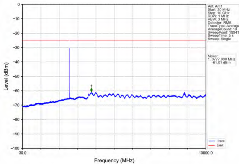
Band38_10MHz_64QAM_LCH_2575MHz_RB_1_0_NTNV
