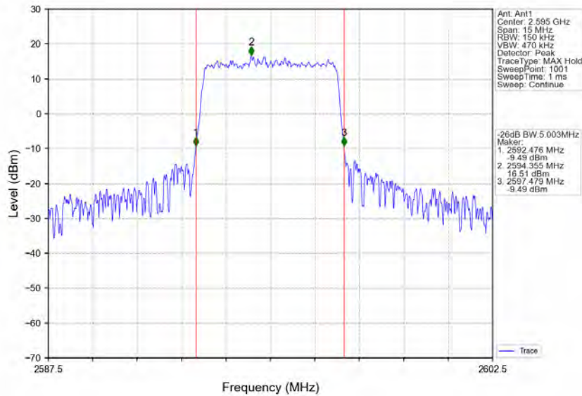
Band38_5MHz_64QAM_MCH_2595MHz_RB_25_0_NTNV
