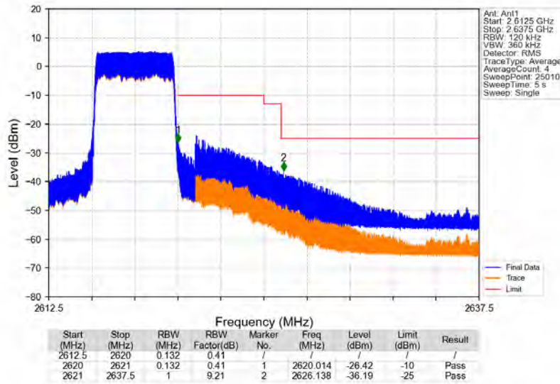
Band38_5MHz_16QAM_HCH_2617.5MHz_RB_25_0_NTNV
