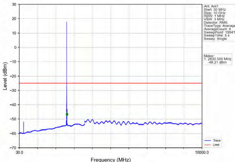
Band38_5MHz_16QAM_HCH_2617.5MHz_RB_1_0_NTNV
