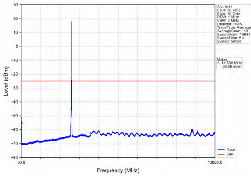
Band38_15MHz_64QAM_HCH_2612.5MHz_RB_1_0_NTNV
