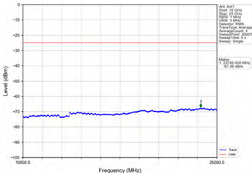
Band38_10MHz_16QAM_HCH_2615MHz_RB_1_0_NTV
