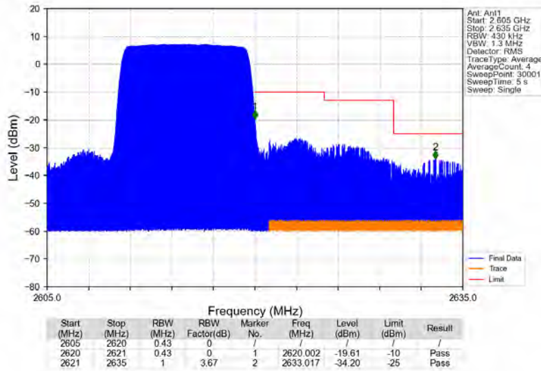
Band38_10MHz_16QAM_HCH_2615MHz_RB_50_0_NTNV
