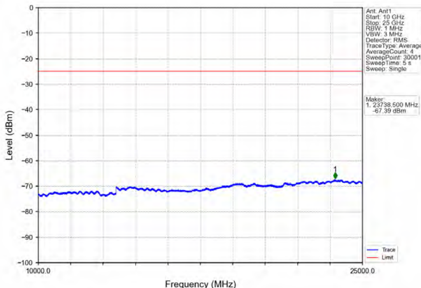
Band38_15MHz_16QAM_MCH_2595MHz_RB_1_0_NTNV
