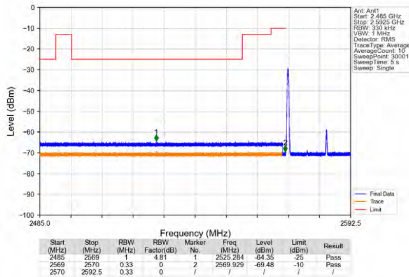
Band38_15MHz_16QAM_LCH_2577.5MHz_RB_1_0_NTNV
