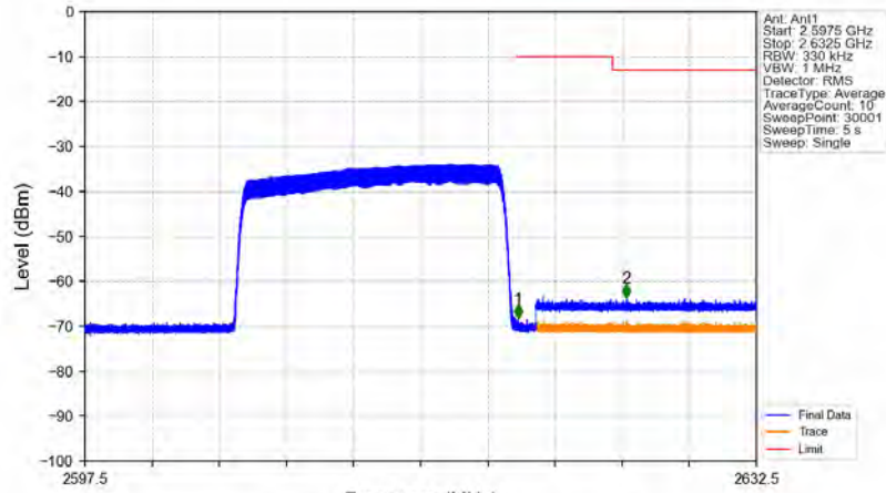
Band38_15MHz_64QAM_HCH_2612.5MHz_RB_75_0_NTNV
