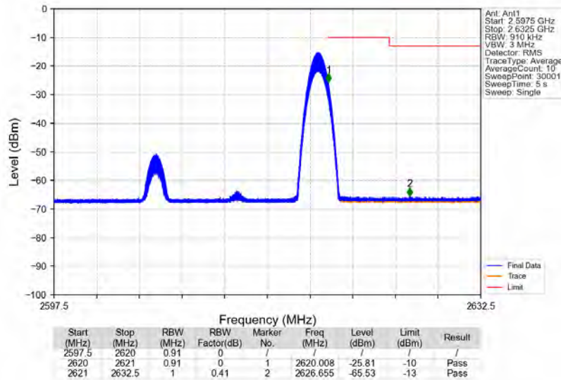
Band38_15MHz_16QAM_HCH_2612.5MHz_RB_1_74_NTNV
