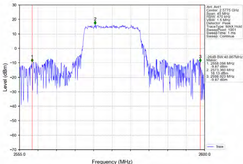
Band38_15MHz_16QAM_LCH_2577.5MHz_RB_75_0_NTNV
