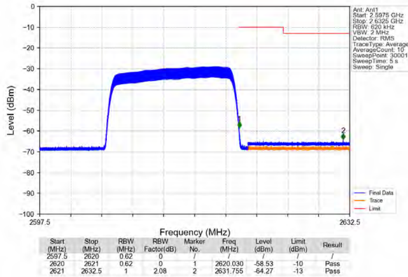
Band38_15MHz_QPSK_HCH_2612.5MHz_RB_75_0_NTNV
