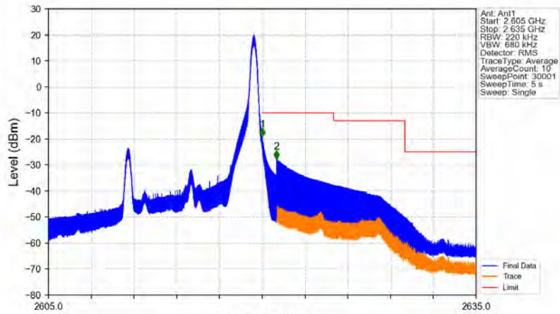
Band38_10MHz_64QAM_HCH_2615MHz_RB_1_49_NTNV
