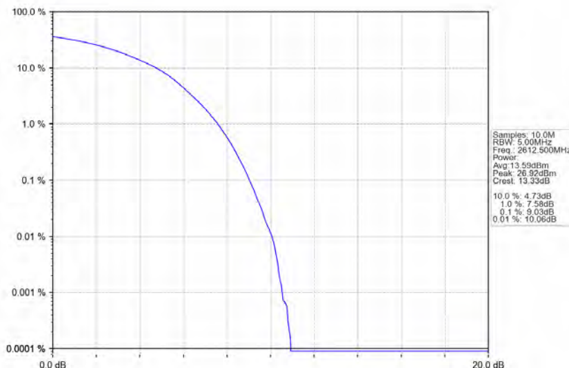
Band38_15MHz_16QAM_HCH_2612.5MHz_RB_75_0_NTNV
