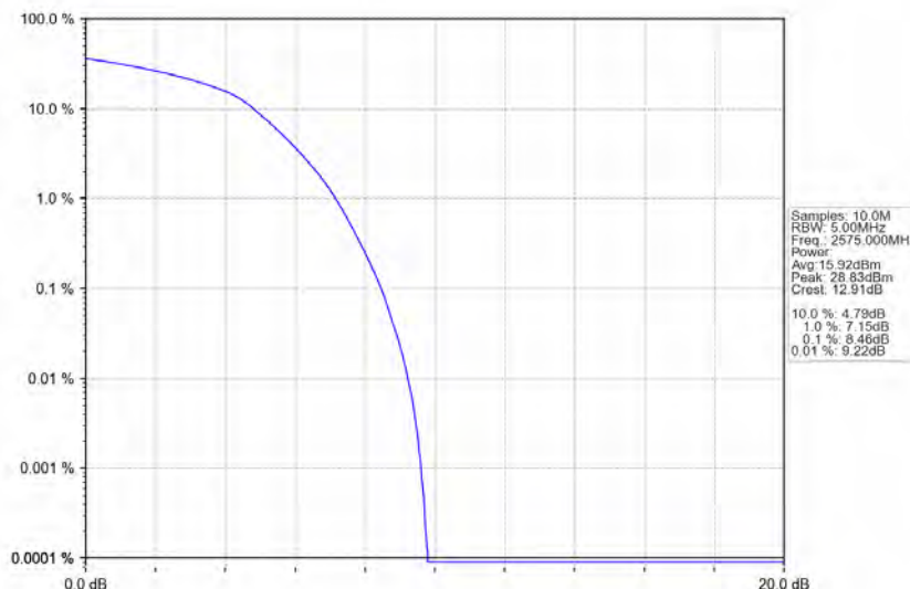
Band38_10MHz_16QAM_LCH_2575MHz_RB_50_0_NTNV
