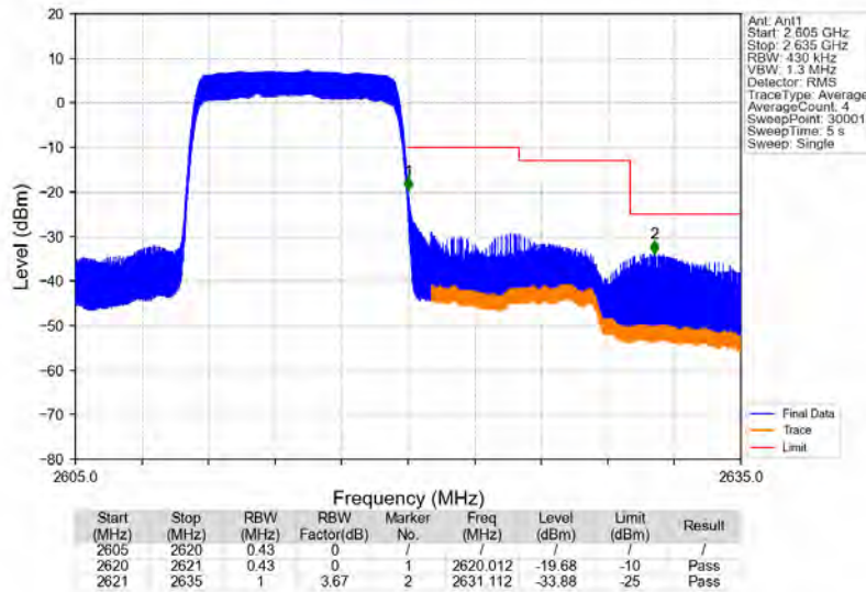
Band38_10MHz_QPSK_HCH_2615MHz_RB_50_0_NTV
