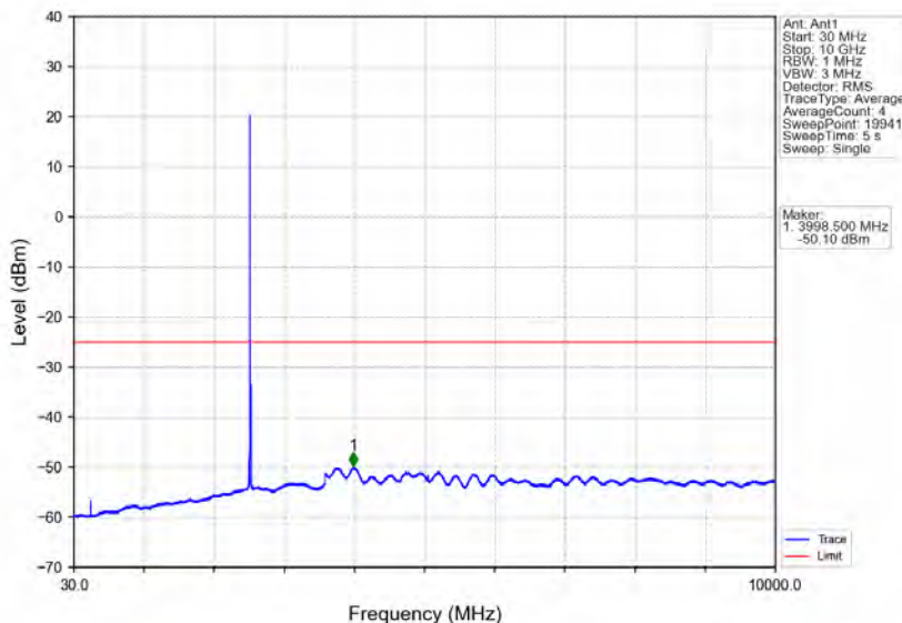
Band7_10MHz_16QAM_MCH_2535MHz_RB_1_0_NTNV
