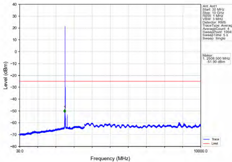
Band7_10MHz_64QAM_MCH_2535MHz_RB_1_0_NTNV
