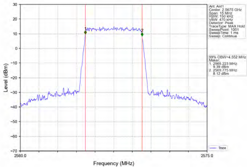
Band7_5MHz_16QAM_HCH_2567.5MHz_RB_25_0_NTNV
