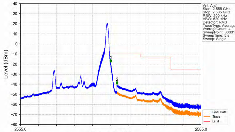
Band7_10MHz_64QAM_HCH_2565MHz_RB_1_49_NTNV
