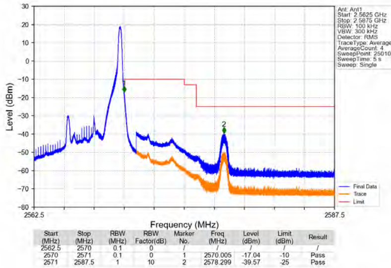
Band7_5MHz_64QAM_HCH_2567.5MHz_RB_1_24_NTNV
