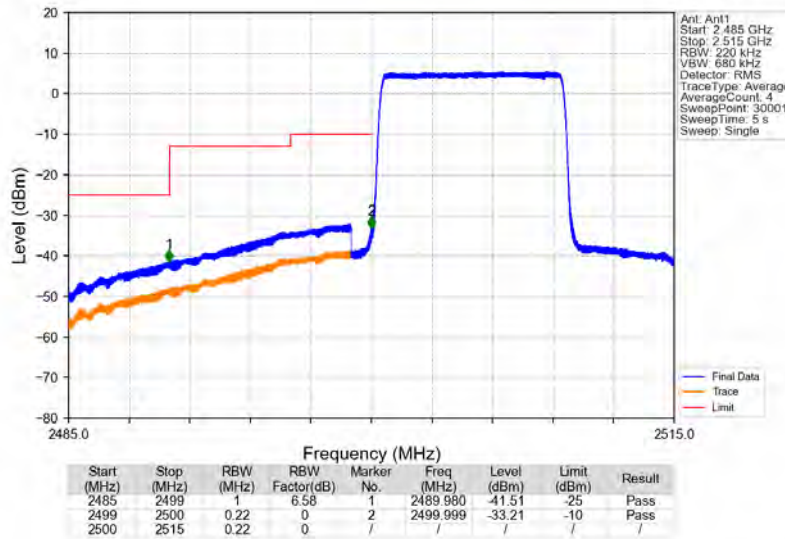
Band7_10MHz_64QAM_LCH_2505MHz_RB_50_0_NTNV
