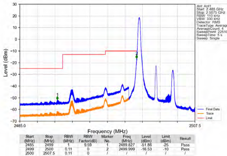
Band7_5MHz_16QAM_LCH_2502.5MHz_RB_1_0_NTNV
