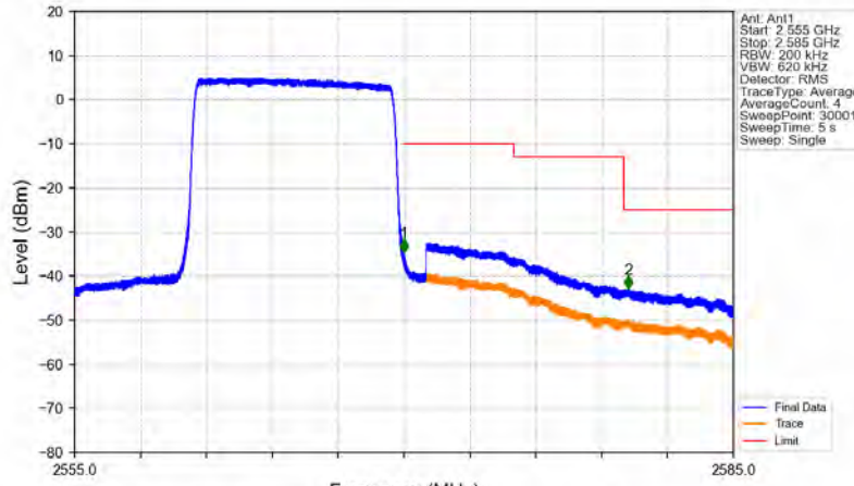
Band7_10MHz_64QAM_HCH_2565MHz_RB_50_0_NTV
