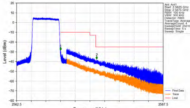
Band7_5MHz_64QAM_HCH_2567.5MHz_RB_25_0_NTNV
