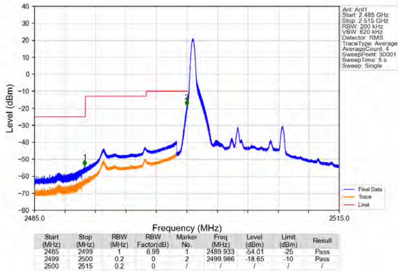
Band7_10MHz_64QAM_LCH_2505MHz_RB_1_0_NTNV
