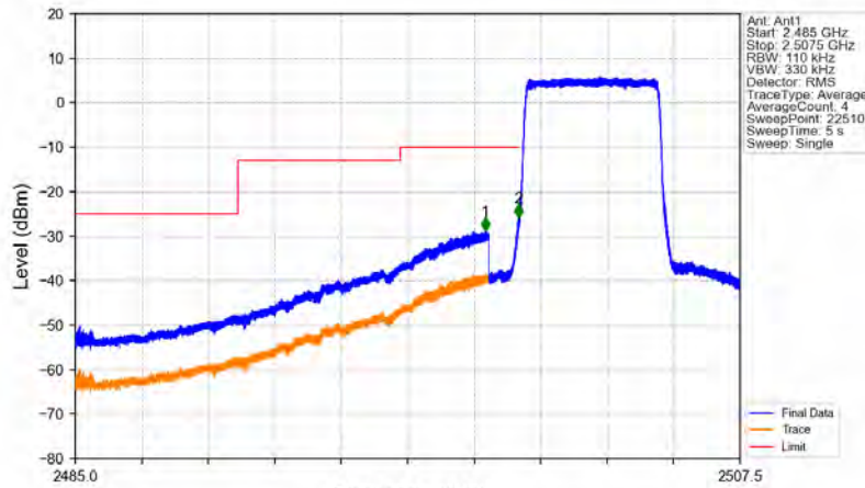
Band7_5MHz_16QAM_LCH_2502.5MHz_RB_25_0_NTNV
