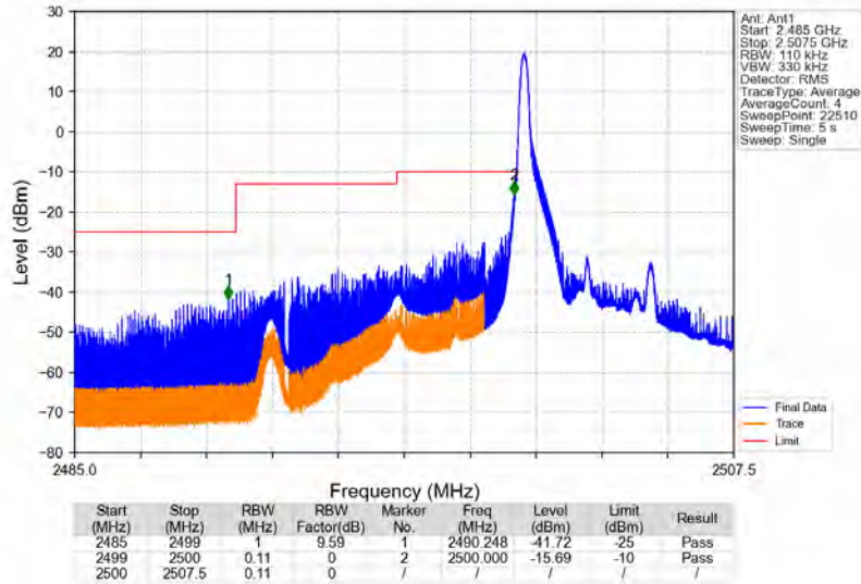
Band7_5MHz_64QAM_LCH_2502.5MHz_RB_1_0_NTNV
