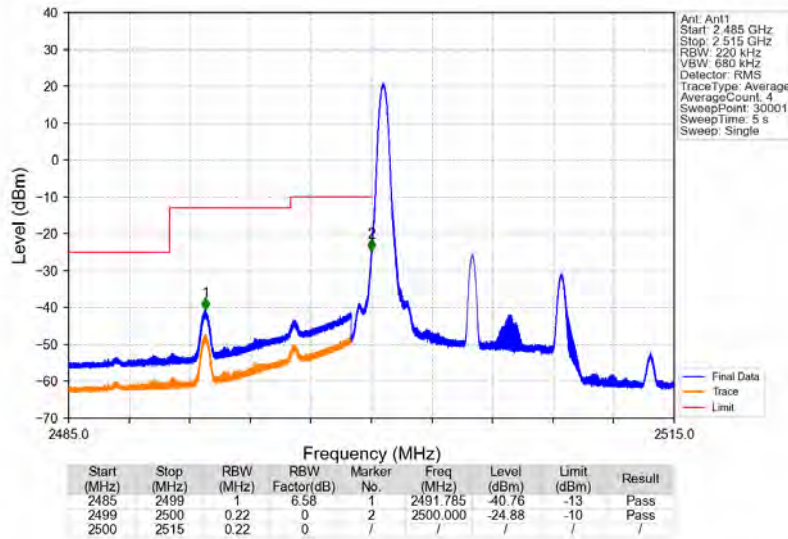
Band7_10MHz_16QAM_LCH_2505MHz_RB_1_0_NTNV
