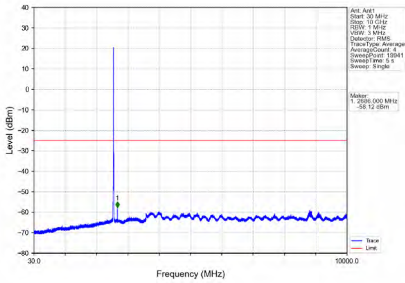
Band7_10MHz_64QAM_HCH_2565MHz_RB_1_0_NTNV
