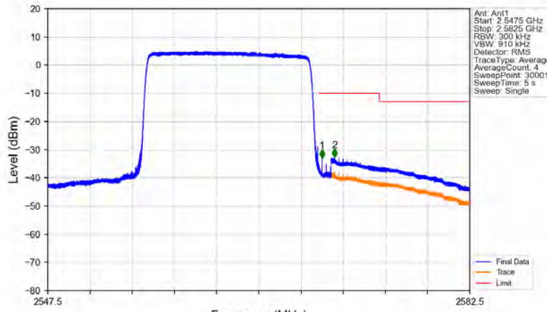
Band7_15MHz_64QAM_HCH_2562.5MHz_RB_75_0_NTNV
