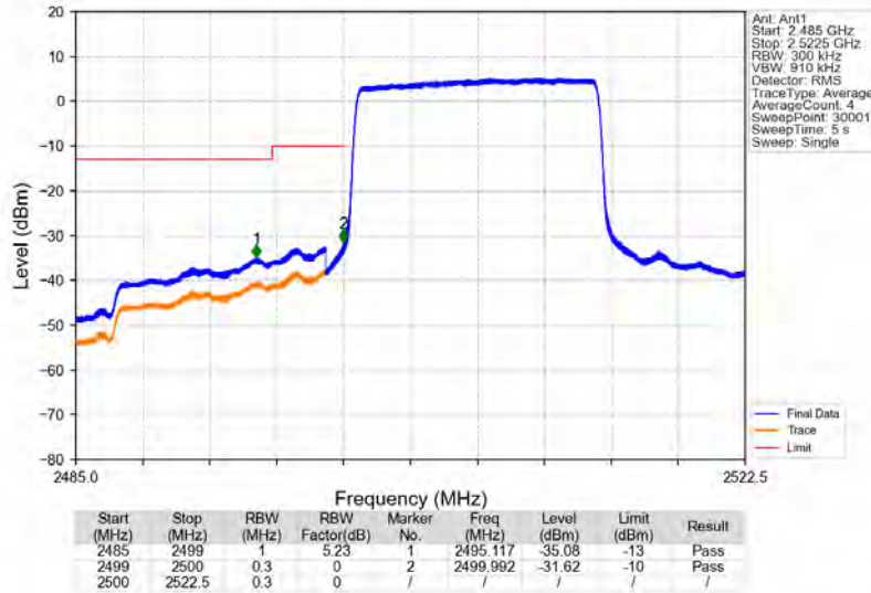
Band7_15MHz_QPSK_LCH_2507.5MHz_RB_75_0_NTNV
