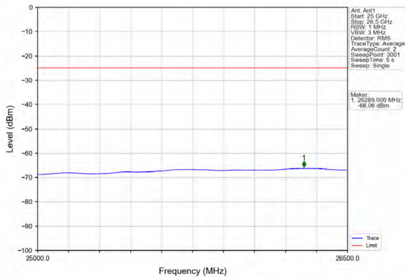
Band7_10MHz_16QAM_LCH_2505MHz_RB_50_0_NTV
