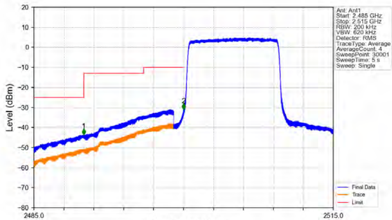
Band7_10MHz_16QAM_LCH_2505MHz_RB_50_0_NTV
