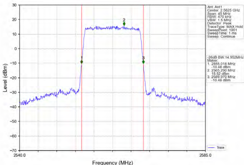
Band7_15MHz_16QAM_HCH_2562.5MHz_RB_75_0_NTNV
