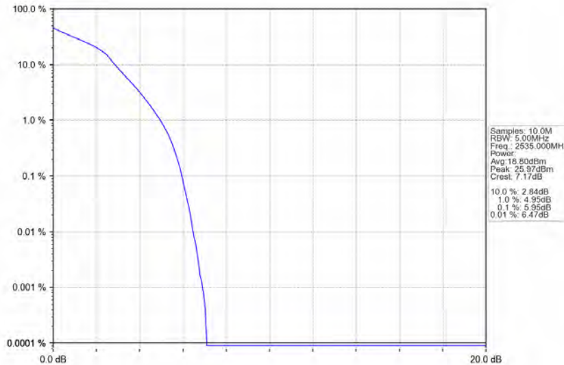
Band7_5MHz_16QAM_MCH_2535MHz_RB_25_0_NTNV
