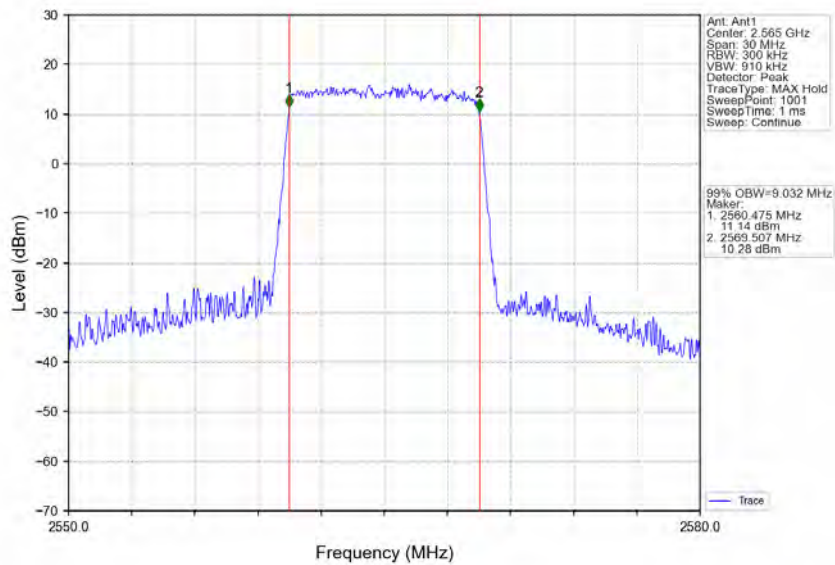
Band7_10MHz_64QAM_HCH_2565MHz_RB_50_0_NTNV
