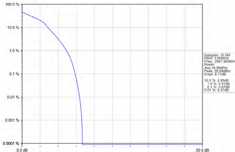
Band7_5MHz_16QAM_HCH_2567.5MHz_RB_25_0_NTNV
