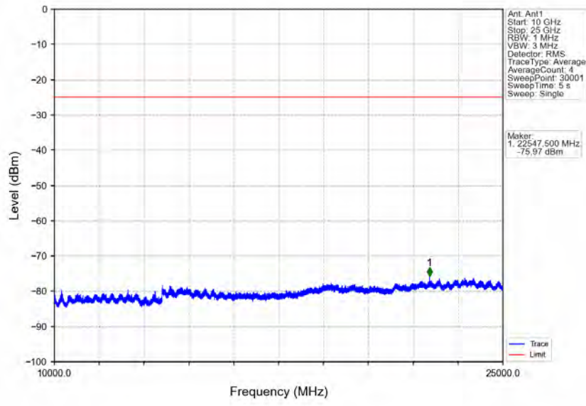
Band7_10MHz_64QAM_HCH_2565MHz_RB_1_0_NTNV
