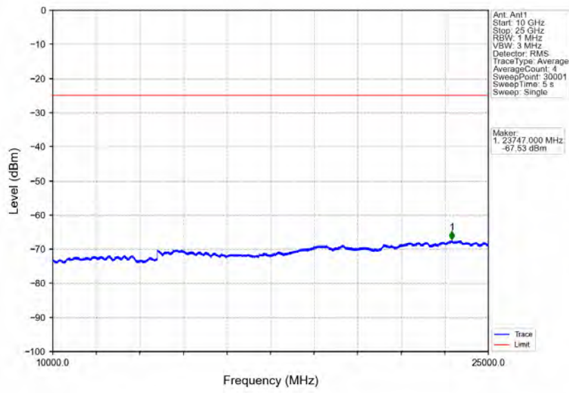
Band7_5MHz_16QAM_HCH_2567.5MHz_RB_1_0_NTNV
