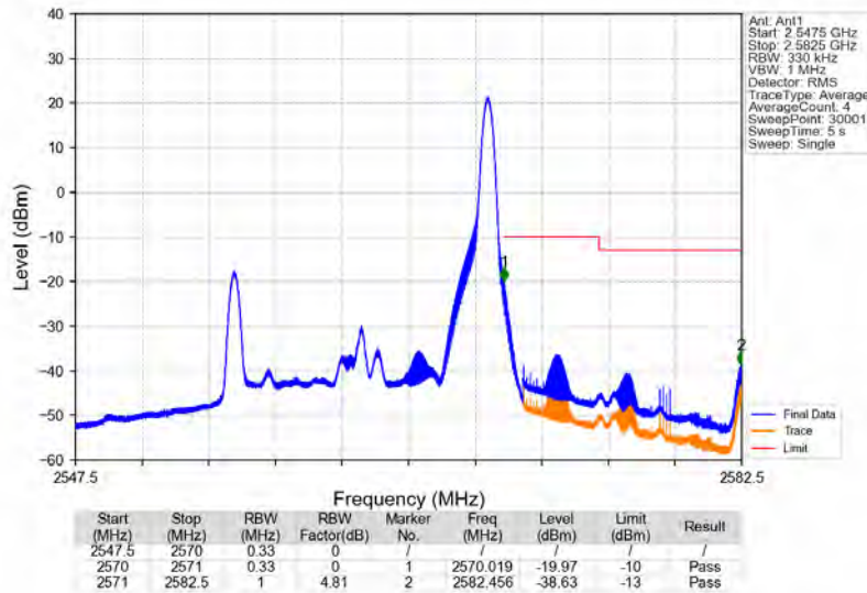
Band7_15MHz_64QAM_HCH_2562.5MHz_RB_1_74_NTNV
