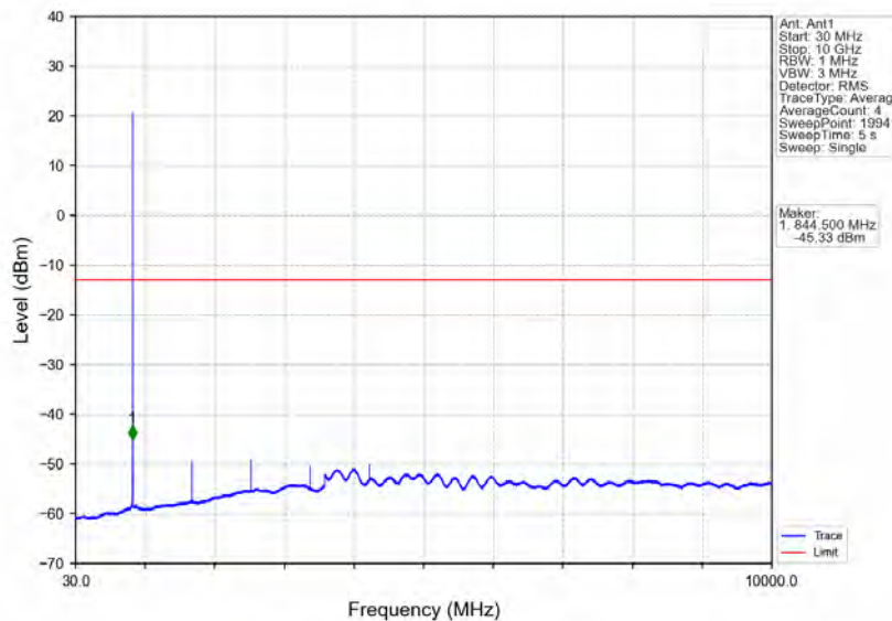
Band5_1.4MHz_16QAM_HCH_848.3MHz_RB_1_0_NTNV
