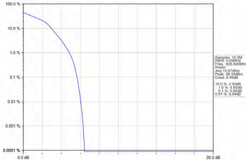
Band5_3MHz_16QAM_LCH_825.5MHz_RB_15_0_NTNV
