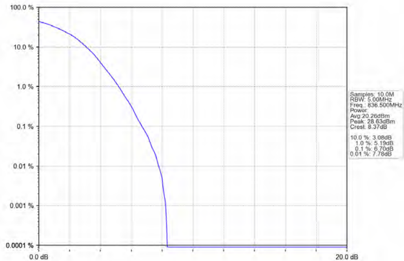
Band5_1.4MHz_64QAM_MCH_836.5MHz_RB_6_0_NTNV
