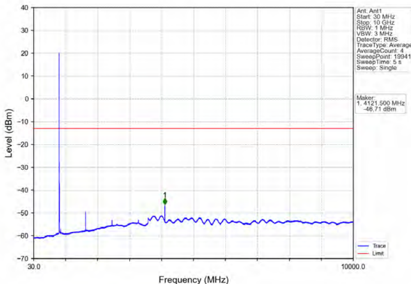
Band5_5MHz_16QAM_LCH_826.5MHz_RB_25_0_NTNV
