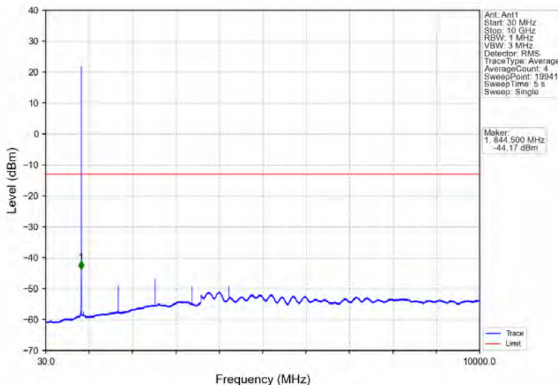
Band5_1.4MHz_QPSK_HCH_848.3MHz_RB_1_5_NTNV
