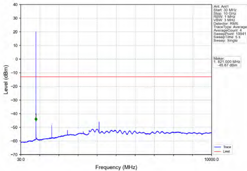
Band5_1.4MHz_16QAM_LCH_824.7MHz_RB_6_0_NTNV
