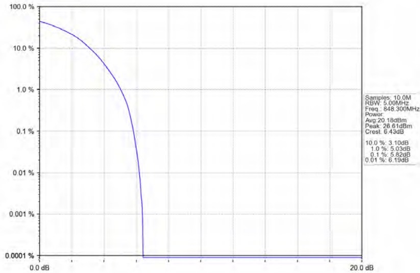
Band5_1.4MHz_64QAM_HCH_848.3MHz_RB_6_0_NTV
