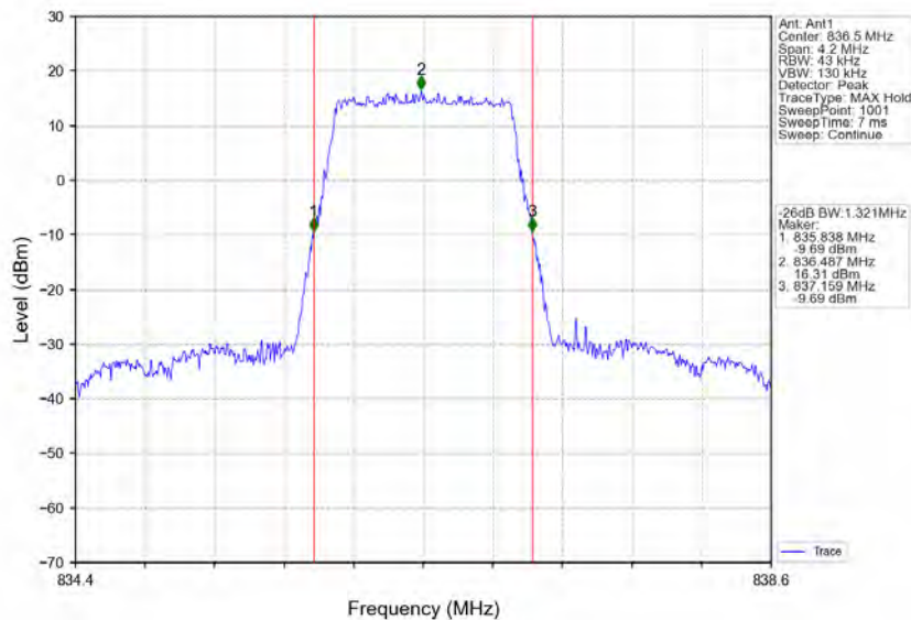
Band5_1.4MHz_64QAM_MCH_836.5MHz_RB_6_0_NTNV
