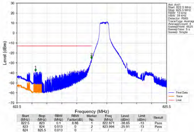
Band5_1.4MHz_64QAM_LCH_824.7MHz_RB_1_0_NTNV
