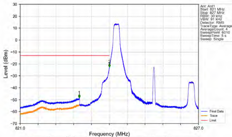
Band5_3MHz_16QAM_LCH_825.5MHz_RB_1_0_NTNV
