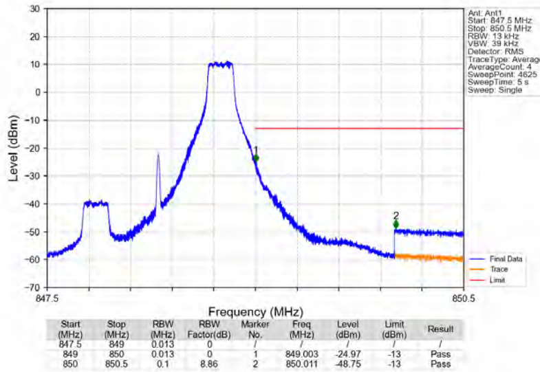
Band5_1.4MHz_16QAM_HCH_848.3MHz_RB_1_5_NTV
