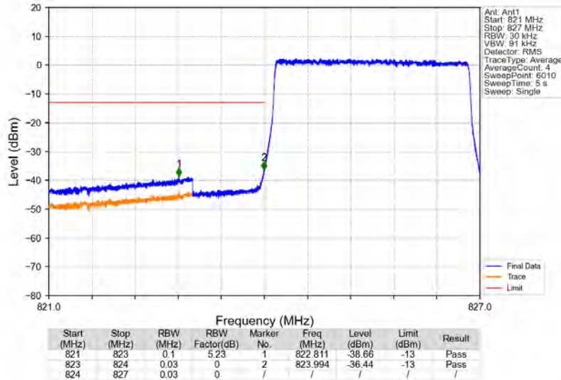
Band5_3MHz_64QAM_LCH_825.5MHz_RB_15_0_NTNV
