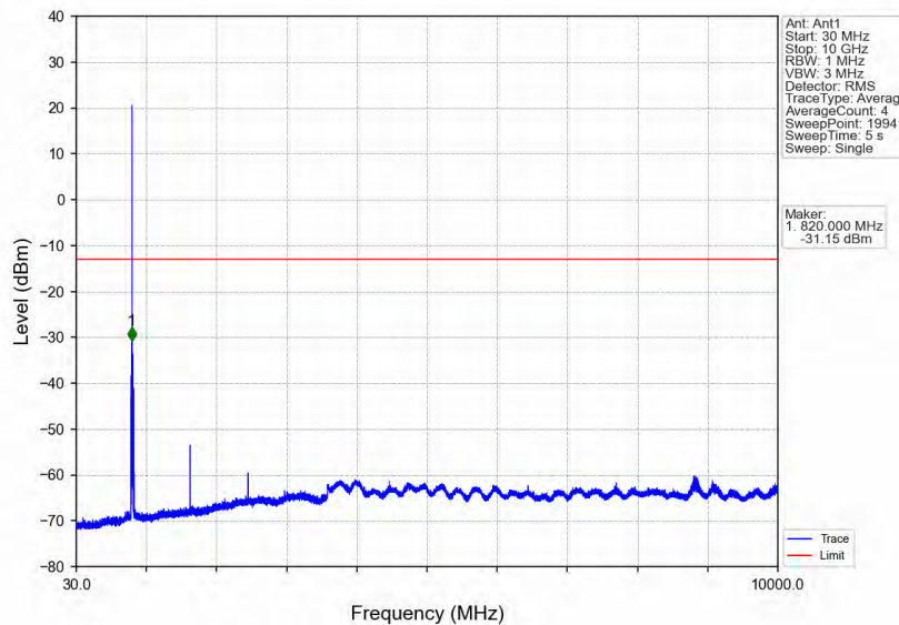
Band5_1.4MHz_64QAM_LCH_824.7MHz_RB_1_0_NTNV
