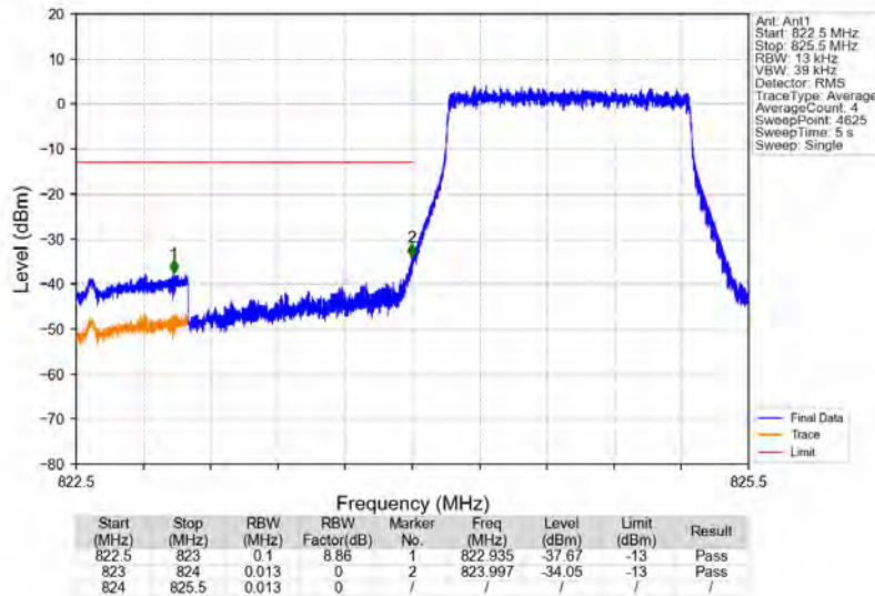
Band5_1.4MHz_64QAM_LCH_824.7MHz_RB_6_0_NTV
