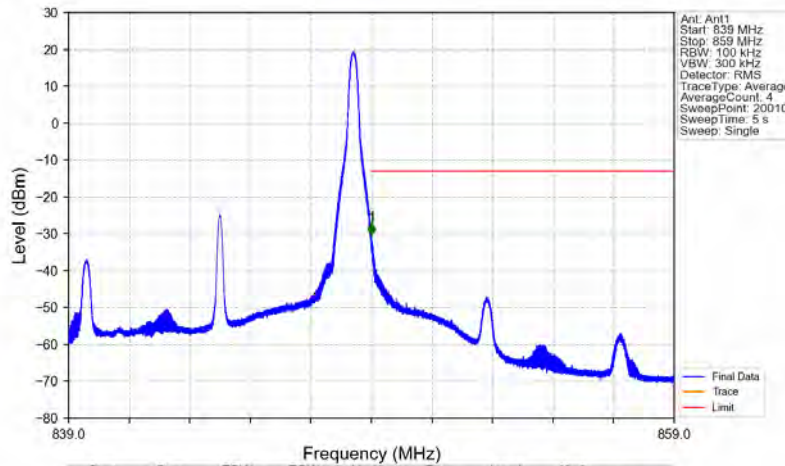
Band5_10MHz_16QAM_HCH_844MHz_RB_1_49_NTNV
