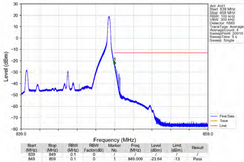
Band5_10MHz_64QAM_HCH_844MHz_RB_1_49_NTNV
