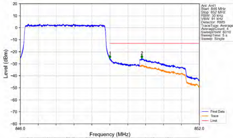
Band5_3MHz_QPSK_HCH_847.5MHz_RB_15_0_NTNV
