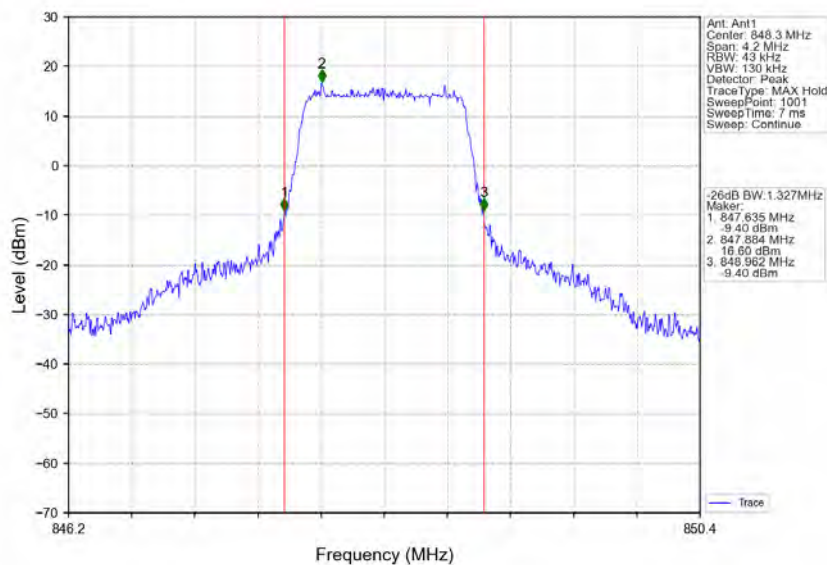
Band5_1.4MHz_16QAM_HCH_848.3MHz_RB_6_0_NTNV
