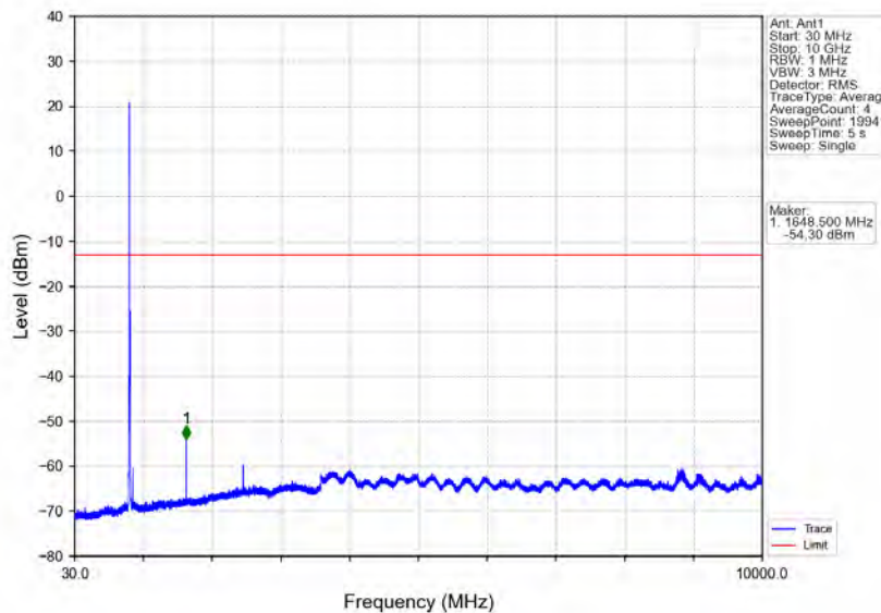
Band5_5MHz_64QAM_LCH_826.5MHz_RB_1_0_NTNV
