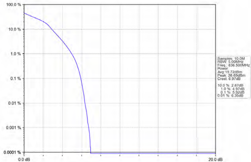
Band5_5MHz_16QAM_MCH_836.5MHz_RB_25_0_NTNV
