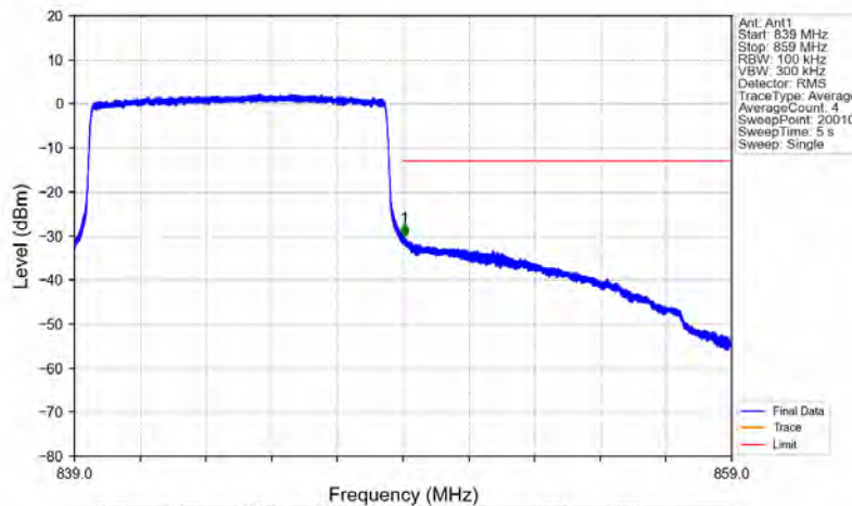
Band5_10MHz_16QAM_HCH_844MHz_RB_50_0_NTNV
