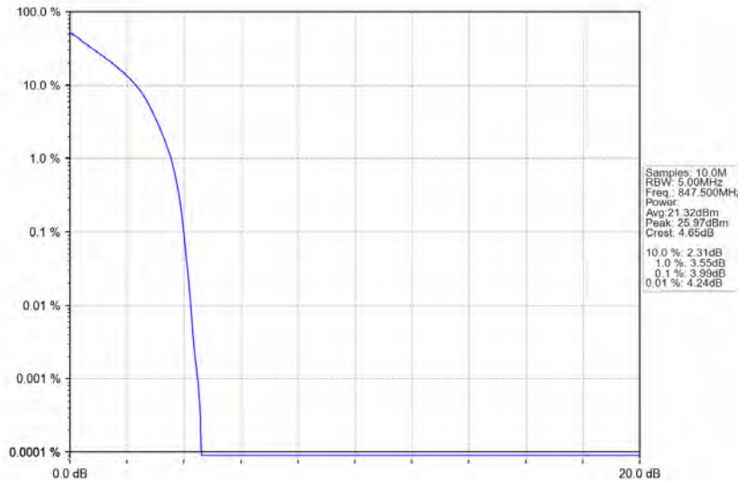
Band5_3MHz_QPSK_HCH_847.5MHz_RB_15_0_NTNV
