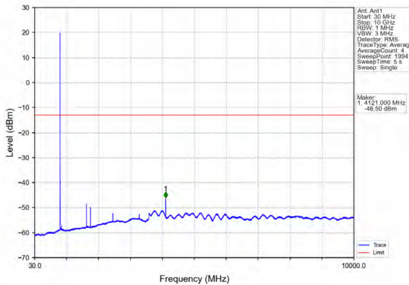
Band5_3MHz_16QAM_LCH_825.5MHz_RB_15_0_NTNV
