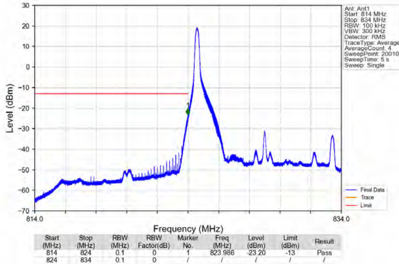
Band5_10MHz_64QAM_LCH_829MHz_RB_1_0_NTNV
