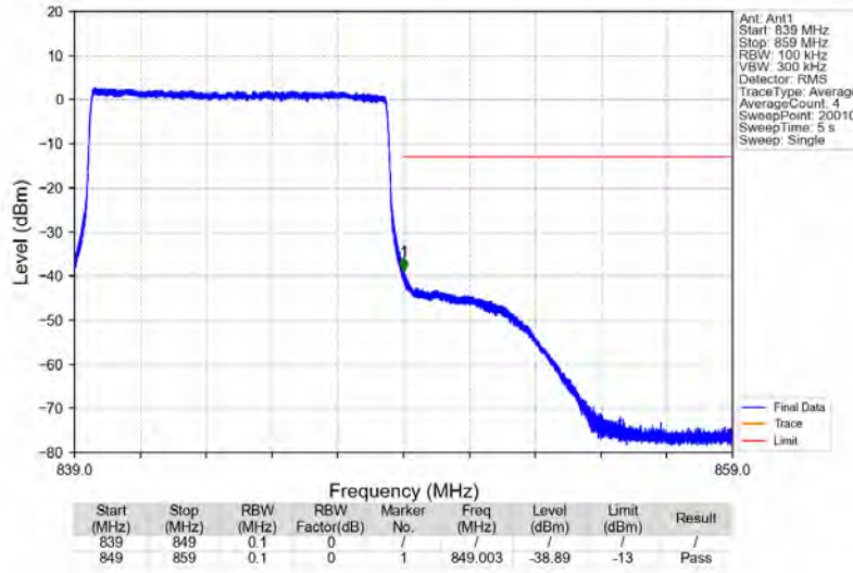
Band5_10MHz_64QAM_HCH_844MHz_RB_50_0_NTNV
