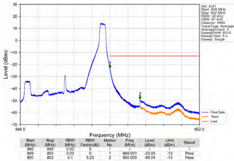
Band5_3MHz_64QAM_HCH_847.5MHz_RB_1_14_NTNV
