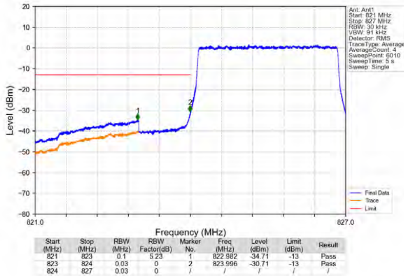
Band5_3MHz_16QAM_LCH_825.5MHz_RB_15_0_NTNV
