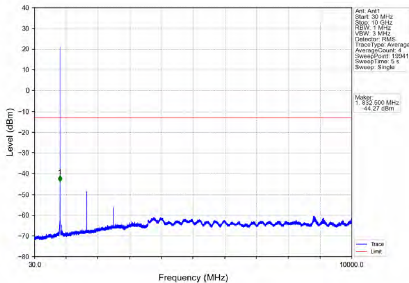
Band5_1.4MHz_64QAM_MCH_836.5MHz_RB_1_0_NTV
