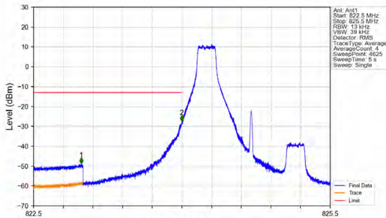
Band5_1.4MHz_16QAM_LCH_824.7MHz_RB_1_0_NTNV
