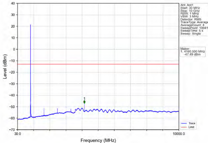
Band5_10MHz_QPSK_MCH_836.5MHz_RB_1_0_NTNV
