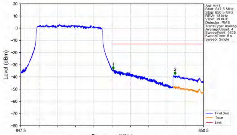
Band5_1.4MHz_64QAM_HCH_848.3MHz_RB_6_0_NTV
