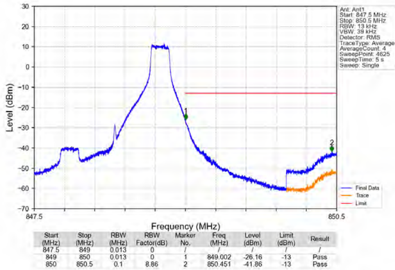
Band5_1.4MHz_64QAM_HCH_848.3MHz_RB_1_5_NTV
