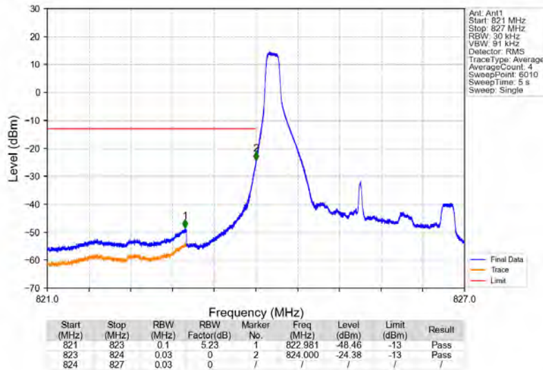
Band5_3MHz_64QAM_LCH_825.5MHz_RB_1_0_NTNV
