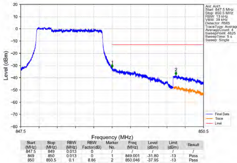
Band5_1.4MHz_16QAM_HCH_848.3MHz_RB_6_0_NTV
