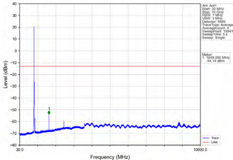
Band5_10MHz_64QAM_LCH_829MHz_RB_1_0_NTNV
