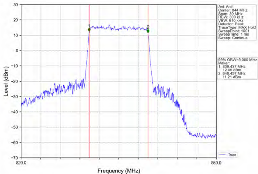
Band5_10MHz_64QAM_HCH_844MHz_RB_50_0_NTNV
