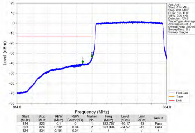
Band5_10MHz_16QAM_LCH_829MHz_RB_50_0_NTNV
