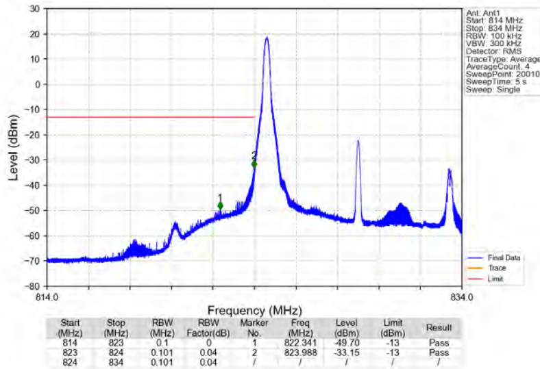
Band5_10MHz_16QAM_LCH_829MHz_RB_1_0_NTNV
