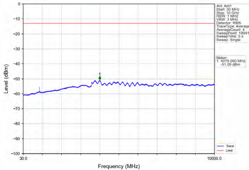
Band5_1.4MHz_QPSK_MCH_836.5MHz_RB_1_0_NTNV
