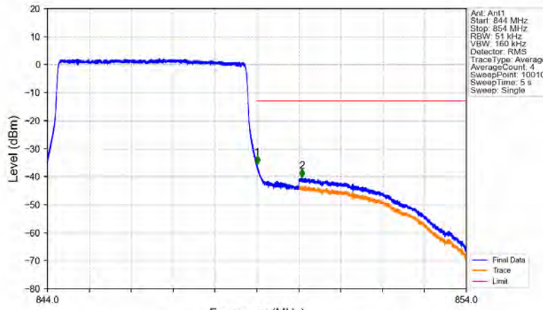
Band5_5MHz_64QAM_HCH_846.5MHz_RB_25_0_NTNV
