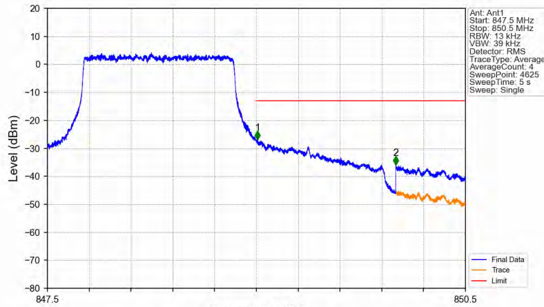
Band5_1.4MHz_QPSK_HCH_848.3MHz_RB_6_0_NTNV
