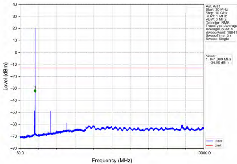
Band5_1.4MHz_64QAM_HCH_848.3MHz_RB_1_5_NTV
