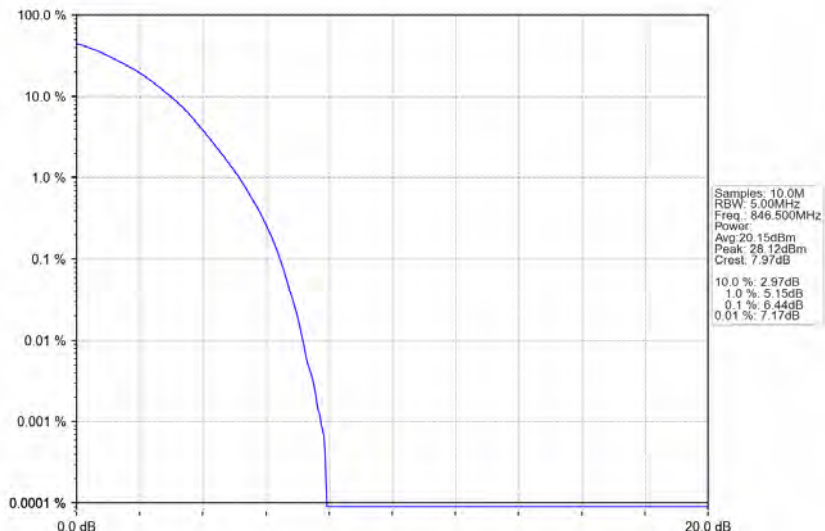
Band5_5MHz_64QAM_HCH_846.5MHz_RB_25_0_NTNV
