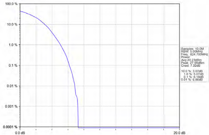
Band5_1.4MHz_64QAM_LCH_824.7MHz_RB_6_0_NTNV
