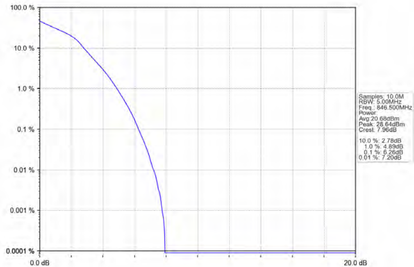
Band5_5MHz_16QAM_HCH_846.5MHz_RB_25_0_NTNV
