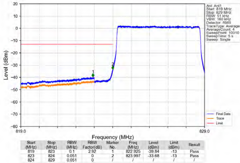
Band5_5MHz_64QAM_LCH_826.5MHz_RB_25_0_NTNV
