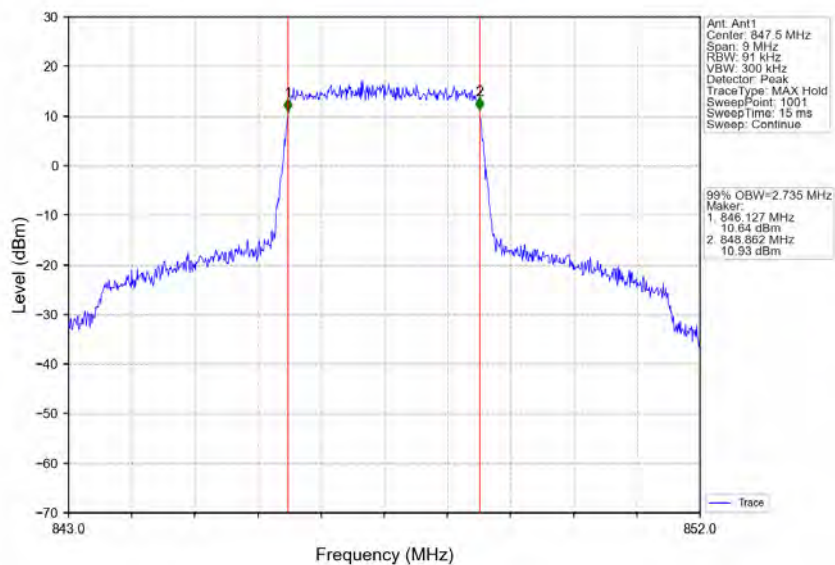
Band5_3MHz_QPSK_HCH_847.5MHz_RB_15_0_NTNV
