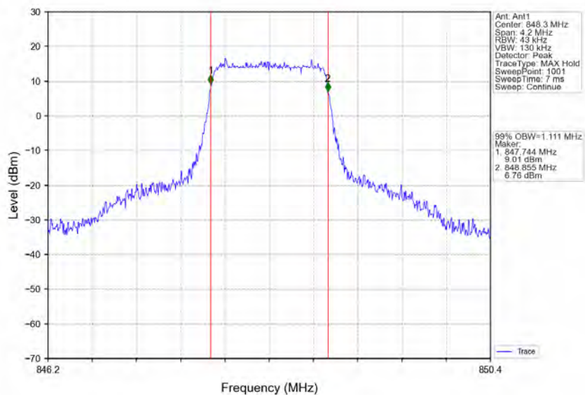
Band5_1.4MHz_16QAM_HCH_848.3MHz_RB_6_0_NTNV
