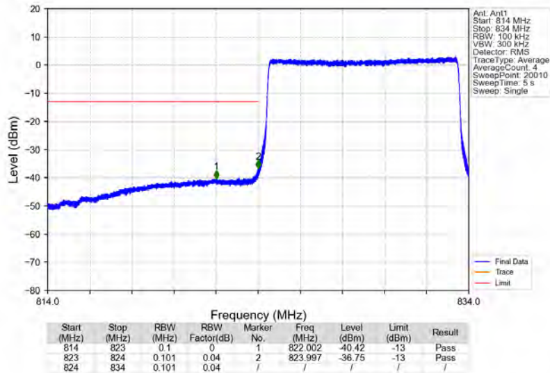
Band5_10MHz_64QAM_LCH_829MHz_RB_50_0_NTNV
