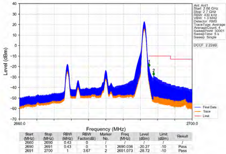
Band41_20MHz_64QAM_HCH_2680MHz_RB_1_99_NTV
