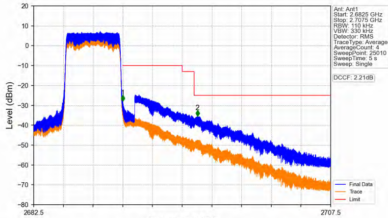
Band41_5MHz_64QAM_HCH_2687.5MHz_RB_25_0_NTNV
