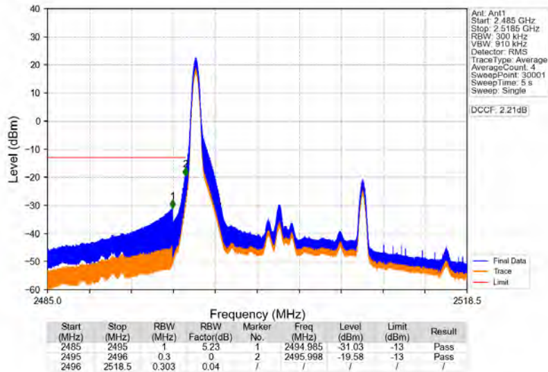
Band41_15MHz_64QAM_LCH_2503.5MHz_RB_1_0_NTNV
