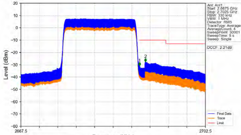
Band41_15MHz_64QAM_HCH_2682.5MHz_RB_75_0_NTNV
