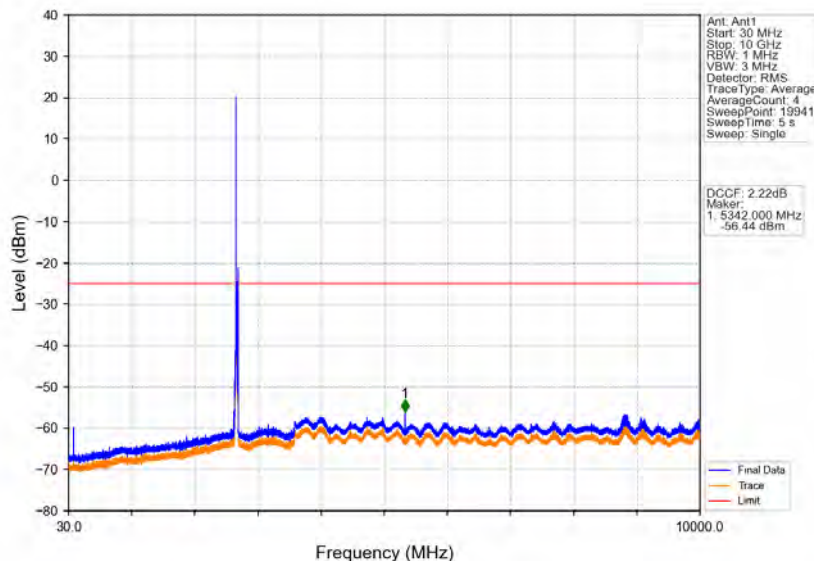
Band41_20MHz_64QAM_HCH_2680MHz_RB_1_0_NTV
