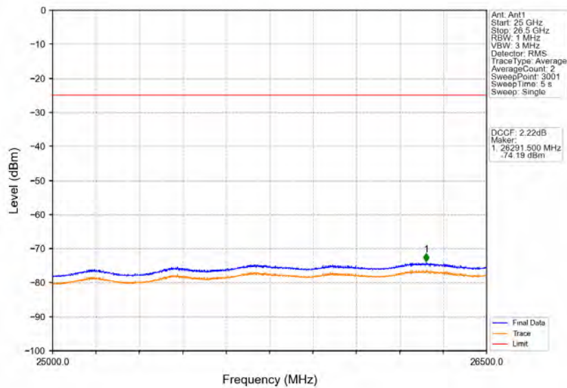
Band41_20MHz_64QAM_HCH_2680MHz_RB_1_99_NTV
