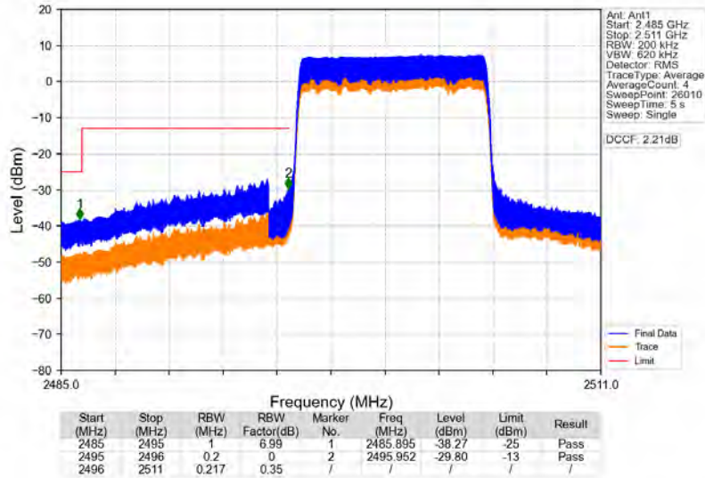
Band41_10MHz_64QAM_LCH_2501MHz_RB_50_0_NTNV
