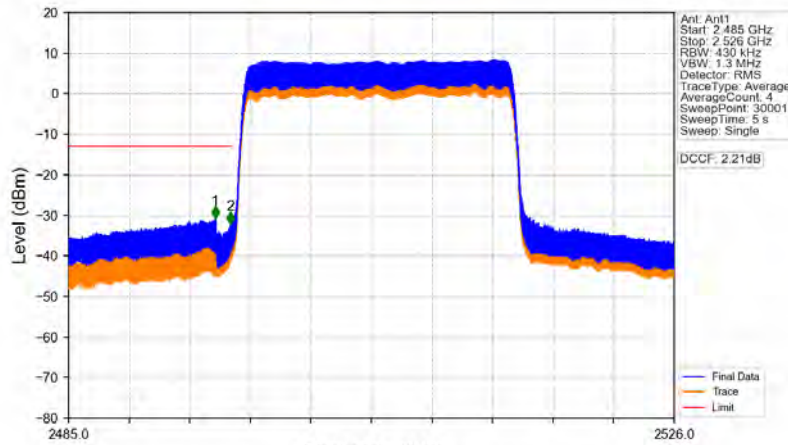
Band41_20MHz_16QAM_LCH_2506MHz_RB_100_0_NTNV
