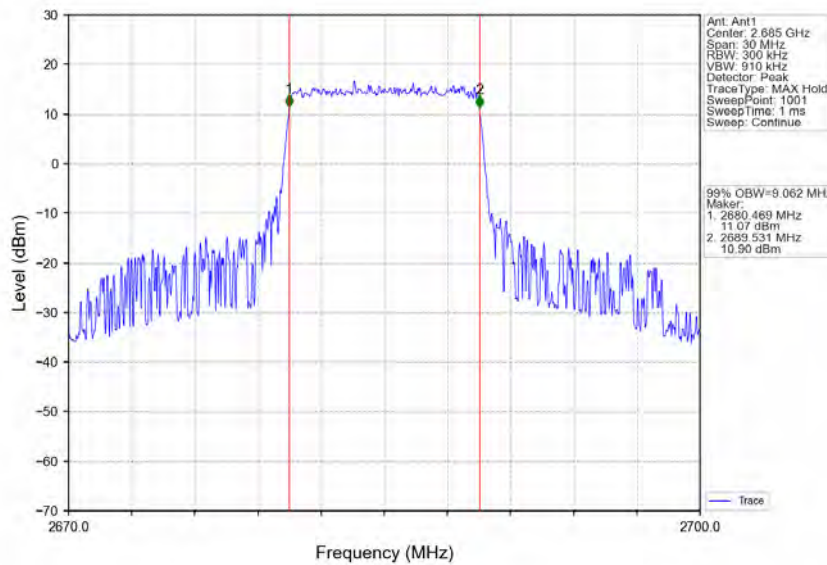
Band41_10MHz_64QAM_HCH_2685MHz_RB_50_0_NTNV
