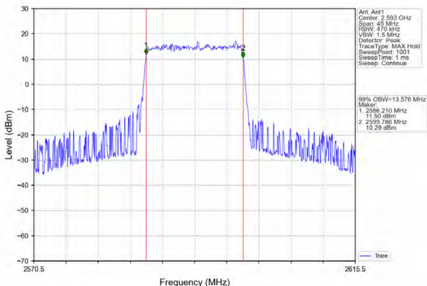
Band41_15MHz_64QAM_MCH_2593MHz_RB_75_0_NTNV
