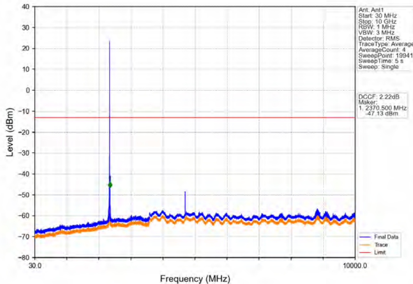
Band40b_5MHz_16QAM_HCH_2357.5MHz_RB_1_0_NTNV
