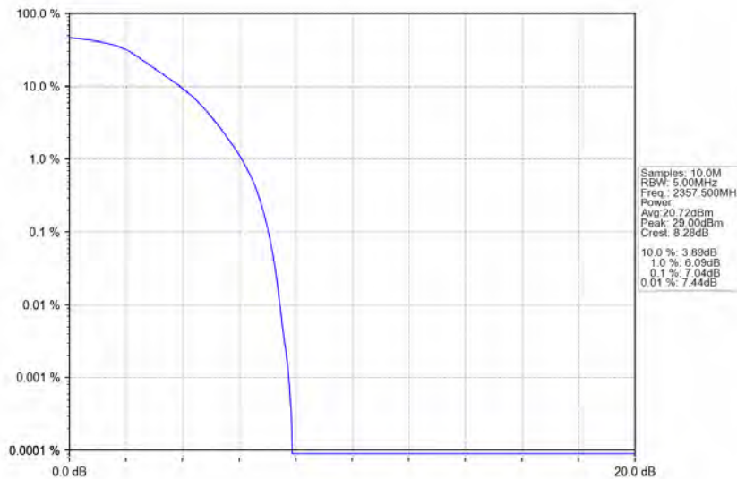
Band40b_5MHz_QPSK_HCH_2357.5MHz_RB_25_0_NTNV
