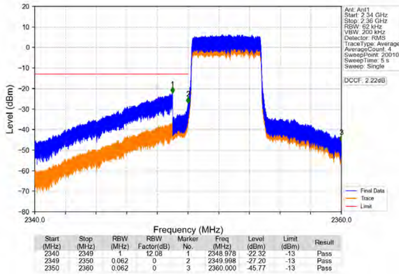
Band40b_5MHz_64QAM_LCH_2352.5MHz_RB_25_0_NTNV
