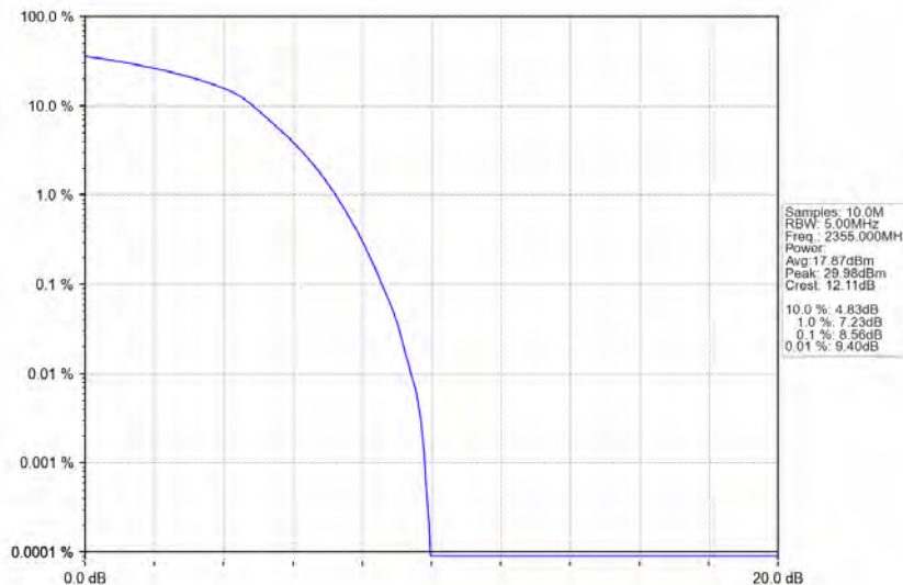
Band40b_10MHz_16QAM_HCH_2355MHz_RB_50_0_NTNV
