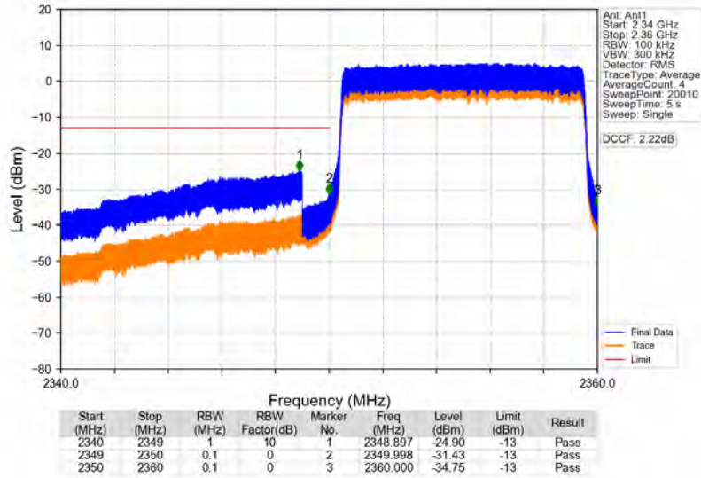
Band40b_10MHz_64QAM_LCH_2355MHz_RB_50_0_NTNV
