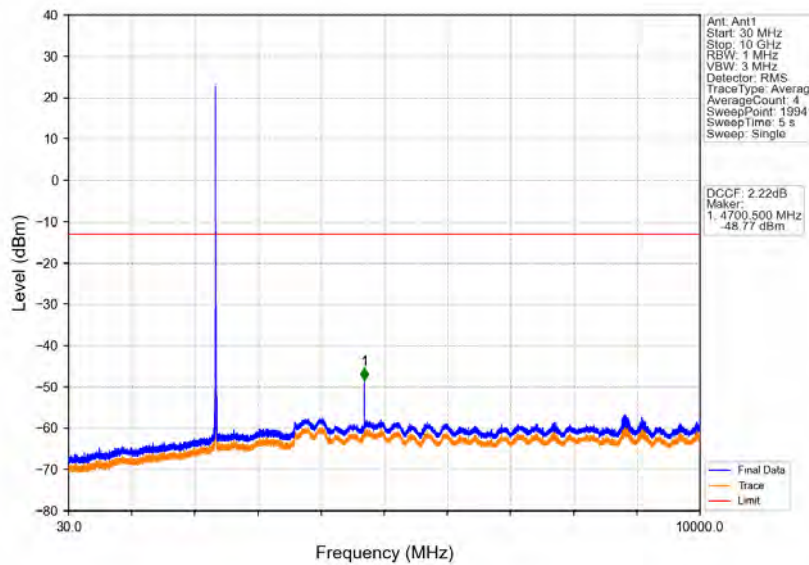
Band40b_5MHz_64QAM_LCH_2352.5MHz_RB_1_0_NTNV
