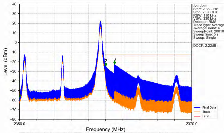
Band40b_10MHz_64QAM_HCH_2355MHz_RB_1_49_NTNV
