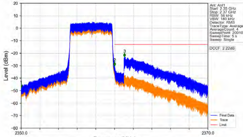
Band40b_5MHz_64QAM_HCH_2357.5MHz_RB_25_0_NTNV
