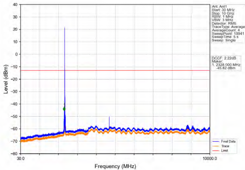
Band40b_10MHz_64QAM_HCH_2355MHz_RB_1_0_NTNV
