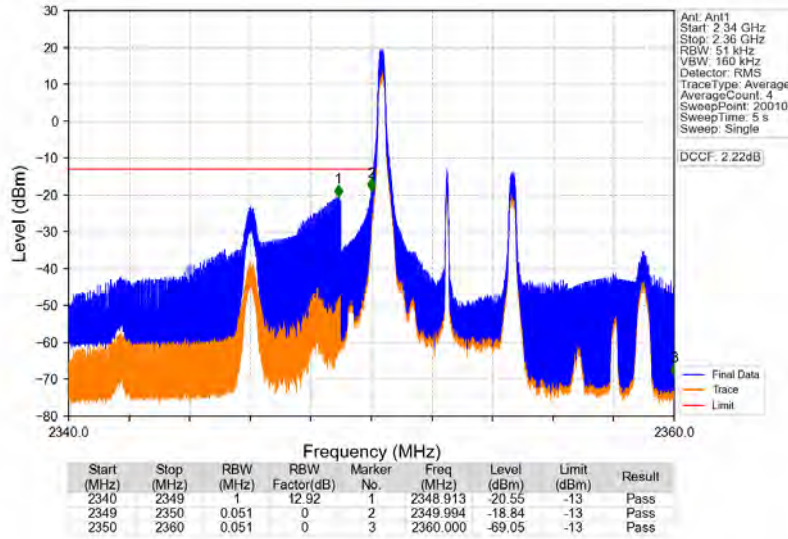
Band40b_5MHz_64QAM_LCH_2352.5MHz_RB_1_0_NTNV
