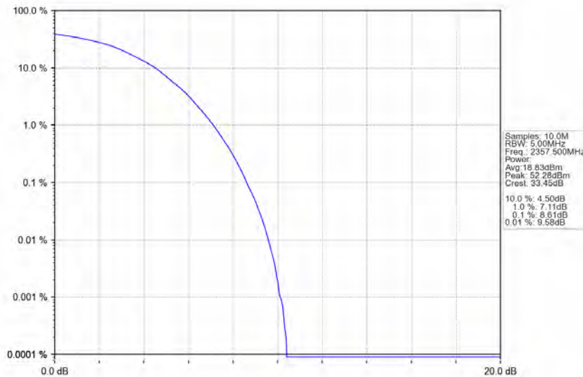
Band40b_5MHz_64QAM_HCH_2357.5MHz_RB_25_0_NTNV
