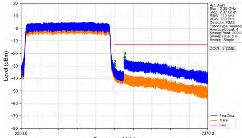
Band40b_10MHz_64QAM_HCH_2355MHz_RB_50_0_NTNV
