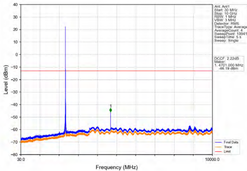
Band40b_10MHz_64QAM_MCH_2355MHz_RB_1_0_NTNV
