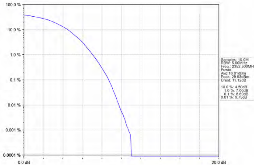
Band40b_5MHz_64QAM_LCH_2352.5MHz_RB_25_0_NTNV
