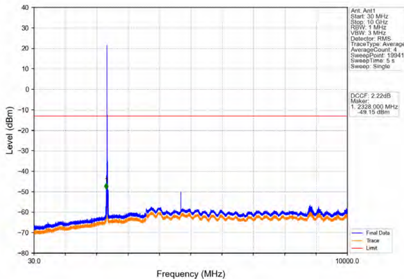
Band40b_10MHz_64QAM_LCH_2355MHz_RB_1_0_NTNV
