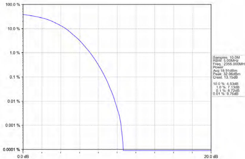
Band40b_5MHz_64QAM_MCH_2355MHz_RB_25_0_NTNV
