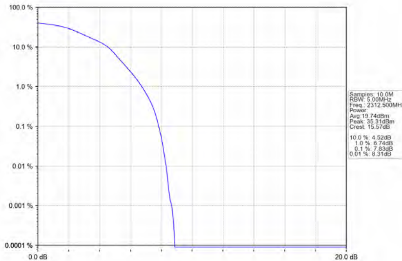
Band40a_5MHz_16QAM_HCH_2312.5MHz_RB_25_0_NTNV
