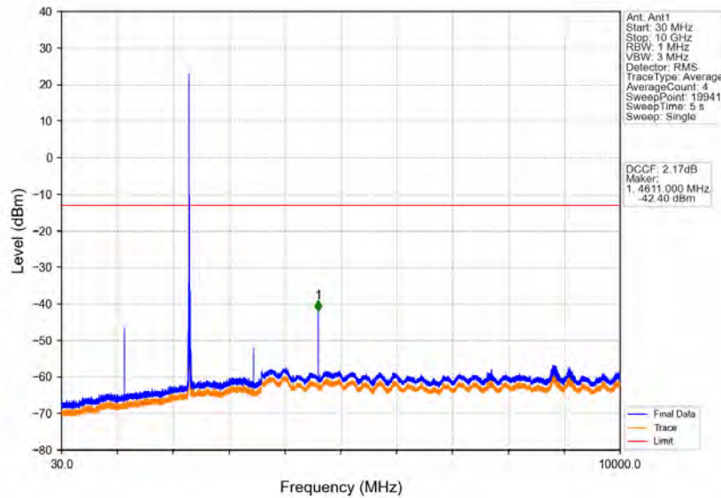
Band40a_10MHz_16QAM_HCH_2310MHz_RB_1_0_NTNV
