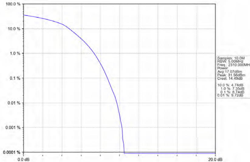
Band40a_10MHz_64QAM_LCH_2310MHz_RB_50_0_NTNV
