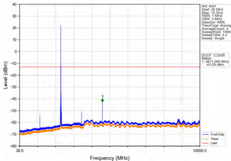
Band40a_10MHz_64QAM_MCH_2310MHz_RB_1_0_NTNV
