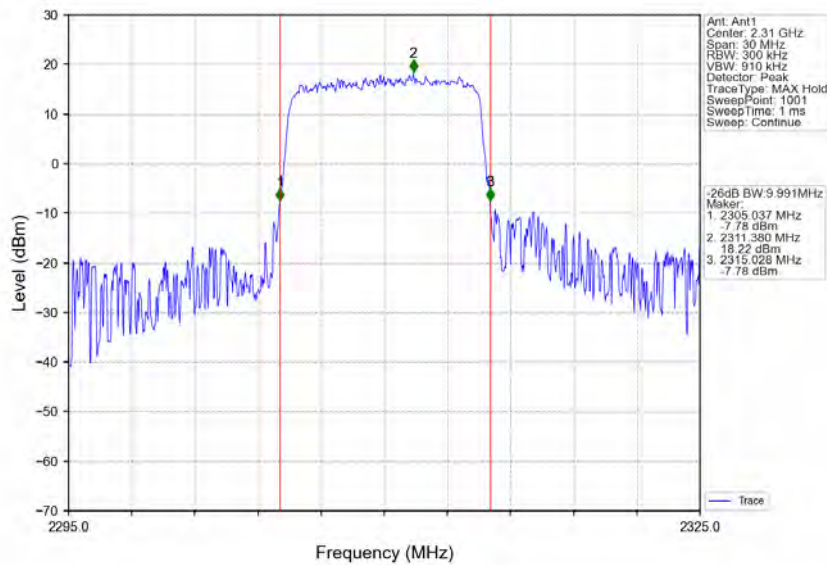
Band40a_10MHz_64QAM_LCH_2310MHz_RB_50_0_NTNV
