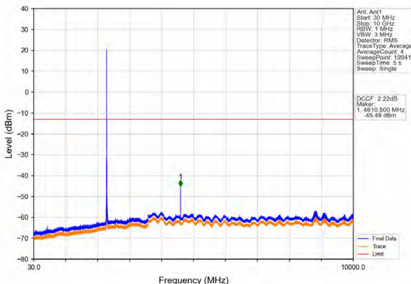
Band40a_5MHz_64QAM_LCH_2307.5MHz_RB_1_0_NTNV
