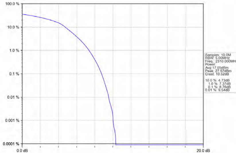
Band40a_10MHz_64QAM_MCH_2310MHz_RB_50_0_NTNV
