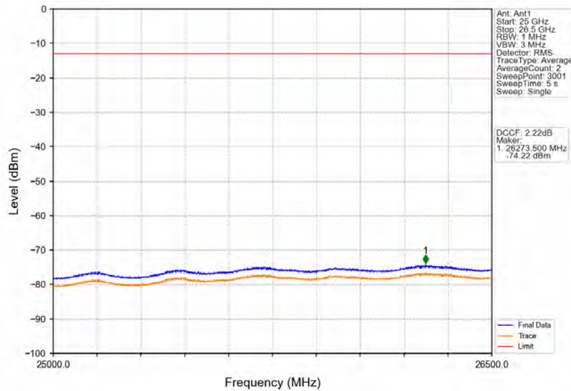
Band40a_10MHz_64QAM_HCH_2310MHz_RB_1_49_NTNV
