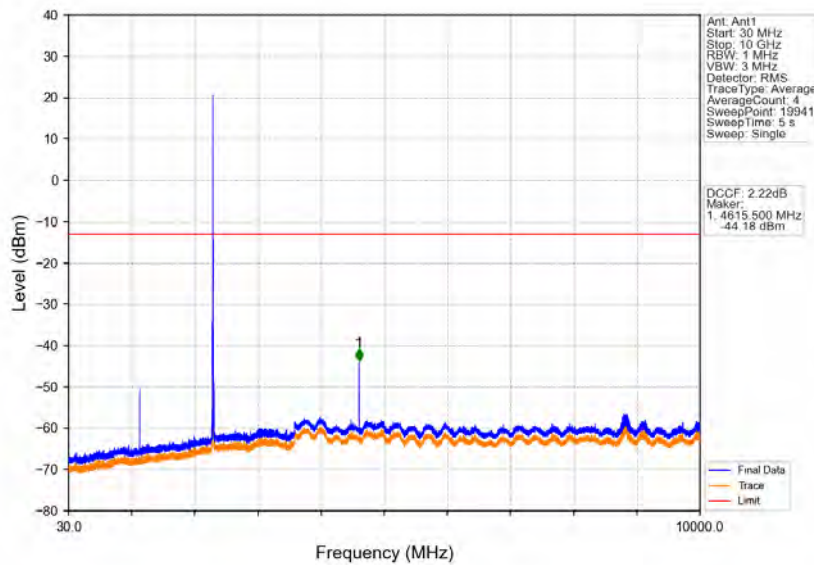
Band40a_5MHz_64QAM_MCH_2310MHz_RB_1_0_NTNV
