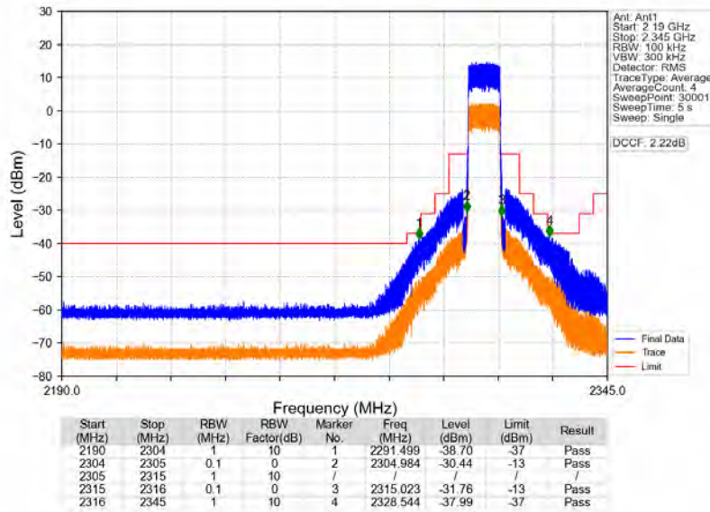
Band40a_10MHz_64QAM_MCH_2310MHz_RB_1_0_NTNV
