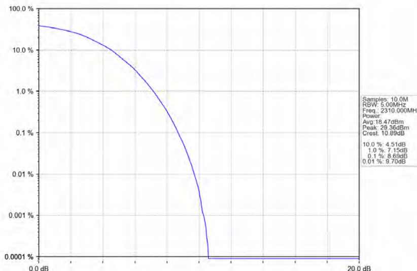
Band40a_5MHz_64QAM_MCH_2310MHz_RB_25_0_NTNV
