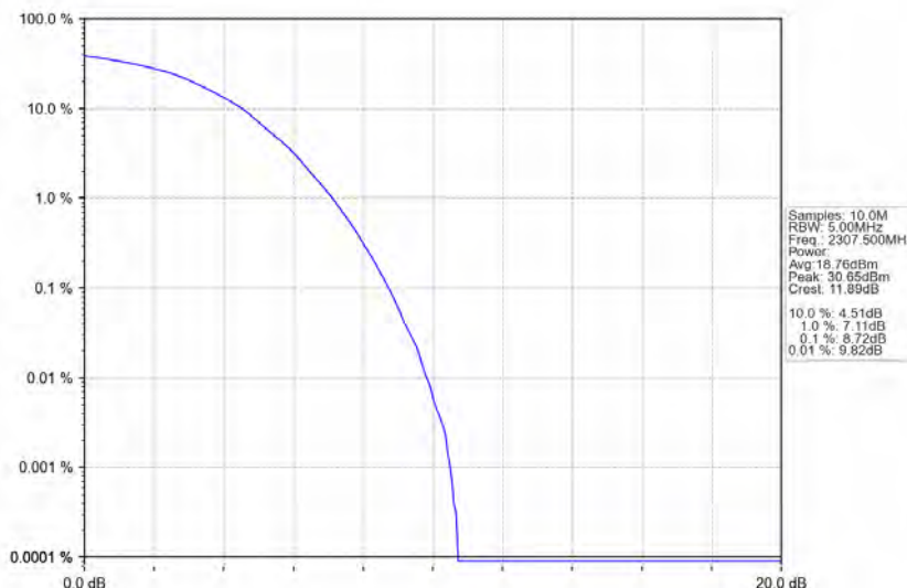
Band40a_5MHz_64QAM_LCH_2307.5MHz_RB_25_0_NTNV
