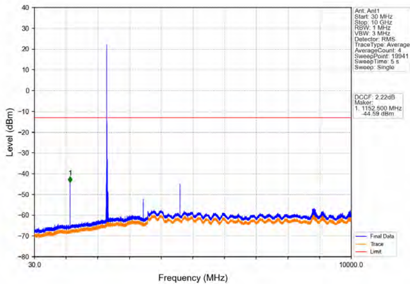
Band40a_10MHz_64QAM_HCH_2310MHz_RB_1_0_NTNV
