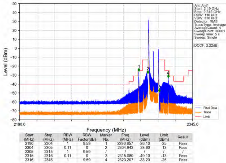
Band40a_10MHz_64QAM_LCH_2310MHz_RB_1_0_NTNV
