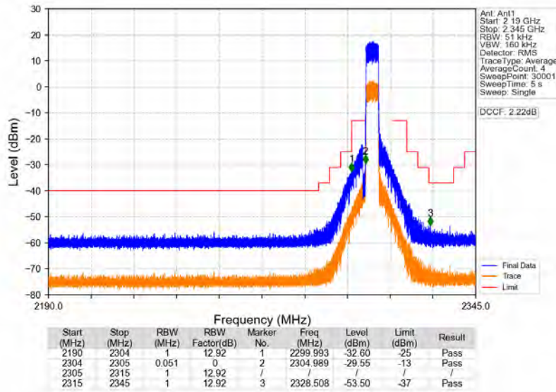
Band40a_5MHz_64QAM_MCH_2310MHz_RB_1_0_NTNV
