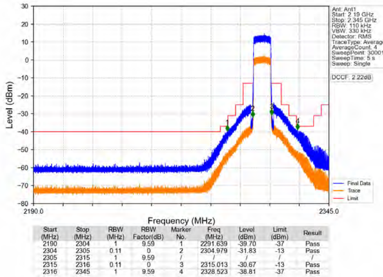
Band40a_10MHz_64QAM_HCH_2310MHz_RB_50_0_NTNV
