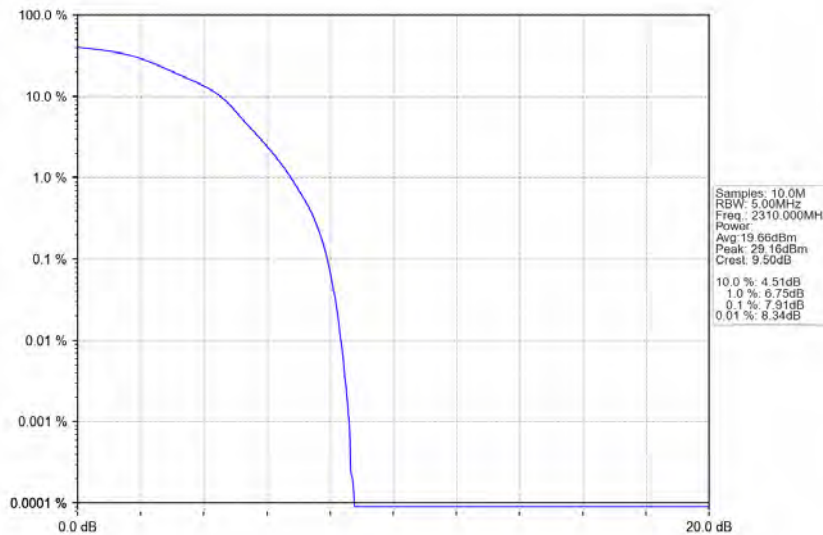
Band40a_5MHz_16QAM_MCH_2310MHz_RB_25_0_NTNV
