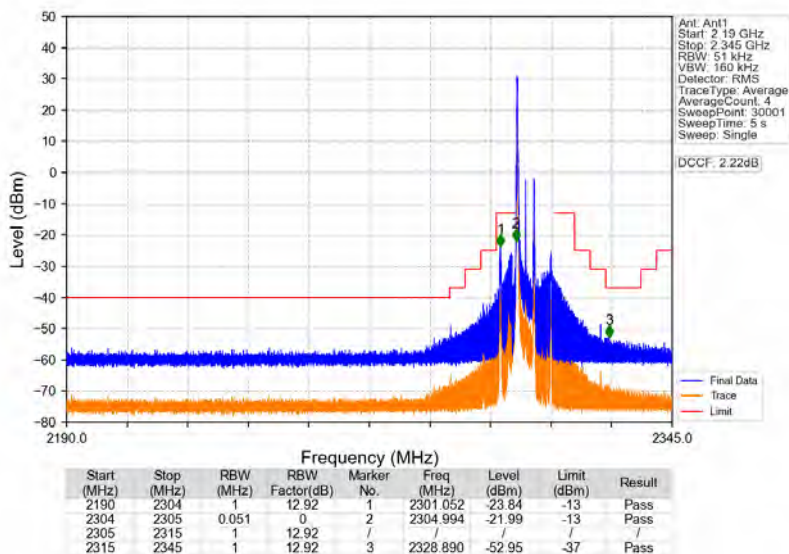
Band40a_5MHz_64QAM_LCH_2307.5MHz_RB_1_0_NTNV
