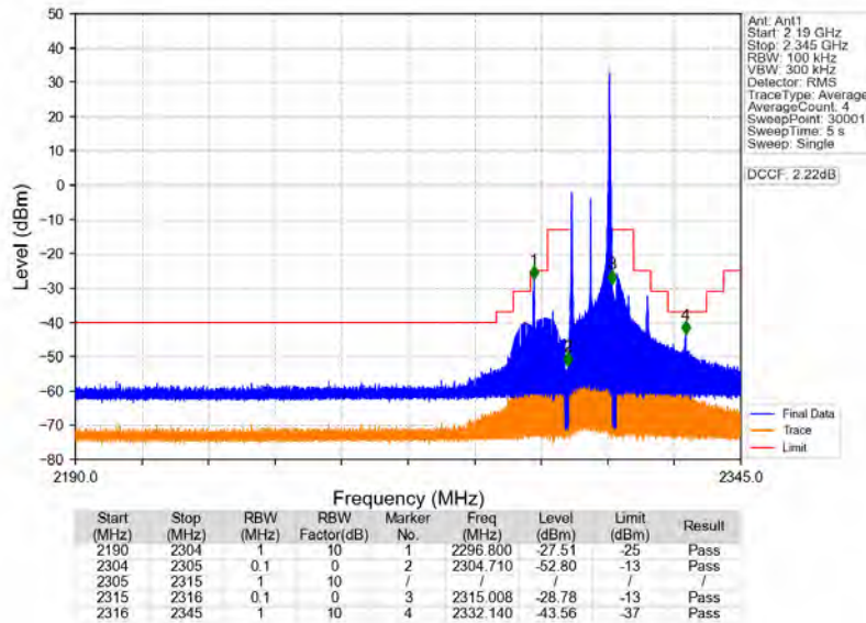
Band40a_10MHz_64QAM_HCH_2310MHz_RB_1_49_NTNV
