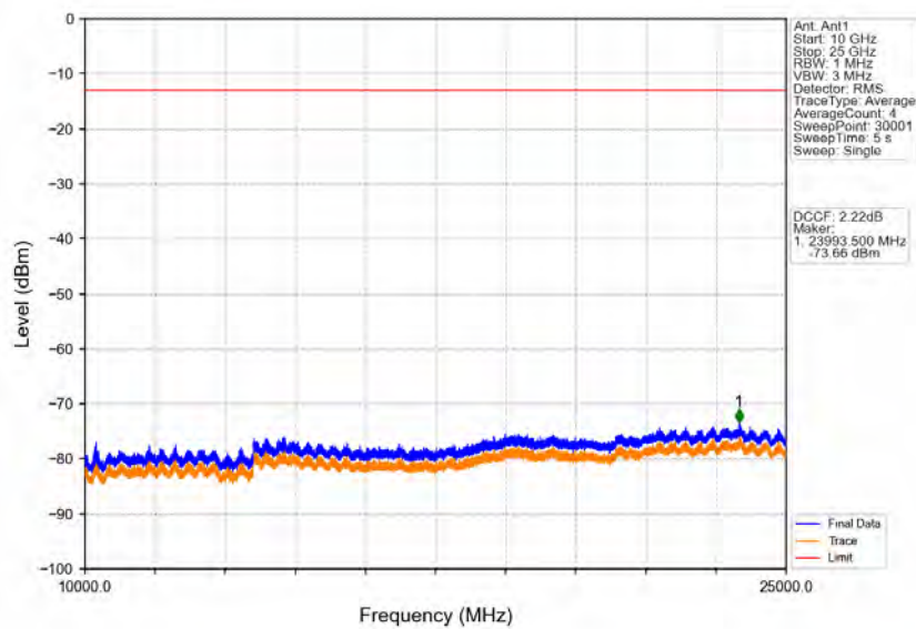
Band40a_5MHz_16QAM_LCH_2307.5MHz_RB_1_0_NTNV
