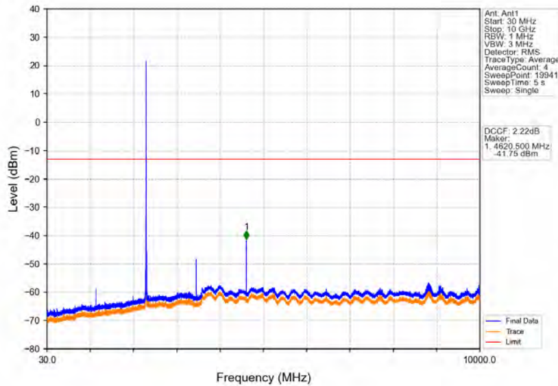
Band40a_5MHz_64QAM_HCH_2312.5MHz_RB_1_0_NTNV
