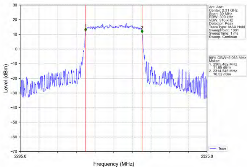
Band40a_10MHz_64QAM_LCH_2310MHz_RB_50_0_NTNV
