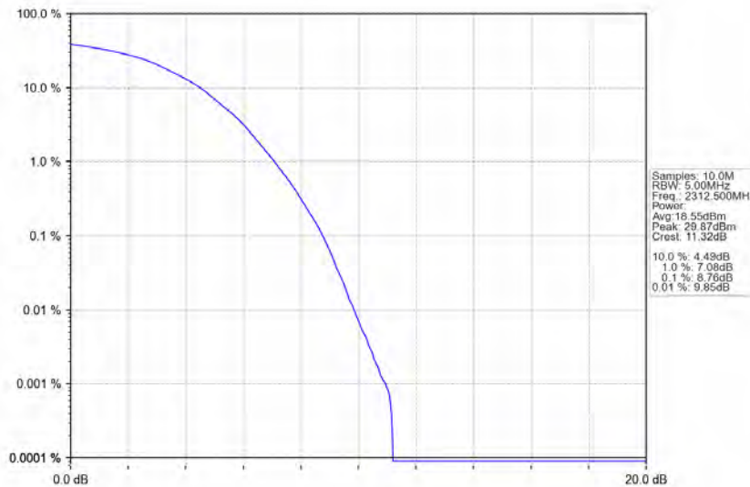
Band40a_5MHz_64QAM_HCH_2312.5MHz_RB_25_0_NTNV
