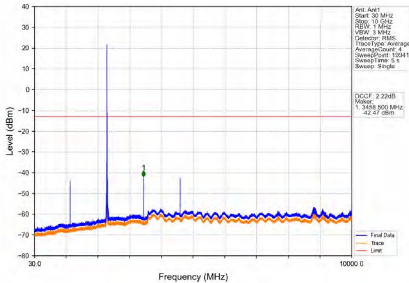
Band40a_10MHz_64QAM_LCH_2310MHz_RB_1_0_NTNV
