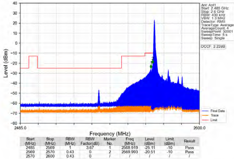
Band38_20MHz_64QAM_LCH_2580MHz_RB_1_0_NTNV
