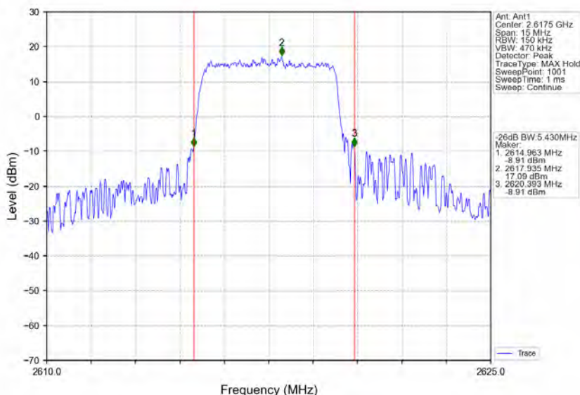
Band38_5MHz_16QAM_HCH_2617.5MHz_RB_25_0_NTNV
