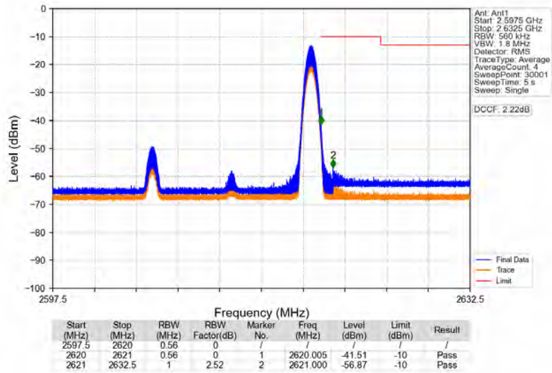
Band38_15MHz_64QAM_HCH_2612.5MHz_RB_1_74_NTNV
