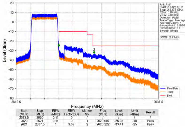
Band38_5MHz_QPSK_HCH_2617.5MHz_RB_25_0_NTNV
