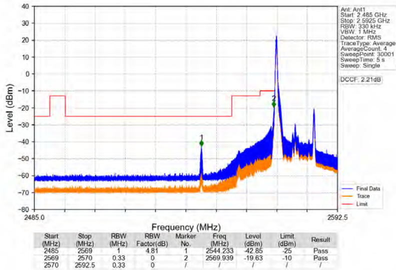
Band38_15MHz_64QAM_LCH_2577.5MHz_RB_1_0_NTNV
