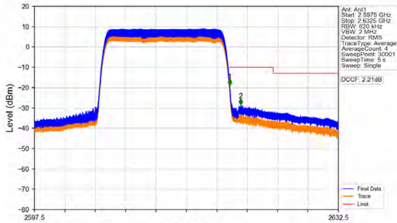
Band38_15MHz_64QAM_HCH_2612.5MHz_RB_75_0_NTNV
