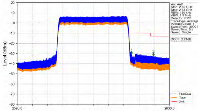
Band38_20MHz_64QAM_HCH_2610MHz_RB_100_0_NTNV
