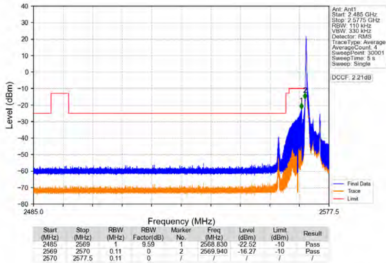
Band38_5MHz_64QAM_LCH_2572.5MHz_RB_1_0_NTNV
