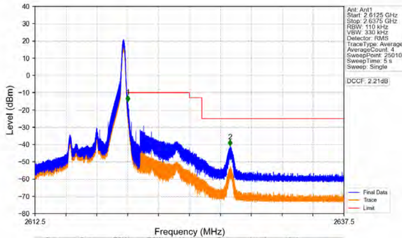
Band38_5MHz_64QAM_HCH_2617.5MHz_RB_1_24_NTNV
