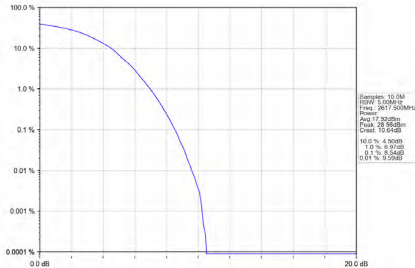
Band38_5MHz_64QAM_HCH_2617.5MHz_RB_25_0_NTNV
