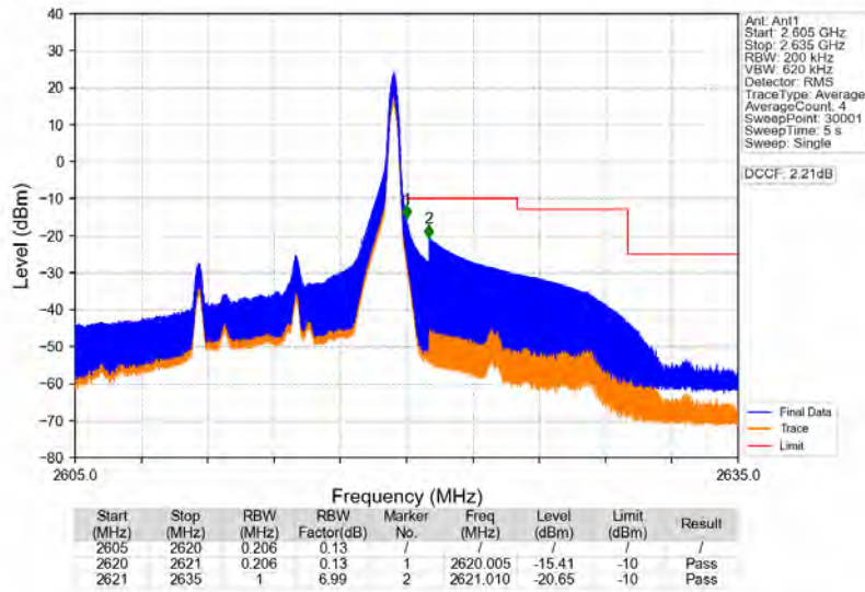
Band38_10MHz_16QAM_HCH_2615MHz_RB_1_49_NTNV
