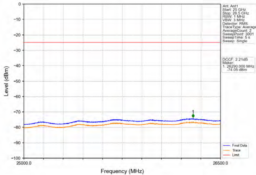
Band38_10MHz_64QAM_HCH_2615MHz_RB_1_49_NTV
