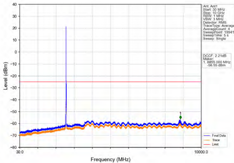
Band38_15MHz_64QAM_LCH_2577.5MHz_RB_1_0_NTNV
