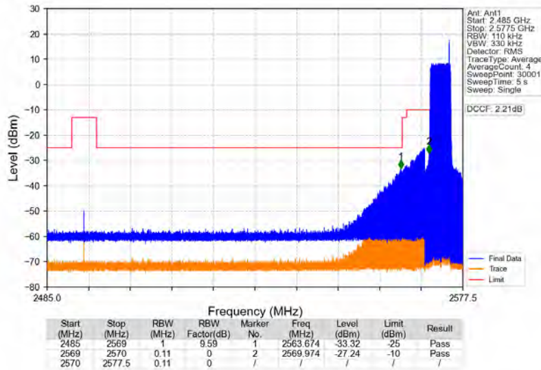
Band38_5MHz_16QAM_LCH_2572.5MHz_RB_25_0_NTNV
