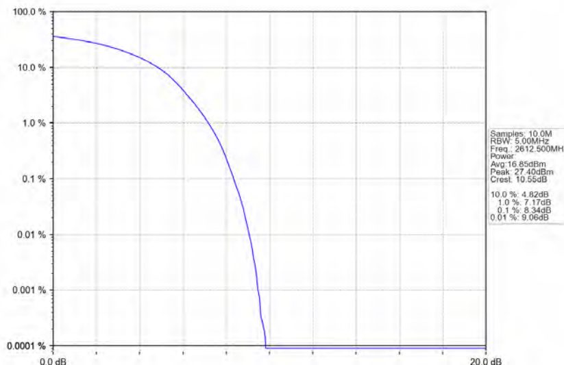
Band38_15MHz_QPSK_HCH_2612.5MHz_RB_75_0_NTNV
