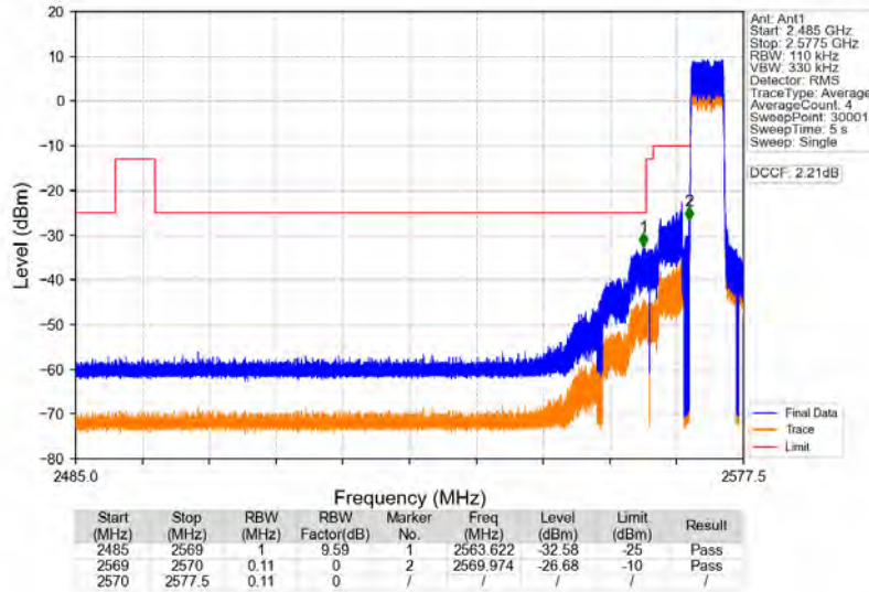
Band38_5MHz_QPSK_LCH_2572.5MHz_RB_25_0_NTNV
