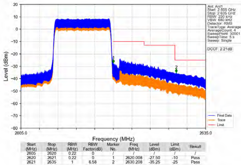
Band38_10MHz_16QAM_HCH_2615MHz_RB_50_0_NTNV
