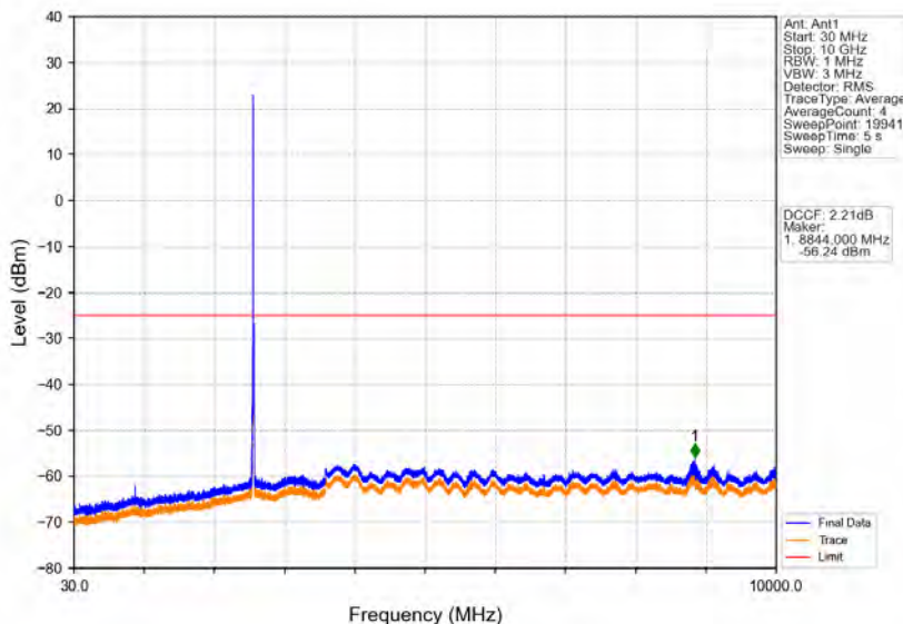
Band38_10MHz_16QAM_LCH_2575MHz_RB_1_0_NTNV
