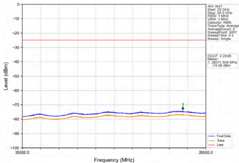
Band38_15MHz_QPSK_LCH_2577.5MHz_RB_1_0_NTV
