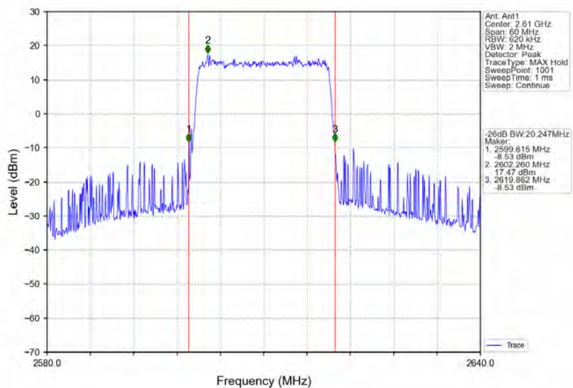
Band38_20MHz_64QAM_HCH_2610MHz_RB_100_0_NTNV
