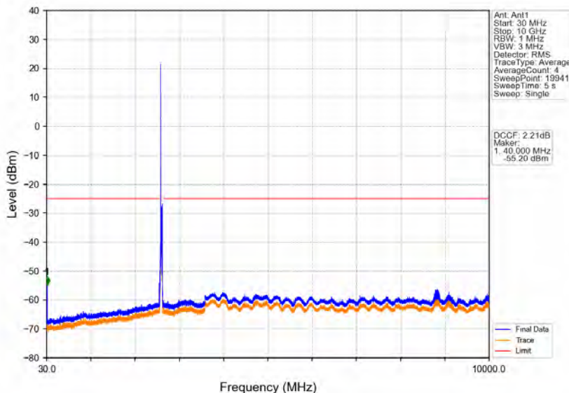
Band38_20MHz_64QAM_HCH_2610MHz_RB_1_0_NTV
