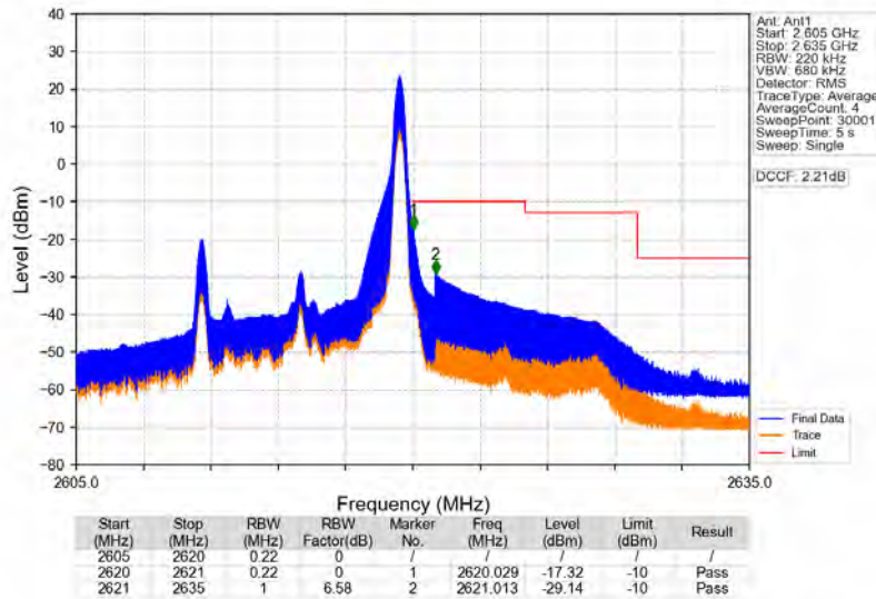
Band38_10MHz_64QAM_HCH_2615MHz_RB_1_49_NTV
