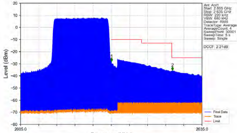
Band38_10MHz_64QAM_HCH_2615MHz_RB_50_0_NTNV
