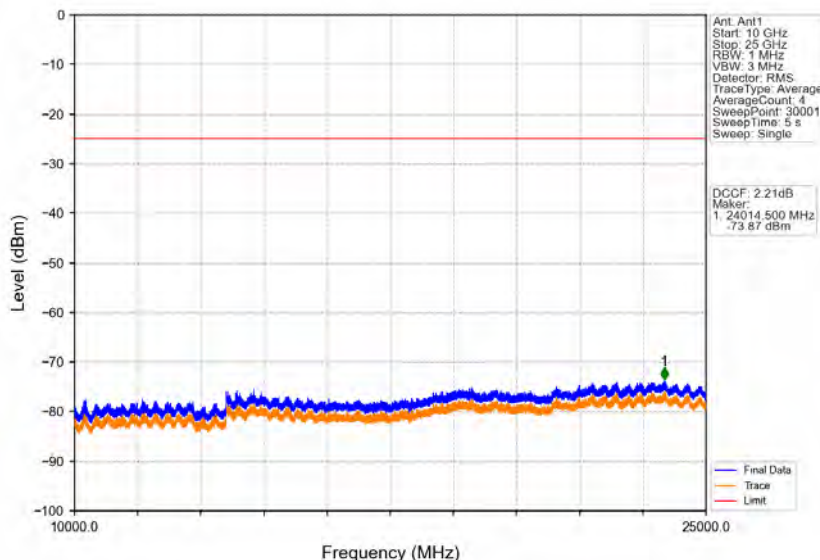
Band38_20MHz_64QAM_HCH_2610MHz_RB_1_0_NTV
