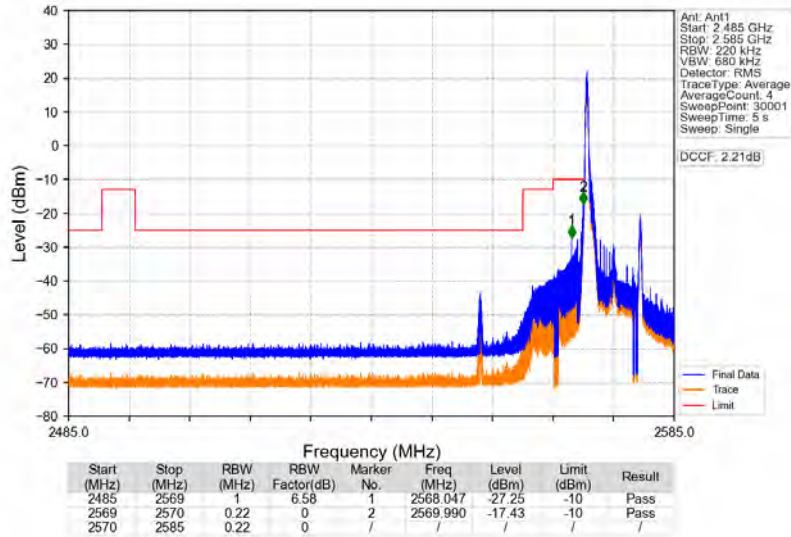
Band38_10MHz_64QAM_LCH_2575MHz_RB_1_0_NTNV
