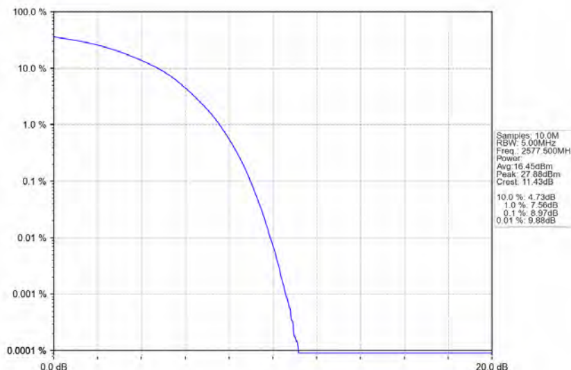
Band38_15MHz_16QAM_LCH_2577.5MHz_RB_75_0_NTNV
