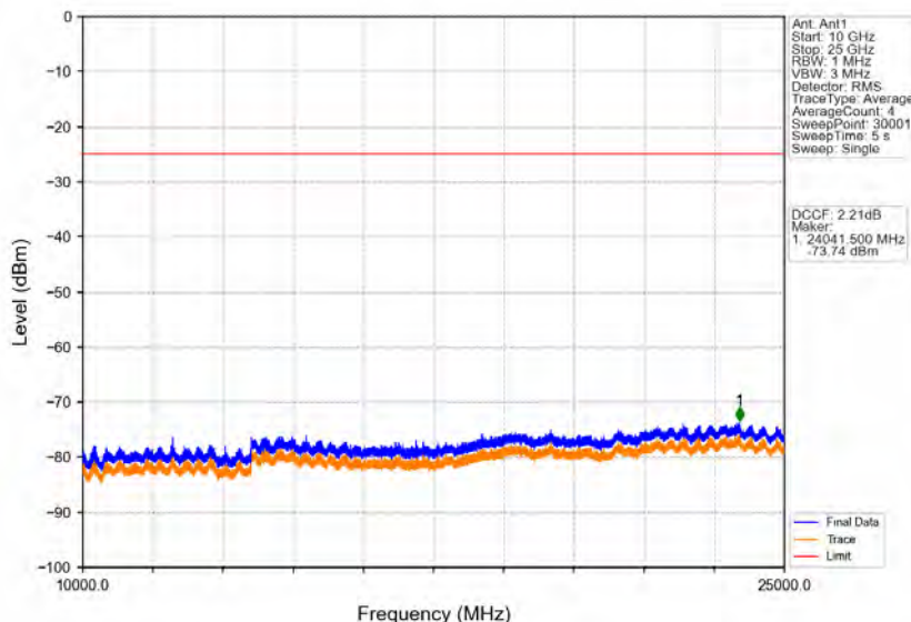
Band38_10MHz_16QAM_LCH_2575MHz_RB_1_0_NTNV
