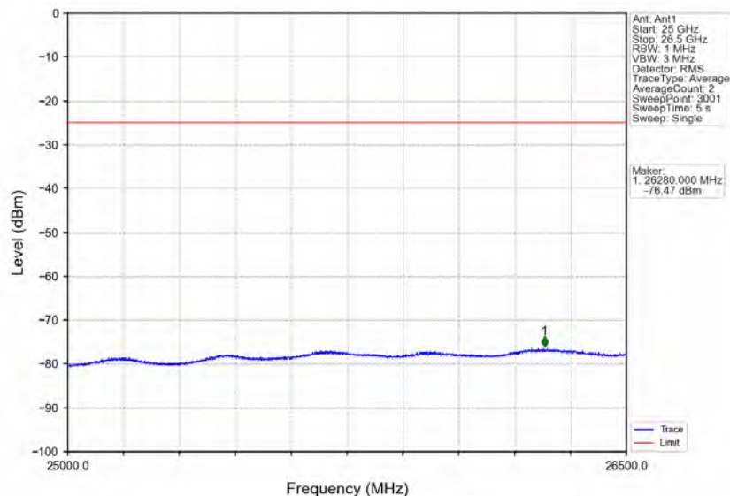
Band7_15MHz_64QAM_HCH_2562.5MHz_RB_1_74_NTNV
