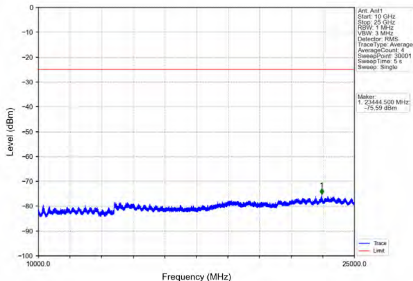
Band7_10MHz_64QAM_MCH_2535MHz_RB_1_0_NTNV
