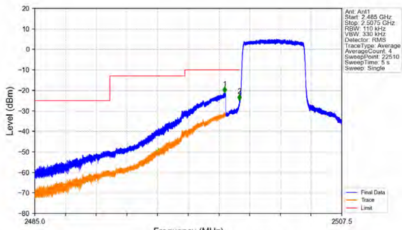
Band7_5MHz_16QAM_LCH_2502.5MHz_RB_25_0_NTNV
