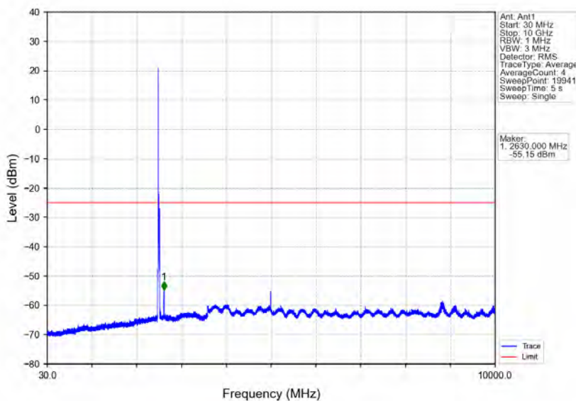
Band7_15MHz_64QAM_LCH_2507.5MHz_RB_1_0_NTNV
