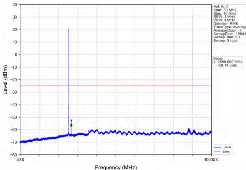
Band7_5MHz_64QAM_HCH_2567.5MHz_RB_1_0_NTNV
