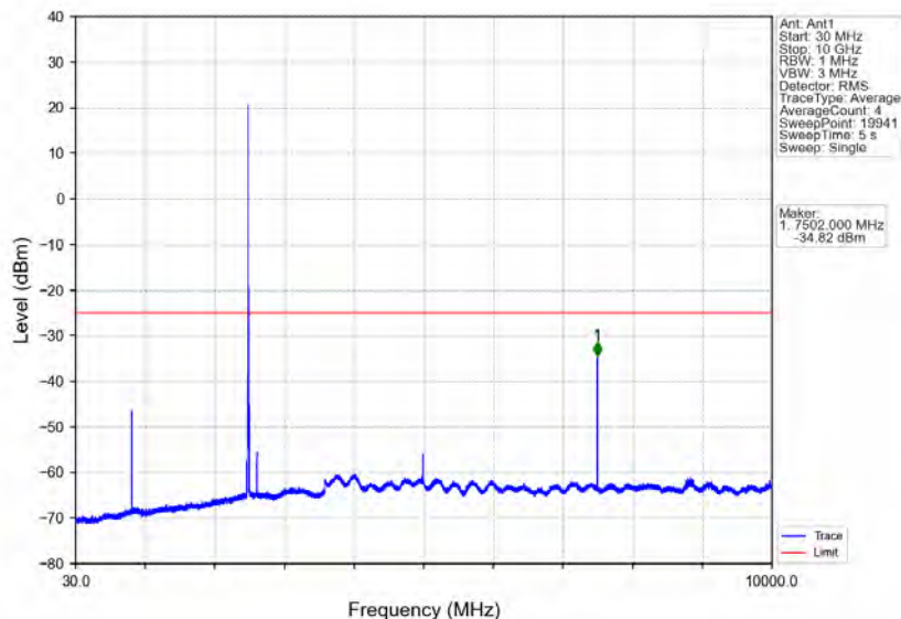
Band7_10MHz_16QAM_LCH_2505MHz_RB_1_0_NTNV
