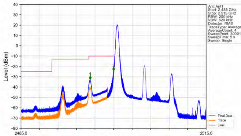
Band7_10MHz_16QAM_LCH_2505MHz_RB_1_0_NTNV
