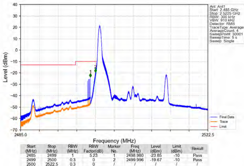
Band7_15MHz_64QAM_LCH_2507.5MHz_RB_1_0_NTNV
