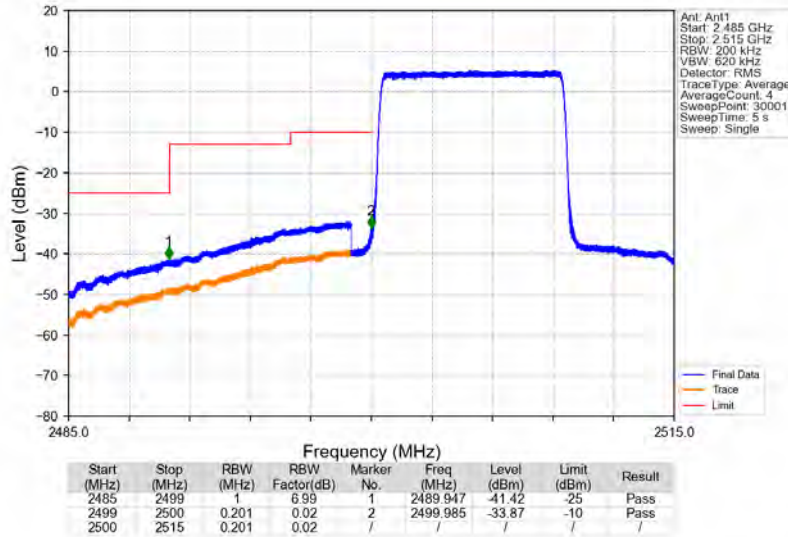
Band7_10MHz_64QAM_LCH_2505MHz_RB_50_0_NTNV
