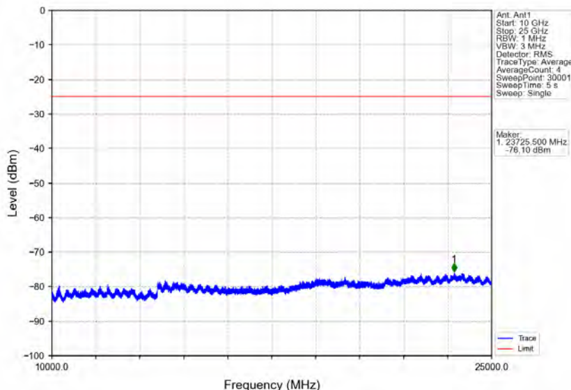
Band7_5MHz_64QAM_HCH_2567.5MHz_RB_1_0_NTNV
