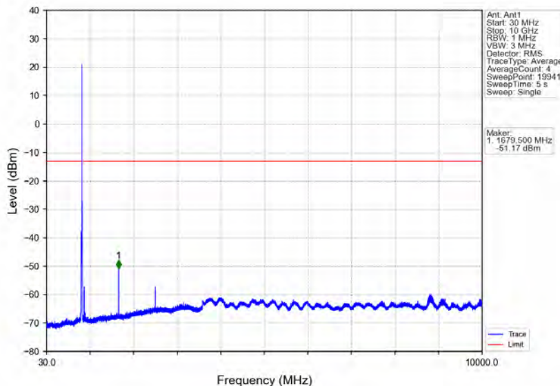
Band5_10MHz_64QAM_HCH_844MHz_RB_1_49_NTNV
