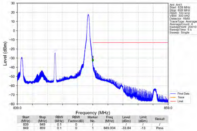
Band5_10MHz_16QAM_HCH_844MHz_RB_1_49_NTNV
