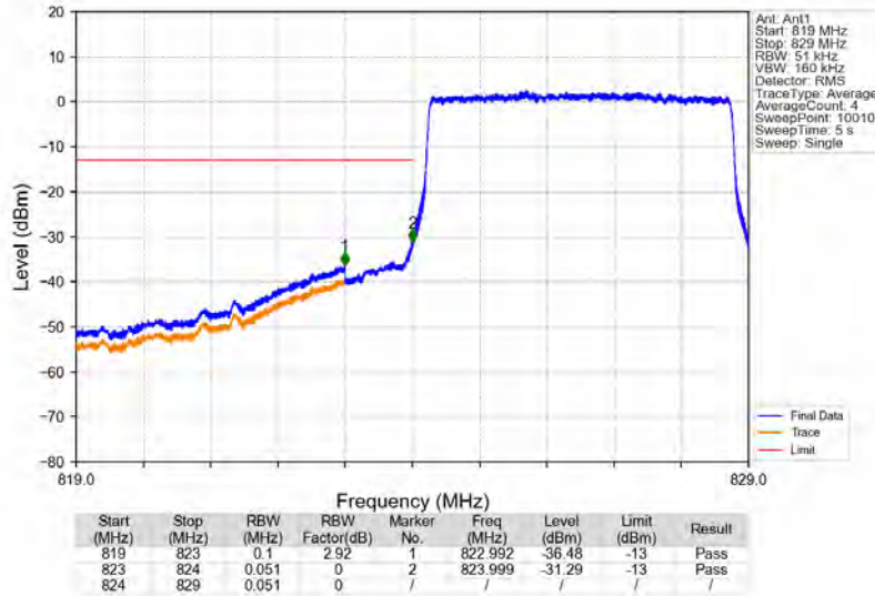
Band5_5MHz_QPSK_LCH_826.5MHz_RB_25_0_NTNV
