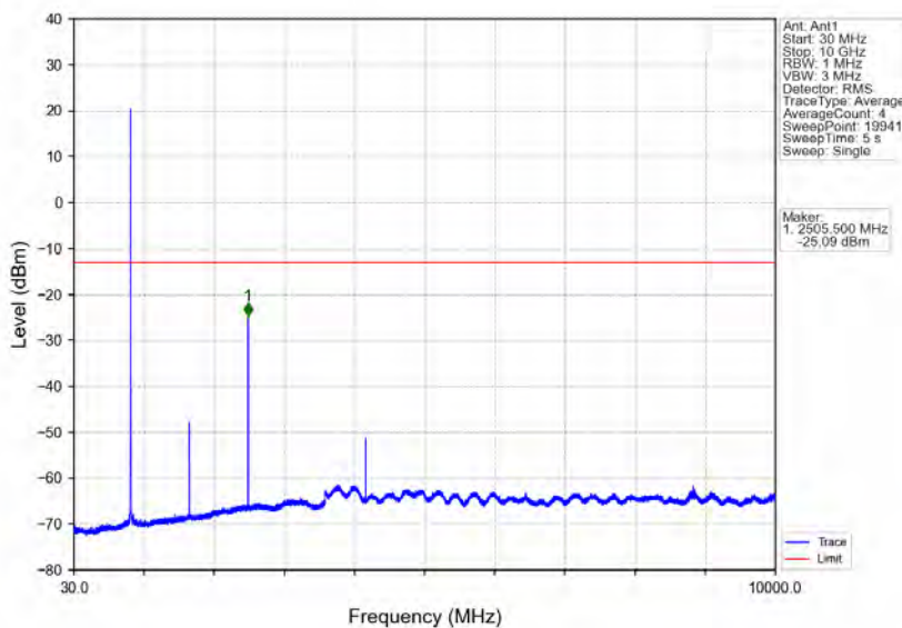
Band5_3MHz_QPSK_MCH_836.5MHz_RB_1_0_NTNV
