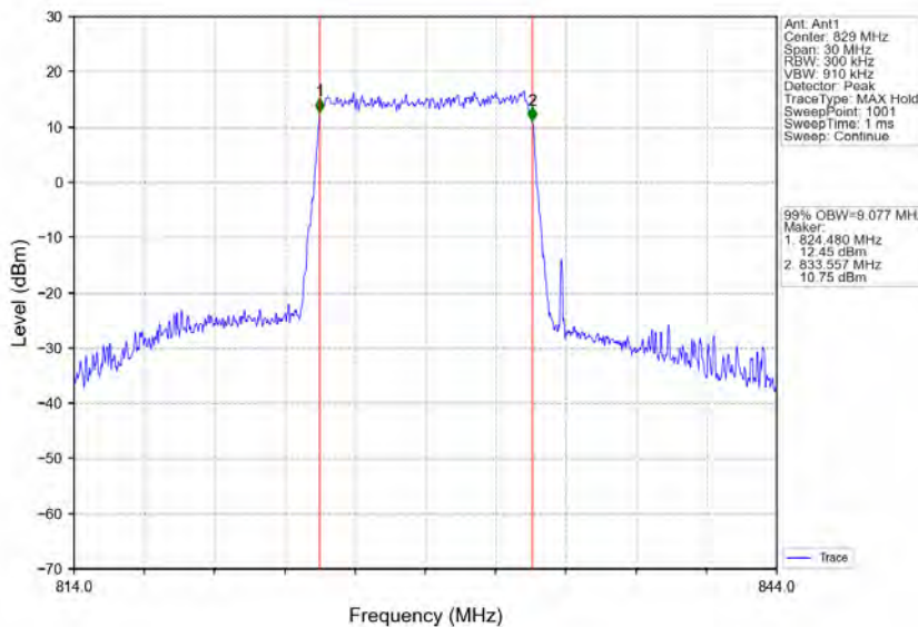
Band5_10MHz_64QAM_LCH_829MHz_RB_50_0_NTNV
