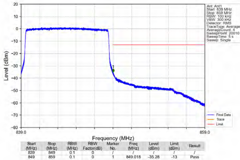
Band5_10MHz_16QAM_HCH_844MHz_RB_50_0_NTNV
