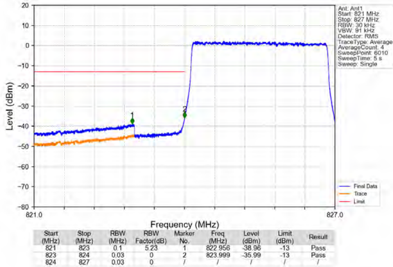
Band5_3MHz_64QAM_LCH_825.5MHz_RB_15_0_NTNV
