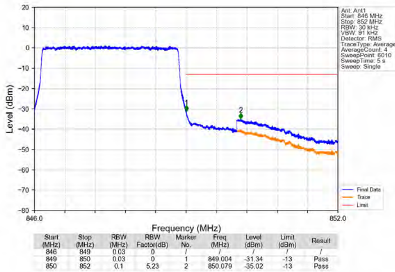
Band5_3MHz_16QAM_HCH_847.5MHz_RB_15_0_NTNV
