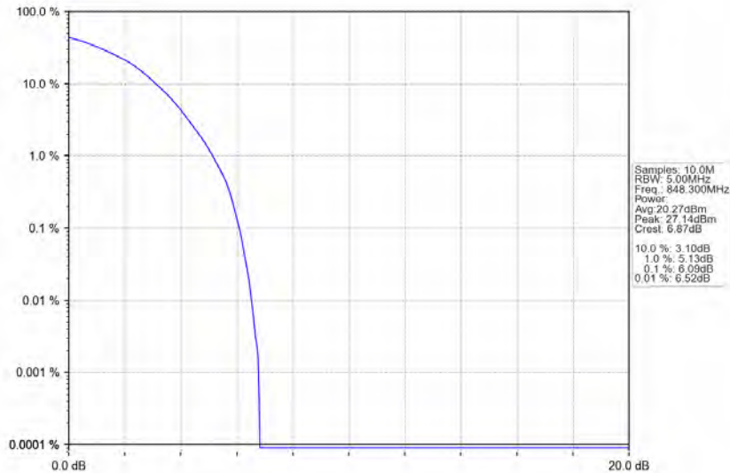
Band5_1.4MHz_64QAM_HCH_848.3MHz_RB_6_0_NTV
