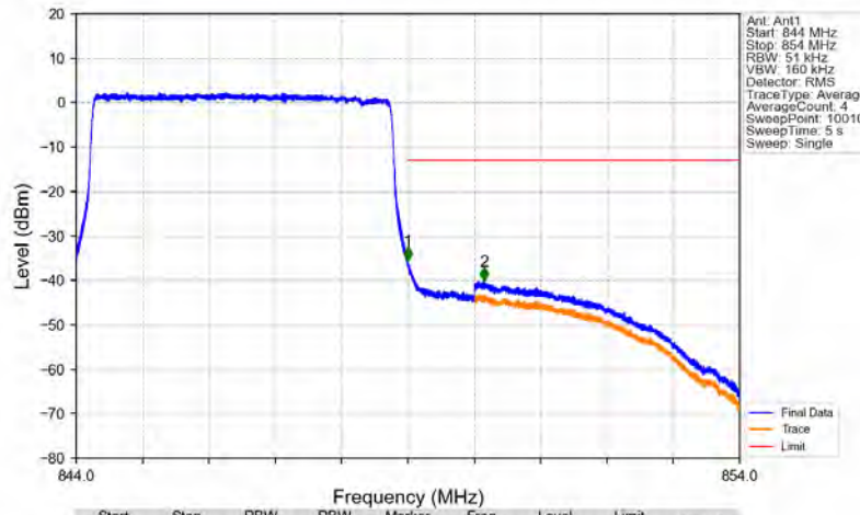
Band5_5MHz_64QAM_HCH_846.5MHz_RB_25_0_NTNV
