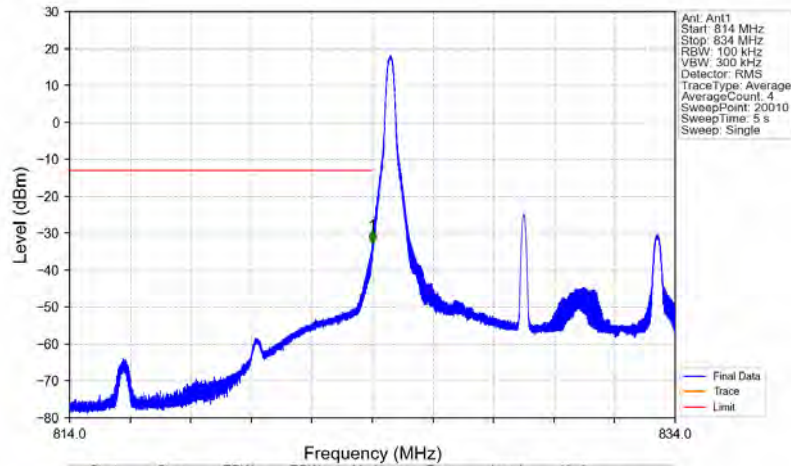
Band5_10MHz_16QAM_LCH_829MHz_RB_1_0_NTNV
