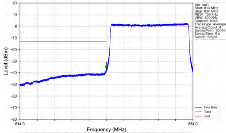
Band5_10MHz_64QAM_LCH_829MHz_RB_50_0_NTNV
