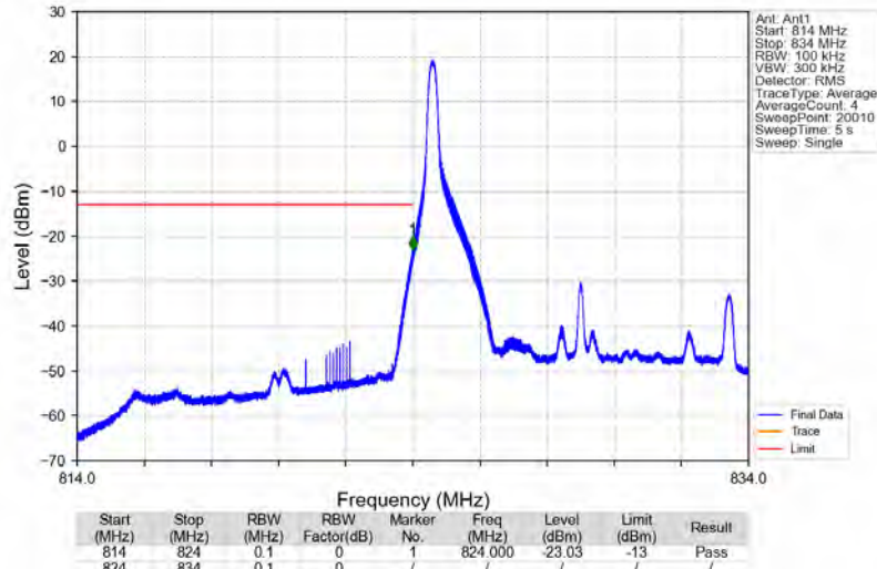
Band5_10MHz_64QAM_LCH_829MHz_RB_1_0_NTNV
