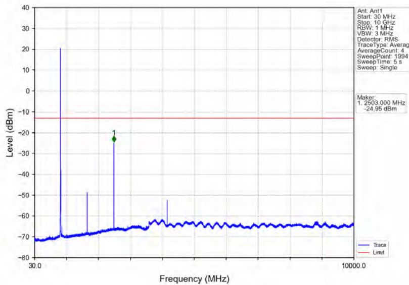
Band5_5MHz_QPSK_MCH_836.5MHz_RB_1_0_NTNV
