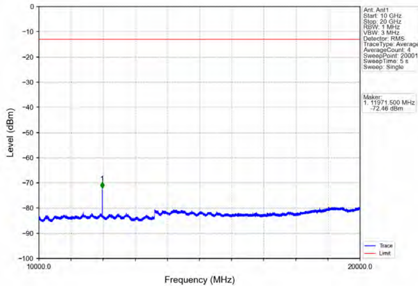
Band4_1.4MHz_QPSK_LCH_1710.7MHz_RB_6_0_NTNV
