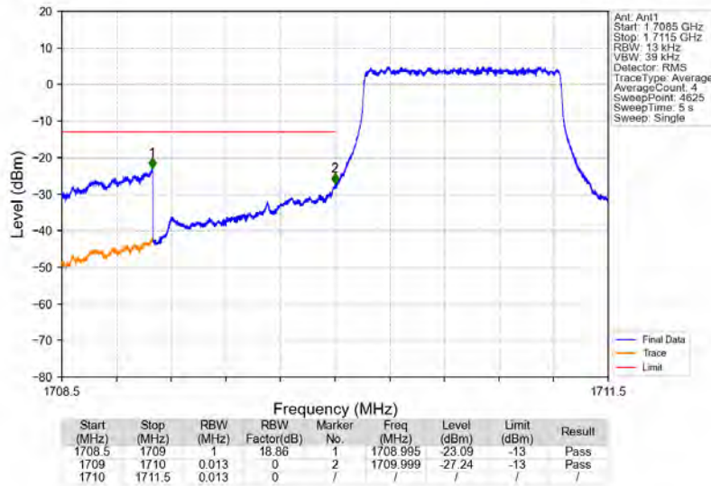
Band4_1.4MHz_QPSK_LCH_1710.7MHz_RB_6_0_NTNV
