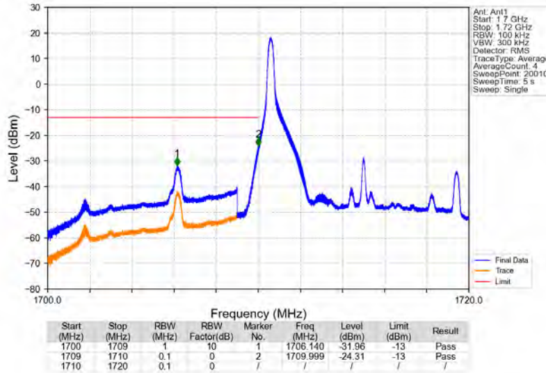
Band4_10MHz_64QAM_LCH_1715MHz_RB_1_0_NTV
