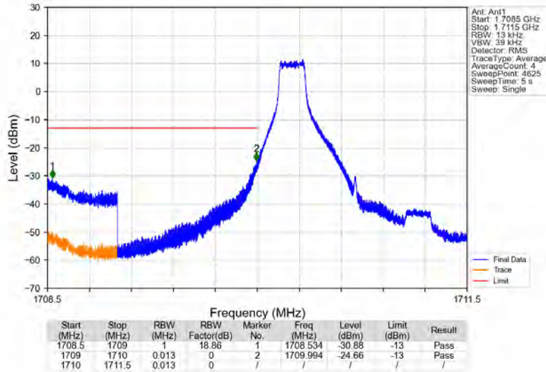
Band4_1.4MHz_64QAM_LCH_1710.7MHz_RB_1_0_NTNV
