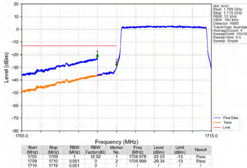
Band4_5MHz_16QAM_LCH_1712.5MHz_RB_25_0_NTNV
