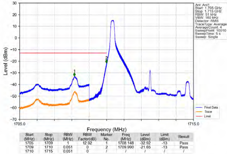
Band4_5MHz_64QAM_LCH_1712.5MHz_RB_1_0_NTNV
