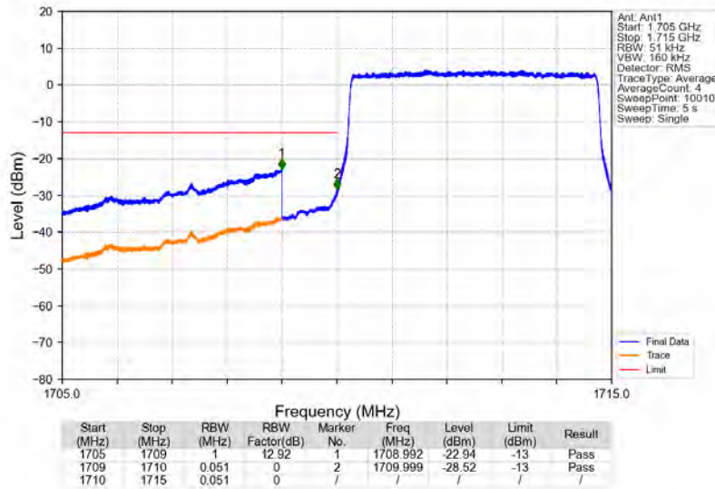
Band4_5MHz_QPSK_LCH_1712.5MHz_RB_25_0_NTNV
