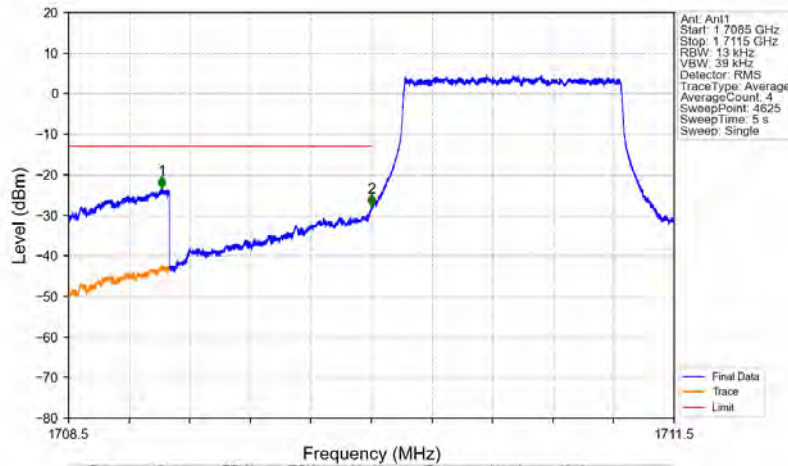
Band4_1.4MHz_16QAM_LCH_1710.7MHz_RB_6_0_NTNV
