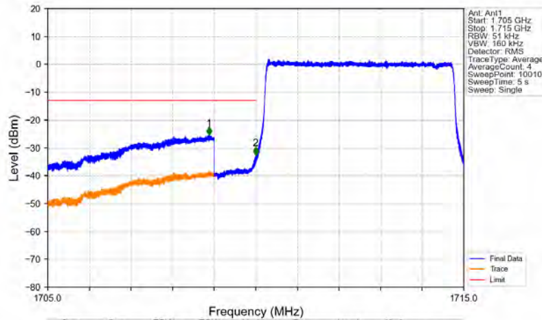
Band4_5MHz_64QAM_LCH_1712.5MHz_RB_25_0_NTNV
