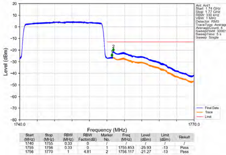
Band4_15MHz_16QAM_HCH_1747.5MHz_RB_75_0_NTNV
