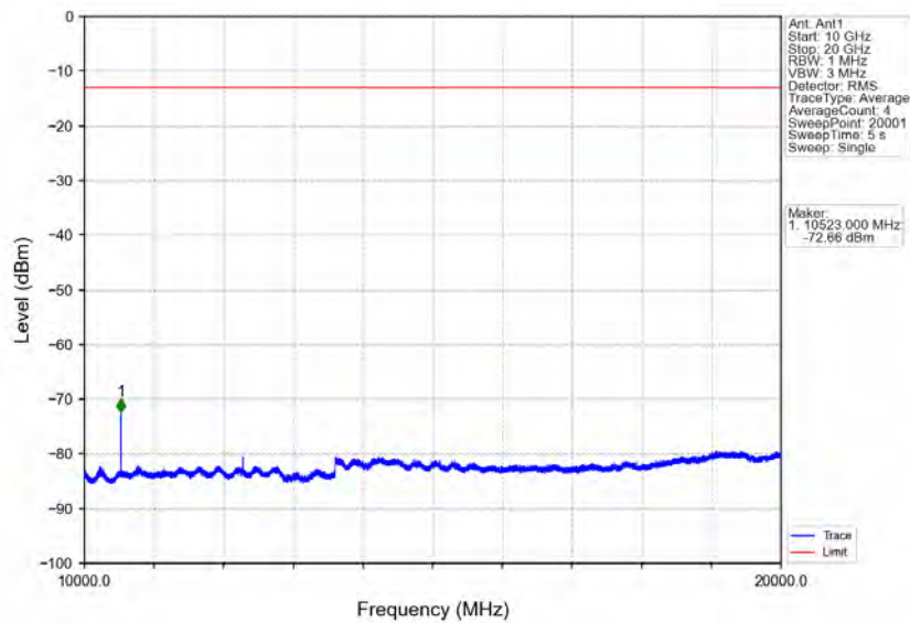
Band4_1.4MHz_QPSK_HCH_1754.3MHz_RB_1_0_NTV
