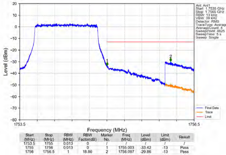
Band4_1.4MHz_64QAM_HCH_1754.3MHz_RB_6_0_NTNV
