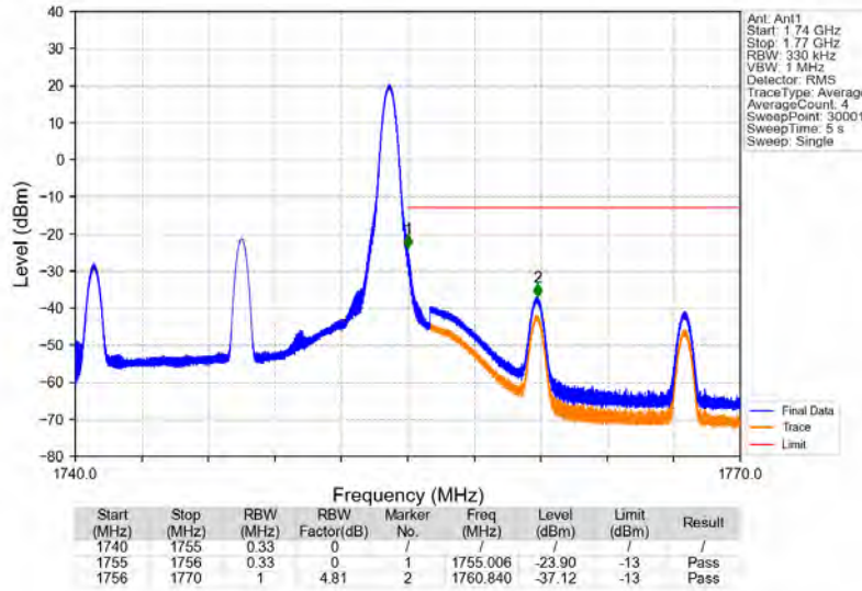
Band4_15MHz_16QAM_HCH_1747.5MHz_RB_1_74_NTNV
