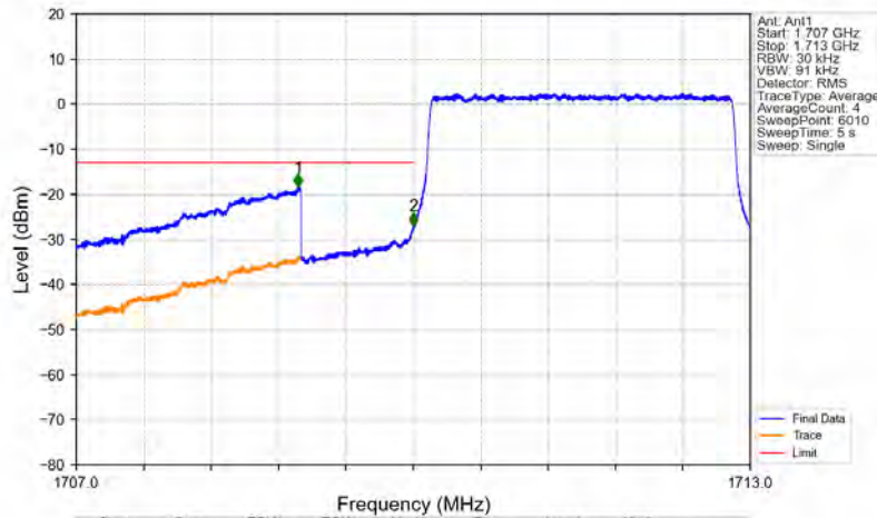
Band4_3MHz_16QAM_LCH_1711.5MHz_RB_15_0_NTNV
