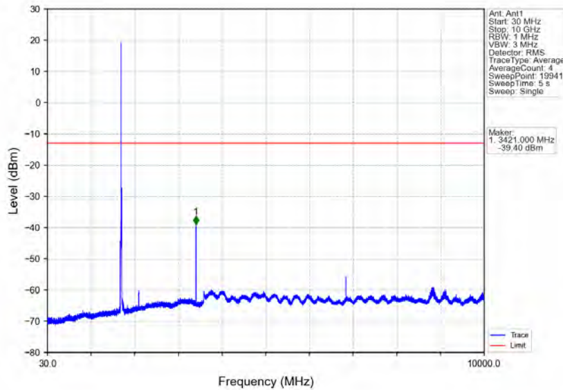
Band4_10MHz_64QAM_LCH_1715MHz_RB_1_0_NTV
