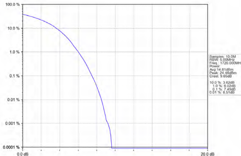
Band4_20MHz_64QAM_LCH_1720MHz_RB_100_0_NTNV
