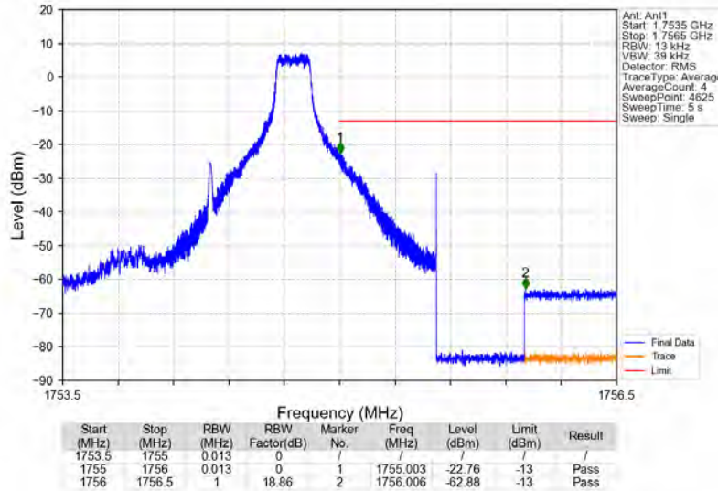
Band4_1.4MHz_16QAM_HCH_1754.3MHz_RB_1_5_NTNV
