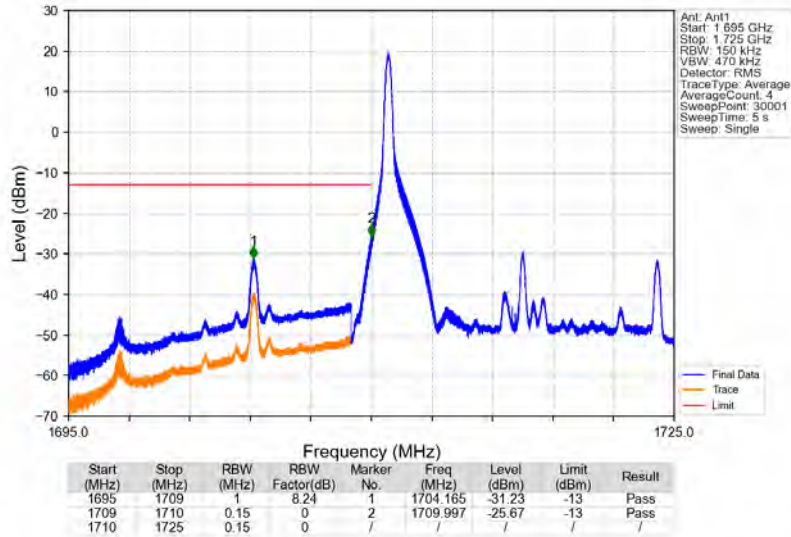
Band4_15MHz_64QAM_LCH_1717.5MHz_RB_1_0_NTNV
