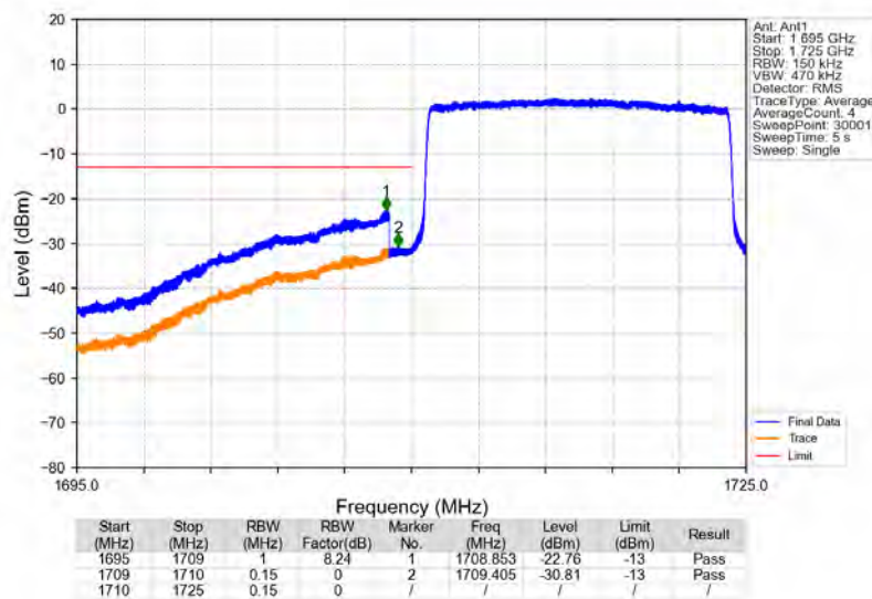
Band4_15MHz_16QAM_LCH_1717.5MHz_RB_75_0_NTNV
