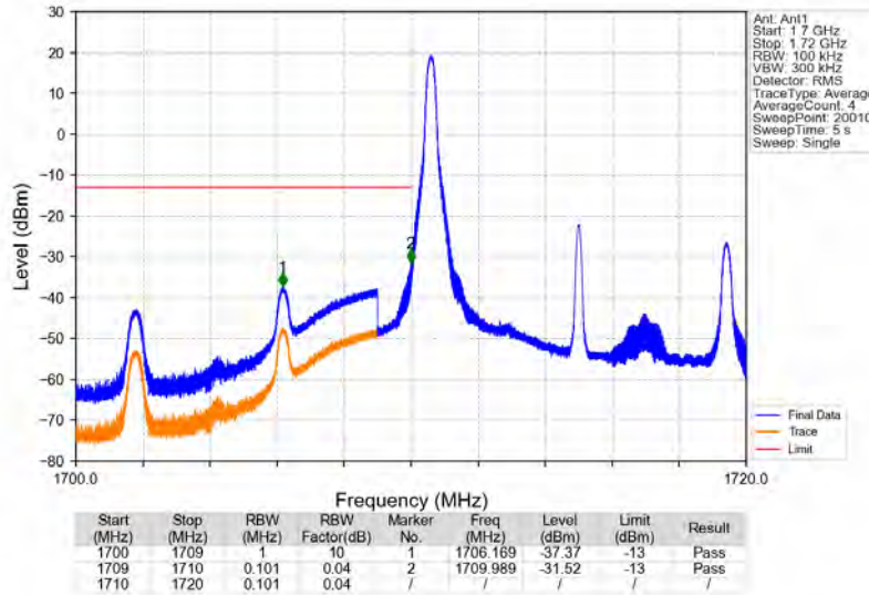
Band4_10MHz_16QAM_LCH_1715MHz_RB_1_0_NTNV
