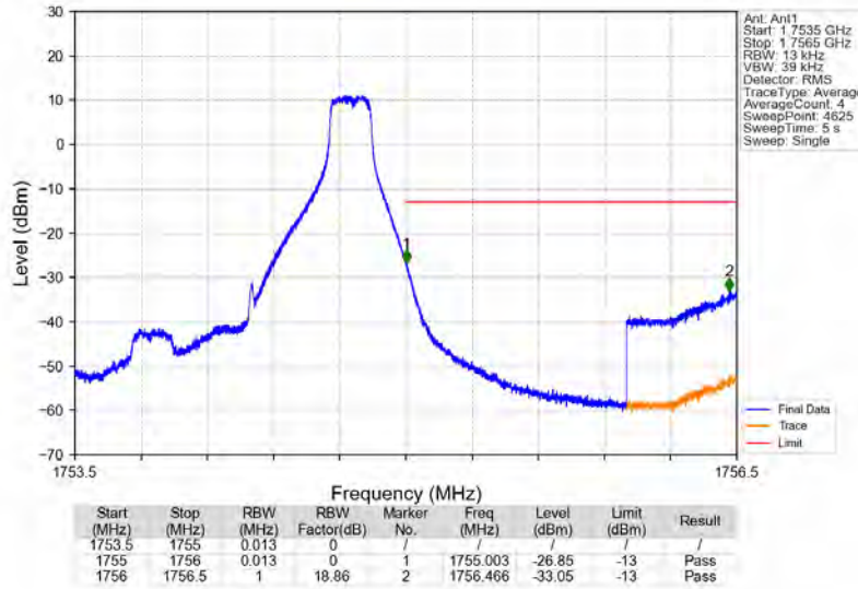
Band4_1.4MHz_64QAM_HCH_1754.3MHz_RB_1_5_NTNV
