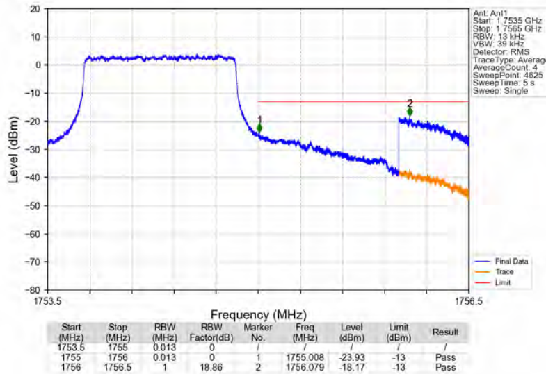
Band4_1.4MHz_16QAM_HCH_1754.3MHz_RB_6_0_NTNV
