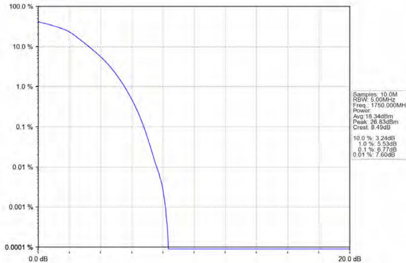
Band4_10MHz_64QAM_HCH_1750MHz_RB_50_0_NTNV
