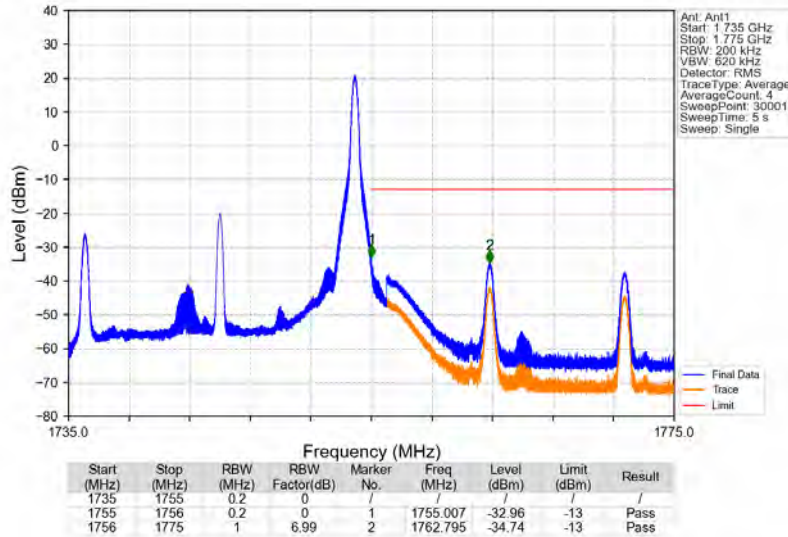
Band4_20MHz_16QAM_HCH_1745MHz_RB_1_99_NTNV
