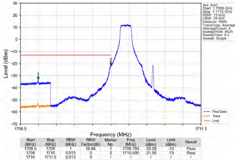
Band4_1.4MHz_16QAM_LCH_1710.7MHz_RB_1_0_NTNV
