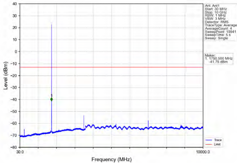
Band4_1.4MHz_QPSK_HCH_1754.3MHz_RB_1_0_NTV
