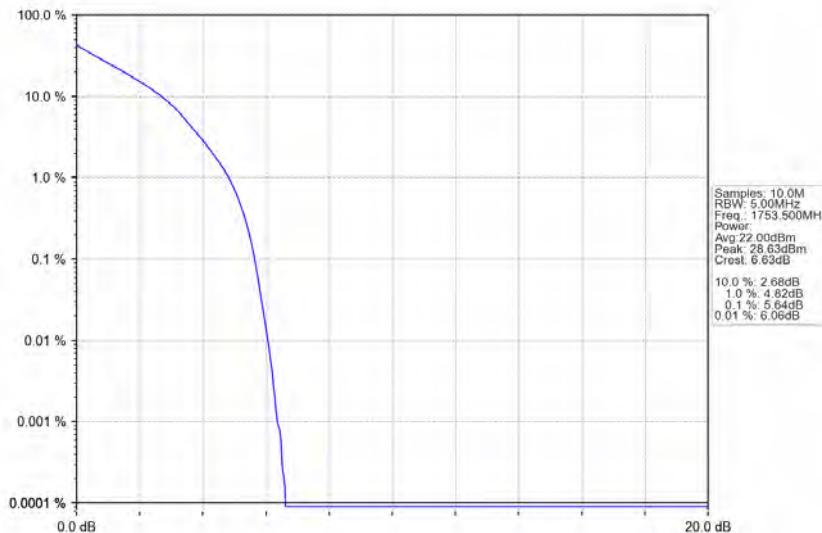
Band4_3MHz_QPSK_HCH_1753.5MHz_RB_15_0_NTNV
