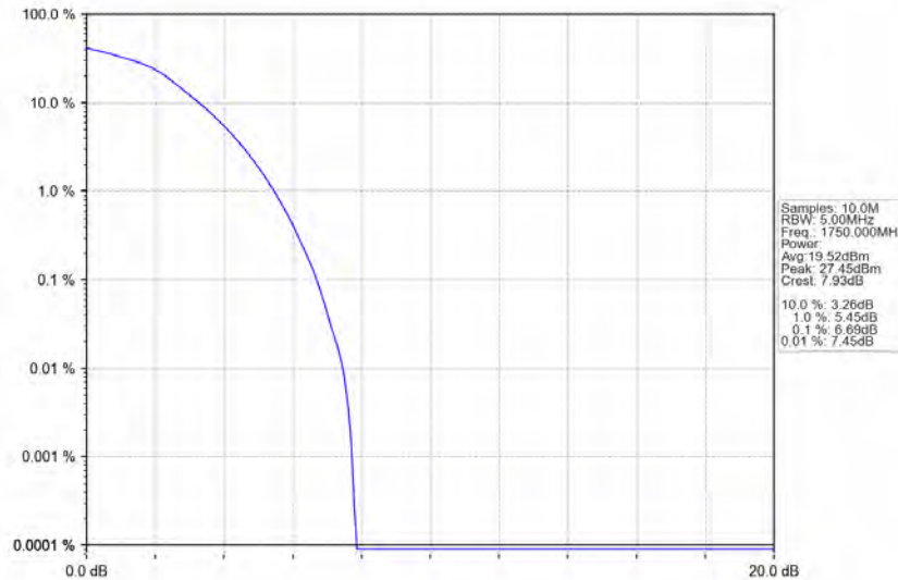
Band4_10MHz_16QAM_HCH_1750MHz_RB_50_0_NTNV
