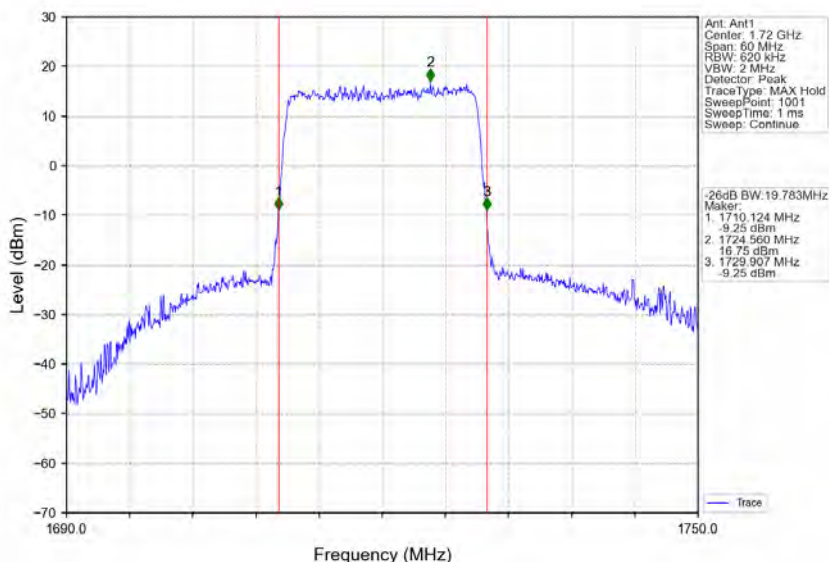
Band4_20MHz_64QAM_LCH_1720MHz_RB_100_0_NTNV
