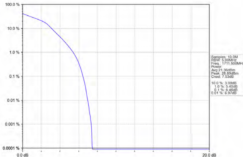
Band4_3MHz_16QAM_LCH_1711.5MHz_RB_15_0_NTNV
