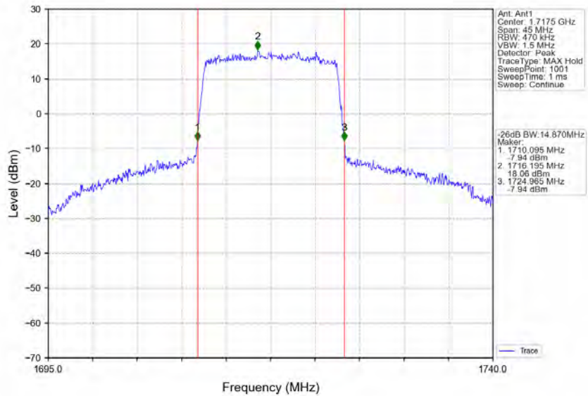
Band4_15MHz_16QAM_LCH_1717.5MHz_RB_75_0_NTNV
