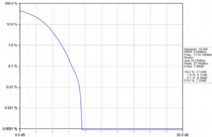
Band4_1.4MHz_64QAM_LCH_1710.7MHz_RB_6_0_NTNV
