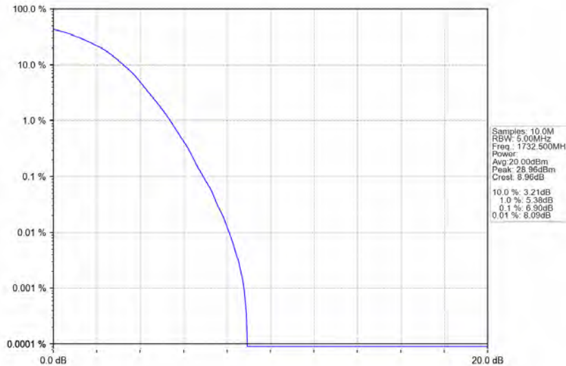
Band4_1.4MHz_64QAM_MCH_1732.5MHz_RB_6_0_NTNV
