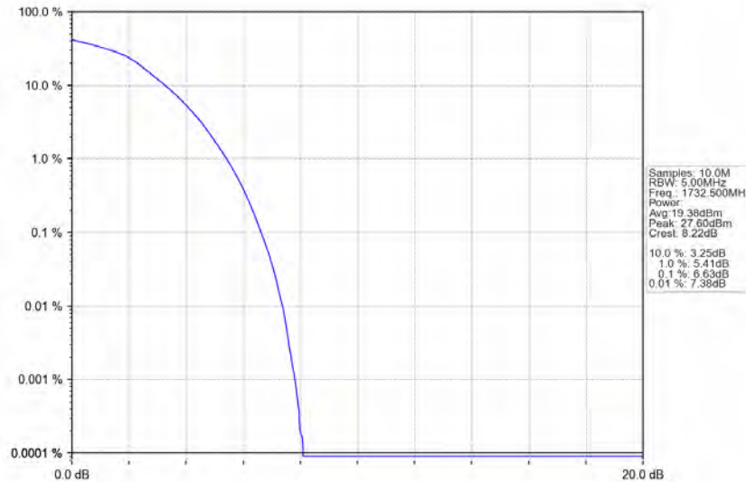
Band4_10MHz_16QAM_MCH_1732.5MHz_RB_50_0_NTNV
