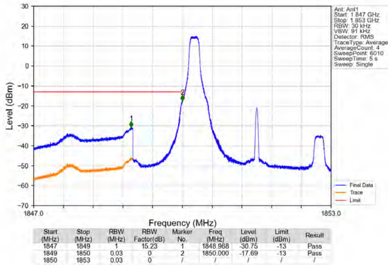
Band2_3MHz_16QAM_LCH_1851.5MHz_RB_1_0_NTNV
