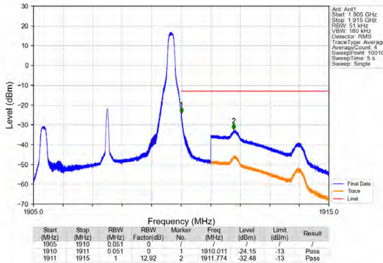
Band2_5MHz_16QAM_HCH_1907.5MHz_RB_1_24_NTNV
