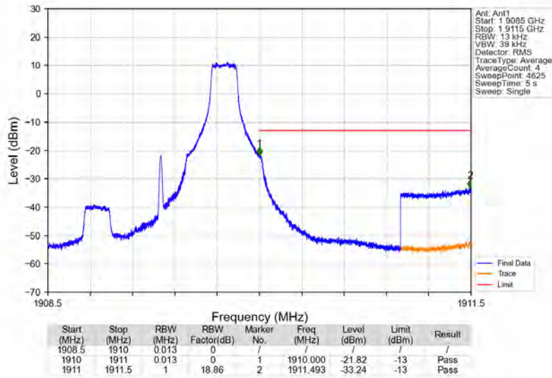
Band2_1.4MHz_16QAM_HCH_1909.3MHz_RB_1_5_NTNV
