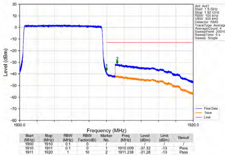
Band2_10MHz_64QAM_HCH_1905MHz_RB_50_0_NTV
