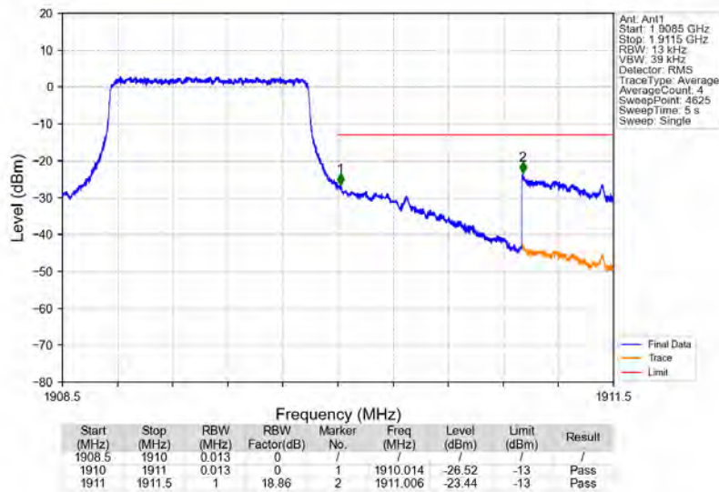
Band2_1.4MHz_16QAM_HCH_1909.3MHz_RB_6_0_NTNV
