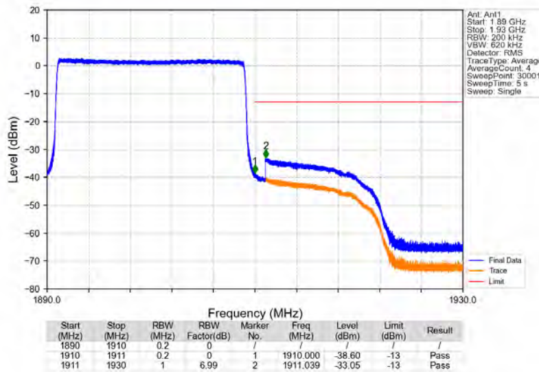
Band2_20MHz_64QAM_HCH_1900MHz_RB_100_0_NTNV
