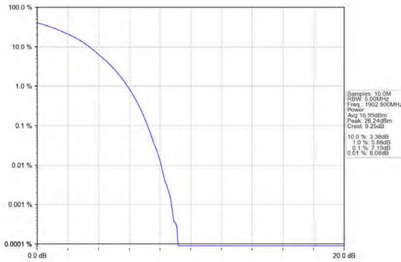
Band2_15MHz_64QAM_HCH_1902.5MHz_RB_75_0_NTNV
