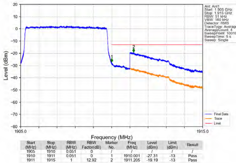
Band2_5MHz_16QAM_HCH_1907.5MHz_RB_25_0_NTNV
