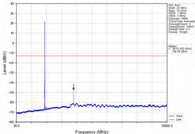
Band2_5MHz_QPSK_HCH_1907.5MHz_RB_1_0_NTNV
