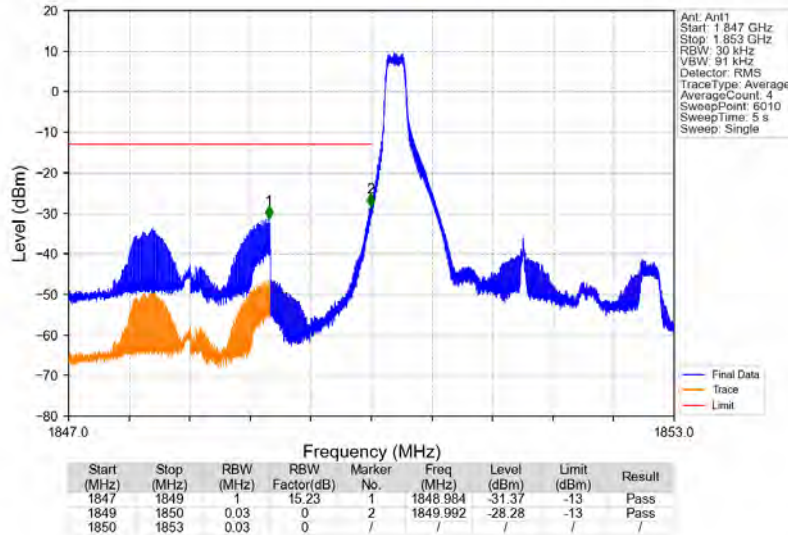
Band2_3MHz_64QAM_LCH_1851.5MHz_RB_1_0_NTNV
