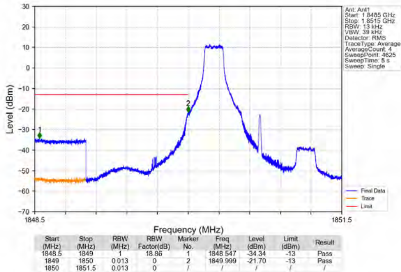
Band2_1.4MHz_16QAM_LCH_1850.7MHz_RB_1_0_NTNV
