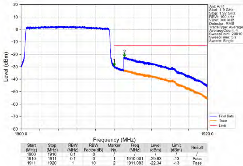
Band2_10MHz_16QAM_HCH_1905MHz_RB_50_0_NTV
