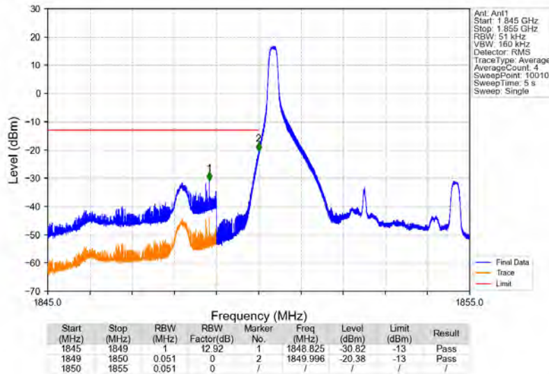
Band2_5MHz_64QAM_LCH_1852.5MHz_RB_1_0_NTNV
