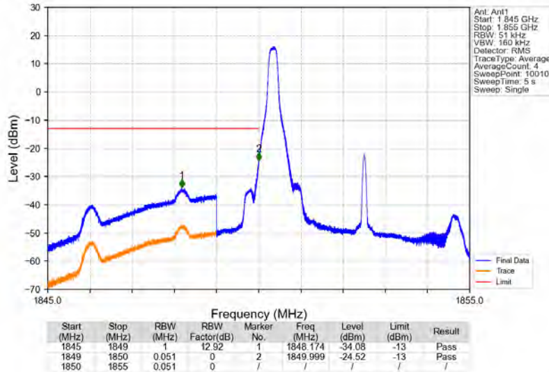
Band2_5MHz_16QAM_LCH_1852.5MHz_RB_1_0_NTNV
