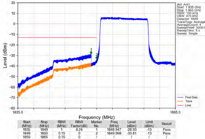
Band2_15MHz_64QAM_LCH_1857.5MHz_RB_1_0_NTNV
