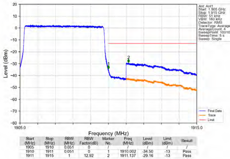
Band2_5MHz_64QAM_HCH_1907.5MHz_RB_25_0_NTNV
