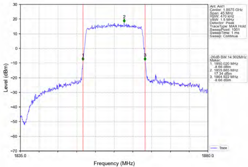
Band2_15MHz_16QAM_LCH_1857.5MHz_RB_75_0_NTNV
