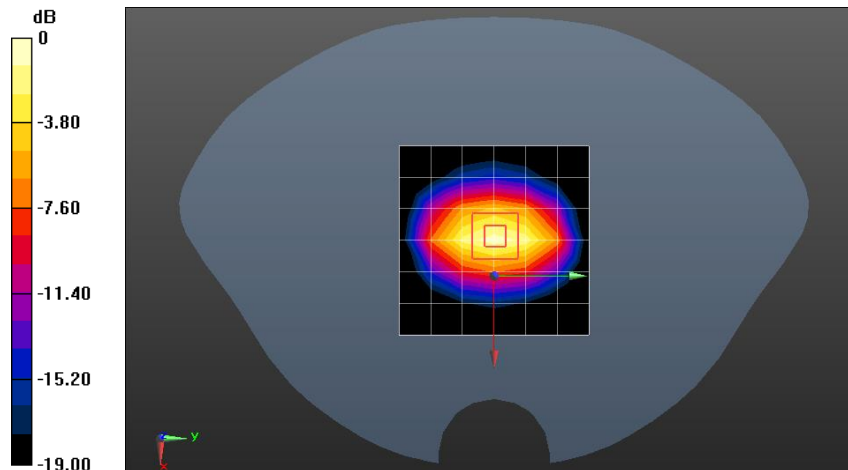
0 dB = 14.5 W/kg = 11.61 dBW/kg
