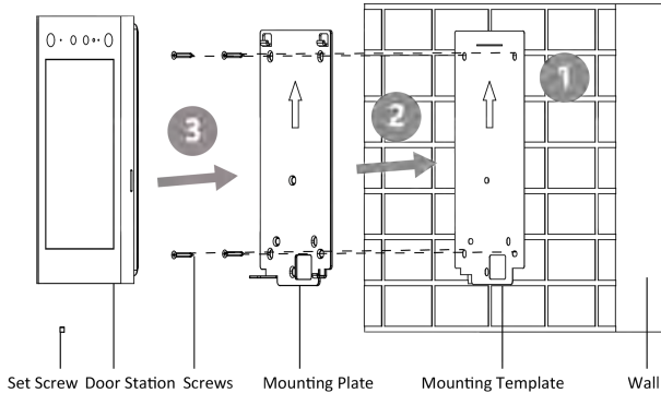
Figure 3-3 Surface Mounting
