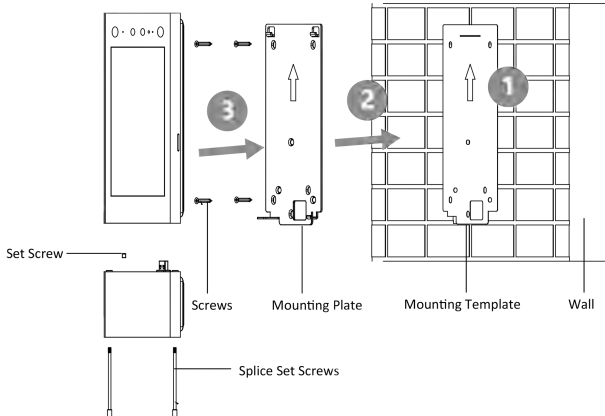
Figure 3-15 Surface Mounting
