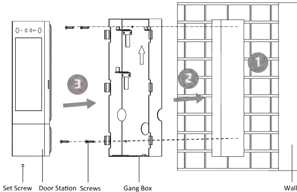
Figure 3-16 Flush Mounting
