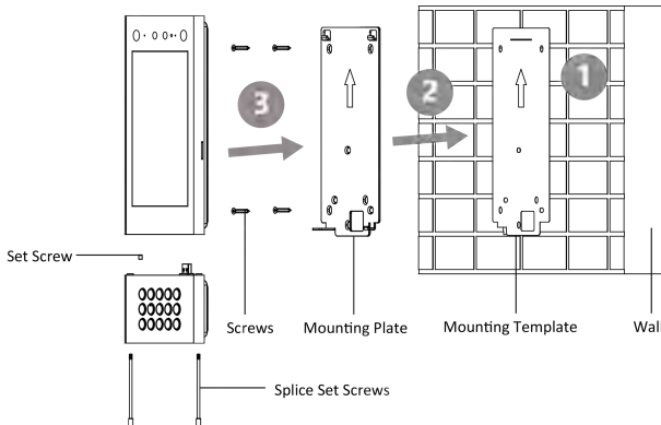
Figure 3-7 Surface Mounting
