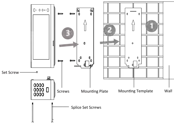
Figure 3-11 Surface Mounting
