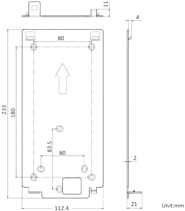
Figure 3-13 Mounting Plate
