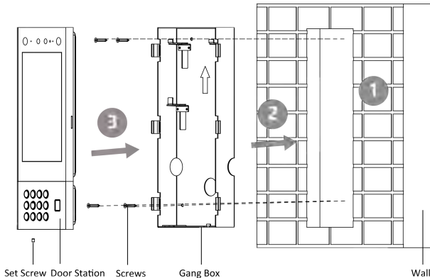
Figure 3-12 Flush Mounting
