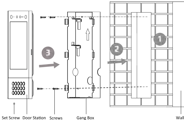
Figure 3-8 Flush Mounting
