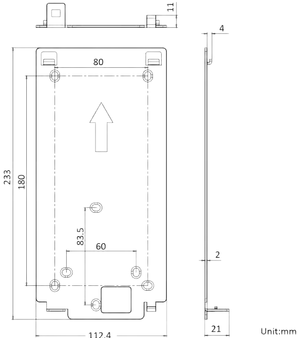
Figure 3-9 Mounting Plate
