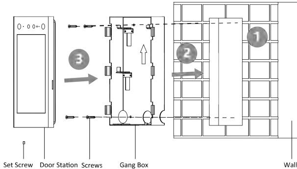
Figure 4-4 Flush Mounting
