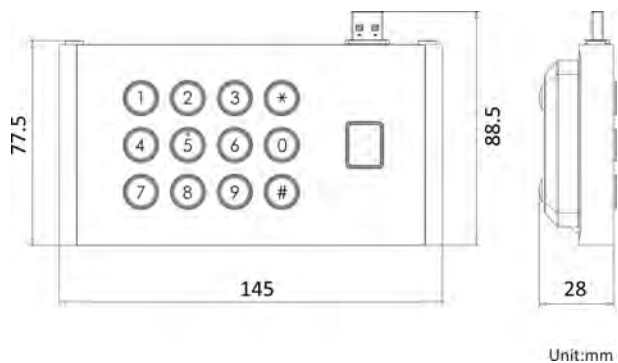
Figure 5-2 Fingerprint Module
