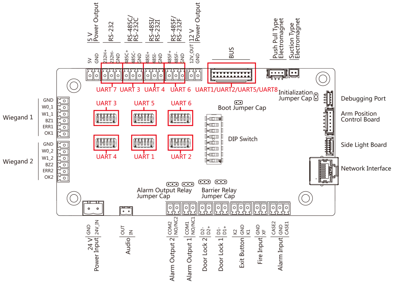
Figure 4-6 UART No. Diagram
