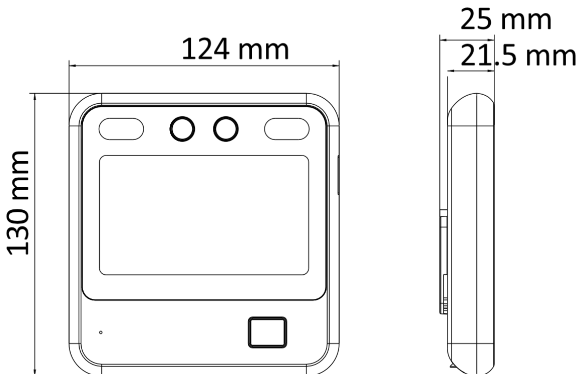
Figure 2-1 Appearance
