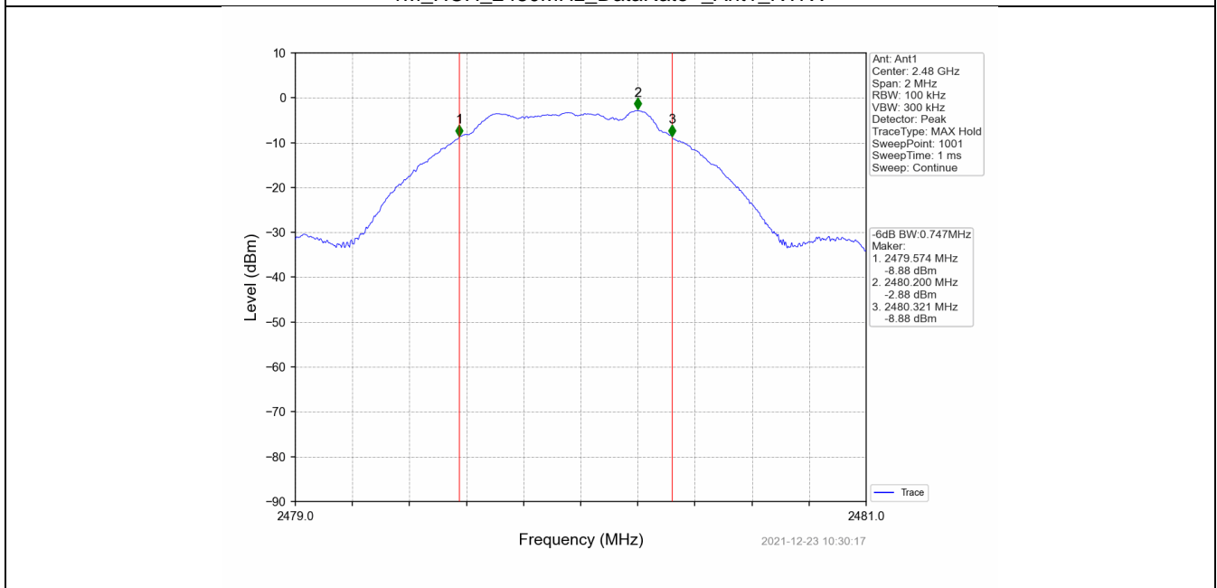
1M_HCH_2480MHz_DataRate=_ Ant1_NTNV
