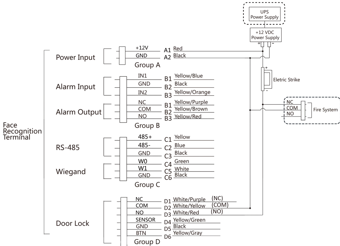
Figure 4-8 Device Wiring
