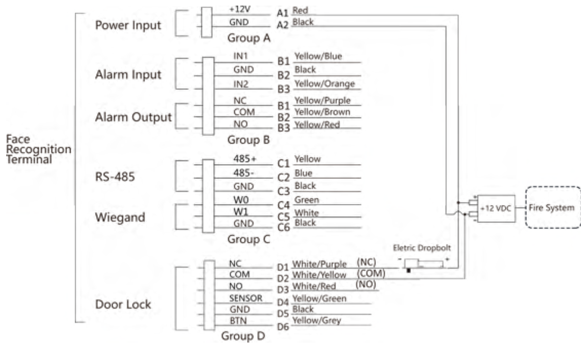
Figure 4-4 Wire Device
