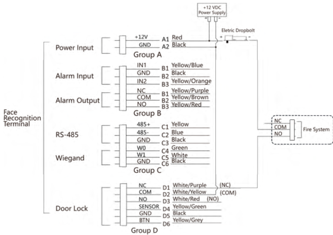
Figure 4-6 Wiring Device
