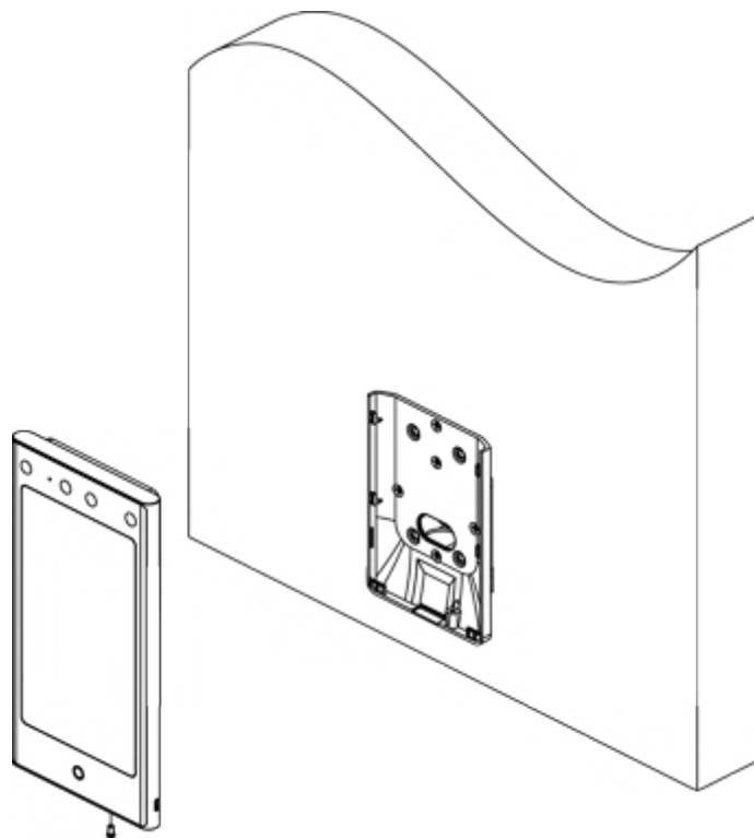
Figure 3-8 Hang Device
