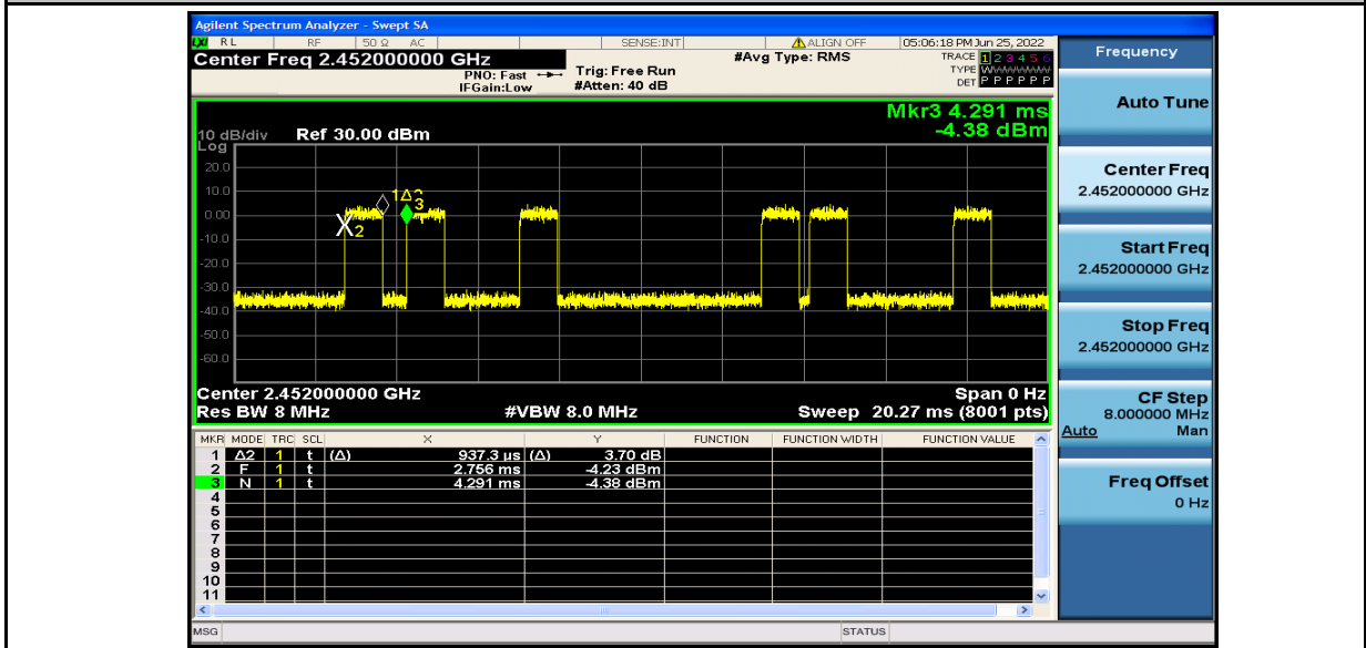
Duty Cycle_11N40SISO_2452_Ant1
